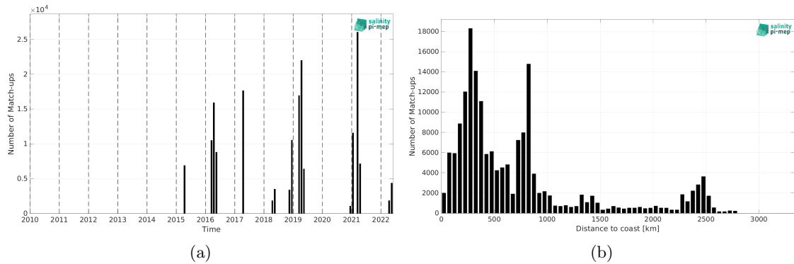
Figure 2: Number of match-ups between TSG (CSIC-UTM) and SMAP SSS L2 v6 - 40 km (RSS) SSS as a function of time (a) and as function of the distance to coast (b) over the South Atlantic Ocean Pi-MEP region and for the full satellite product period.
