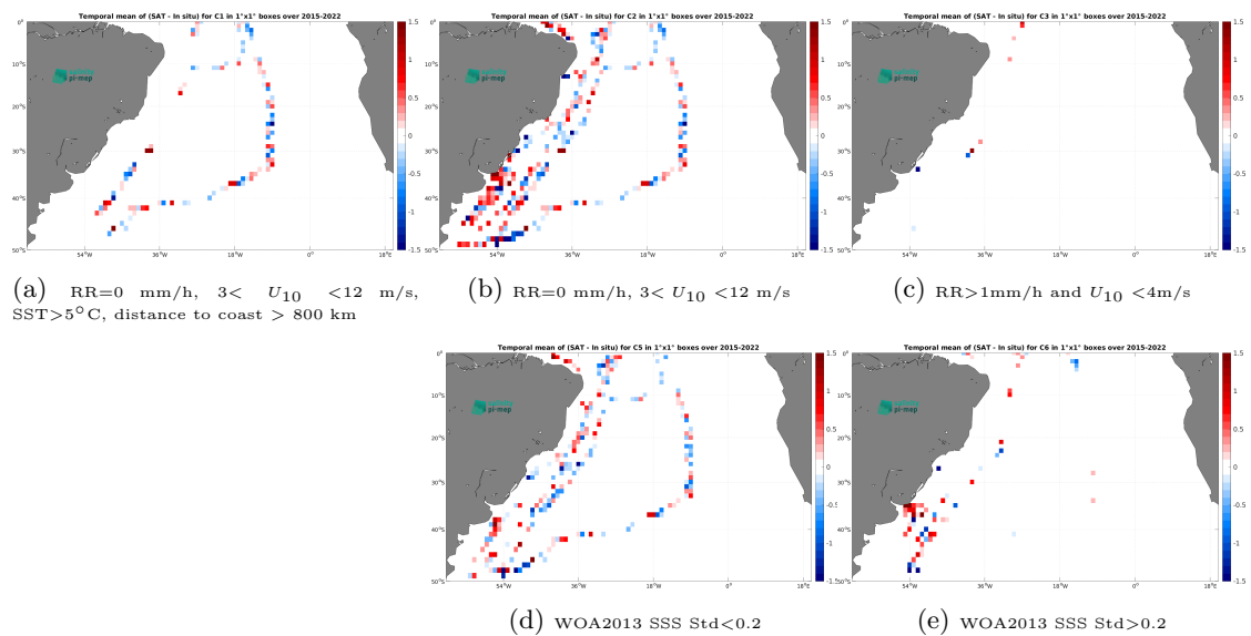
Figure 14: Temporal mean gridded over spatial boxes of size 1^\circ \times 1^\circ of \Delta\text{SSS} (SMAP SSS L2 v6 - 40 km (RSS) - TSG (CSIC-UTM)) for 5 different subdatasets corresponding to:RR=0 mm/h, 3 < U_{10} < 12 m/s, SST>5°C, distance to coast > 800 km (a), RR=0 mm/h, 3 < U_{10} < 12 m/s (b), RR>1mm/h and U_{10} < 4 m/s (c), WOA2013 SSS Std<0.2 (d), WOA2013 SSS Std>0.2 (e).
