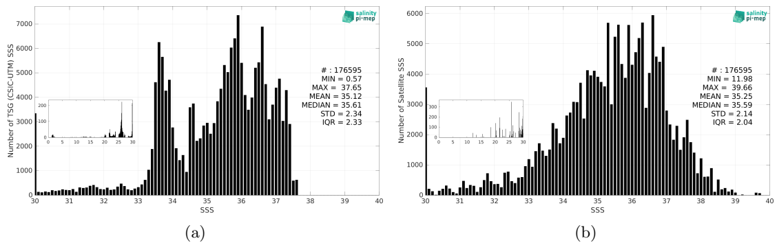
Figure 3: Histograms of SSS from TSG (CSIC-UTM) (a) and SMAP SSS L2 v6 - 40 km (RSS) (b) considering all match-up pairs per bins of 0.1 over the South Atlantic Ocean Pi-MEP region and for the full satellite product period.
