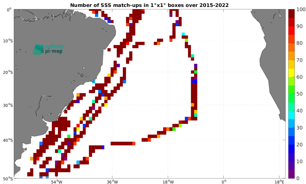
Figure 5: Number of SSS match-ups between TSG (CSIC-UTM) SSS and the SMAP SSS L2 v6 - 40 km (RSS) SSS product for the South Atlantic Ocean Pi-MEP region over 1^\circ \times 1^\circ boxes and for the full satellite product period.
