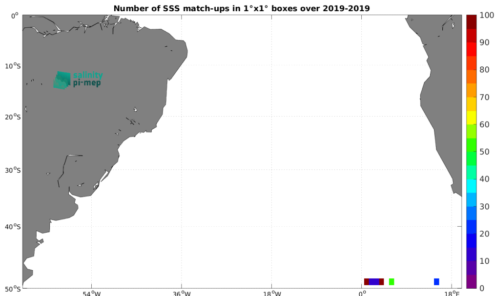
Figure 5: Number of SSS match-ups between Saildrone SSS and the SMAP SSS L2 v6 - 40 km (RSS) SSS product for the South Atlantic Ocean Pi-MEP region over 1^\circ \times 1^\circ boxes and for the full satellite product period.
