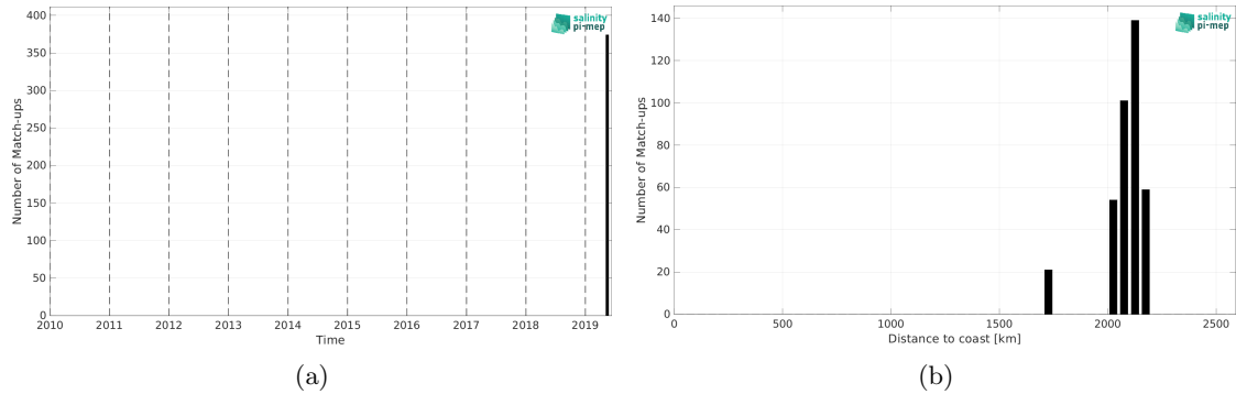
Figure 2: Number of match-ups between Saildrone and SMAP SSS L2 v6 - 40 km (RSS) SSS as a function of time (a) and as function of the distance to coast (b) over the South Atlantic Ocean Pi-MEP region and for the full satellite product period.
