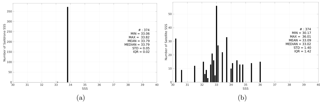
Figure 3: Histograms of SSS from Saildrone (a) and SMAP SSS L2 v6 - 40 km (RSS) (b) considering all match-up pairs per bins of 0.1 over the South Atlantic Ocean Pi-MEP region and for the full satellite product period.
