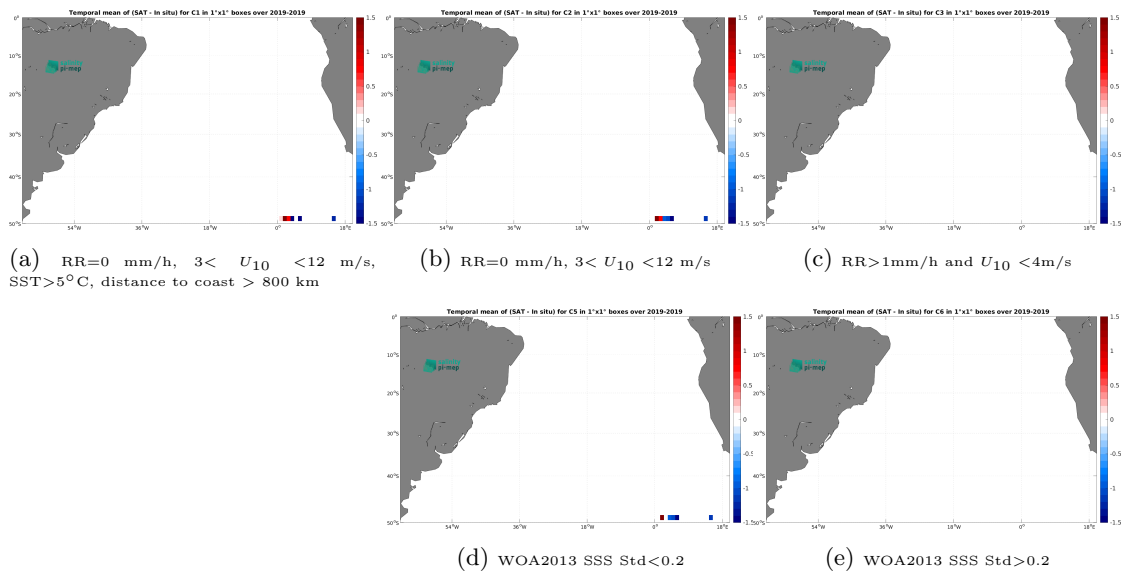
Figure 14: Temporal mean gridded over spatial boxes of size 1^\circ \times 1^\circ of \Delta SSS (SMAP SSS L2 v6 - 40 km (RSS) - Saldron) for 5 different subdatasets corresponding to:RR=0 mm/h, 3 < U_{10} < 12 m/s, SST>5°C, distance to coast > 800 km (a), RR=0 mm/h, 3 < U_{10} < 12 m/s (b), RR>1mm/h and U_{10} < 4 m/s (c), WOA2013 SSS Std<0.2 (d), WOA2013 SSS Std>0.2 (e).
