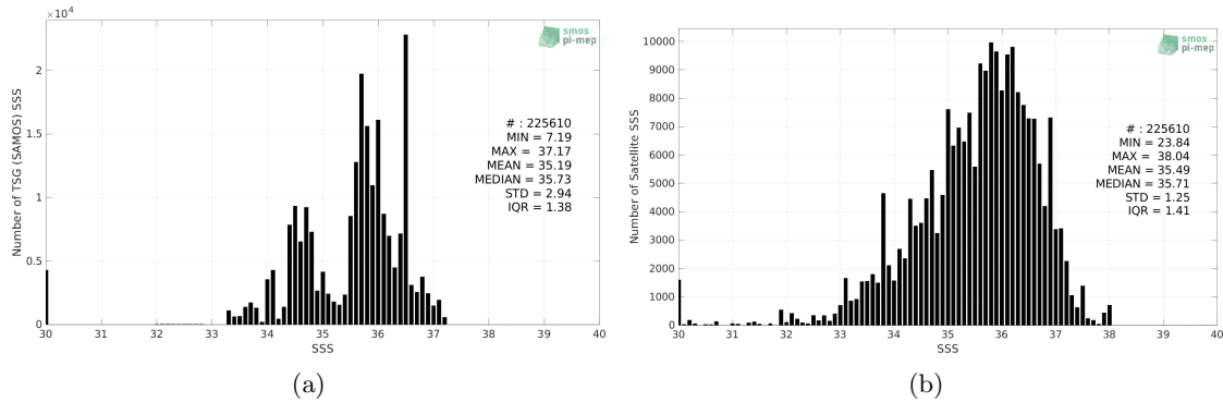
Figure 2: Histograms of SSS from TSG (SAMOS) (a) and SMAP SSS L2 v5 (RSS) (b) considering all match-up pairs per bins of 0.1 over the South Atlantic Ocean Pi-MEP region and for the full satellite product period.
