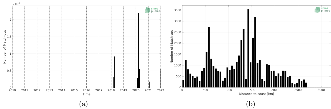
Figure 1: Number of match-ups between TSG (SAMOS) and SMAP SSS L2 v5 (RSS) SSS as a function of time (a) and as function of the distance to coast (b) over the South Atlantic Ocean Pi-MEP region and for the full satellite product period.
