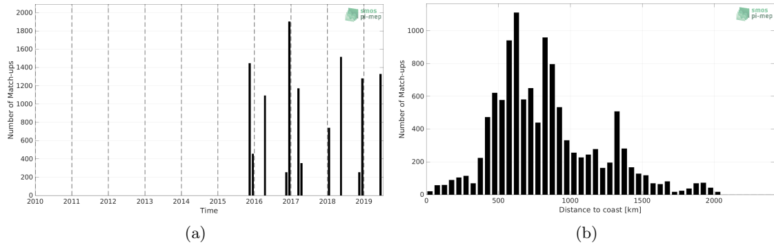
Figure 1: Number of match-ups between TSG (Polarstern) and SMAP SSS L2 v5 (RSS) SSS as a function of time (a) and as function of the distance to coast (b) over the South Atlantic Ocean Pi-MEP region and for the full satellite product period.
