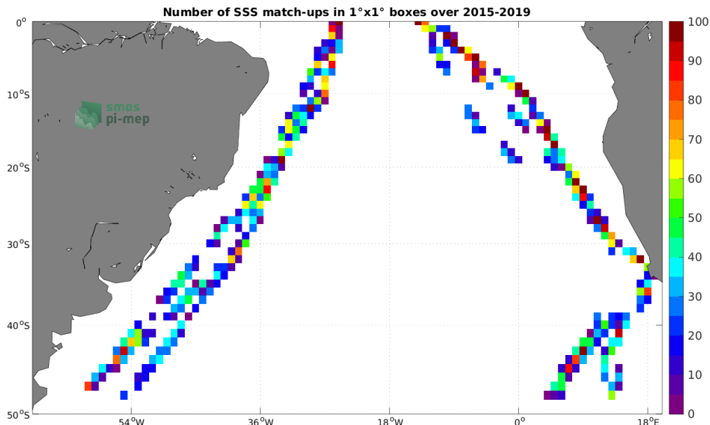
Figure 4: Number of SSS match-ups between TSG (Polarstern) SSS and the SMAP SSS L2 v5 (RSS) SSS product for the South Atlantic Ocean Pi-MEP region over 1^\circ \times 1^\circ boxes and for the full satellite product period.
