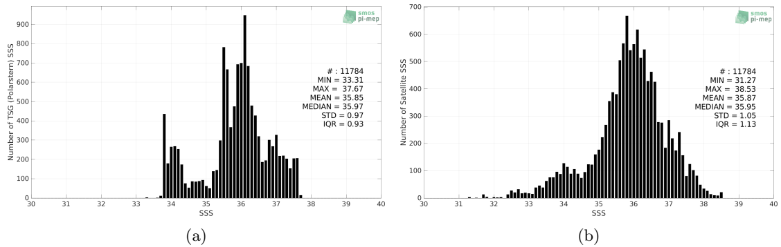
Figure 2: Histograms of SSS from TSG (Polarstern) (a) and SMAP SSS L2 v5 (RSS) (b) considering all match-up pairs per bins of 0.1 over the South Atlantic Ocean Pi-MEP region and for the full satellite product period.
