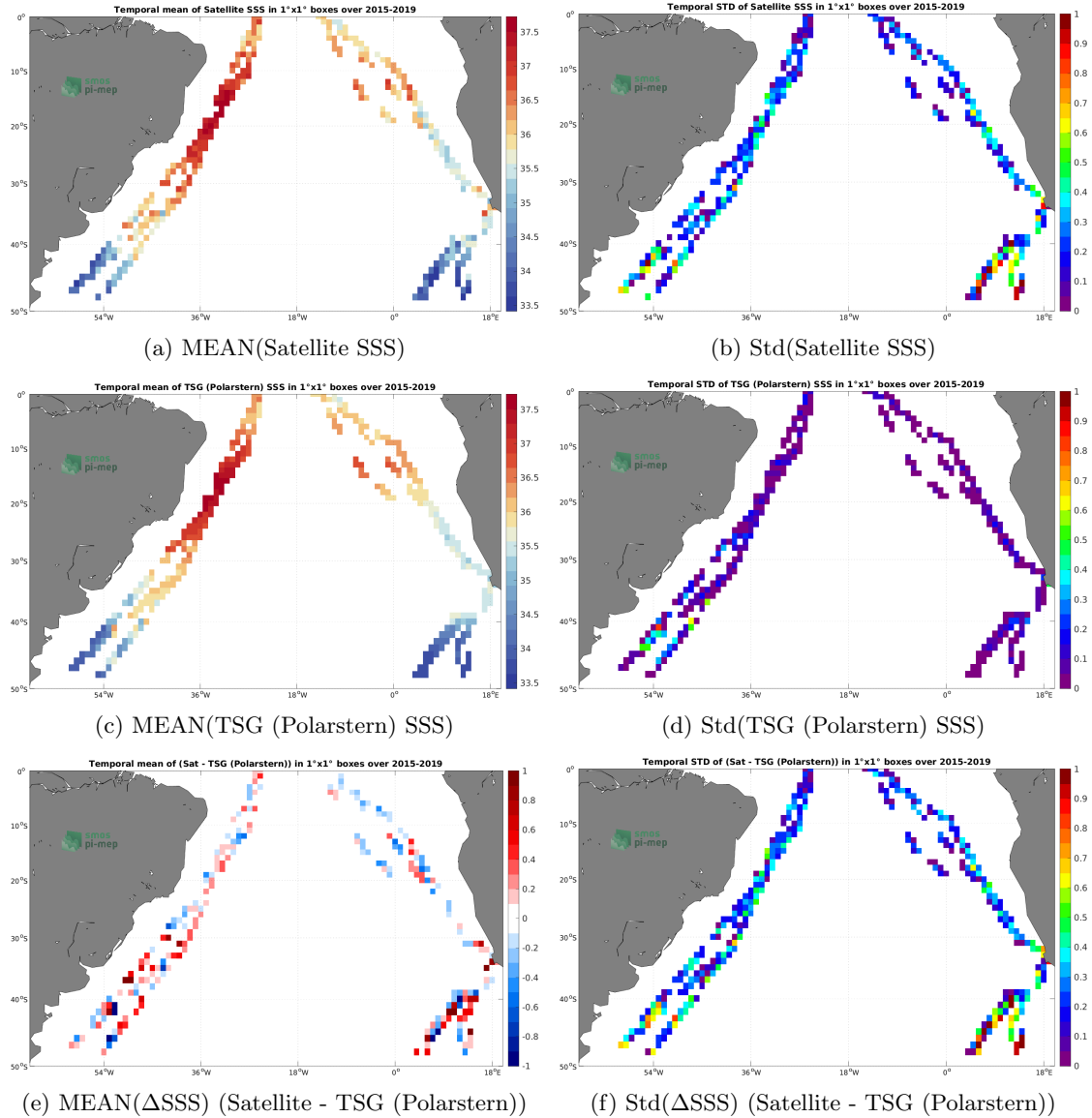
Figure 6: Temporal mean (left) and Std (right) of SSS from SMAP SSS L2 v5 (RSS) (top), TSG (Polarstern) (middle), and of \Delta SSS (Satellite - TSG (Polarstern)). Only match-up pairs are used to generate these maps.
