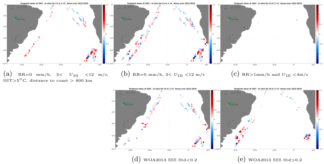
Figure 12: Temporal mean gridded over spatial boxes of size 1^\circ \times 1^\circ of \Delta SSS (SMAP SSS L2 v5 (RSS) - TSG (Polarstern)) for 5 different subdatasets corresponding to:RR=0 mm/h, 3 < U_{10} < 12 m/s, SST >5^\circ\text{C} , distance to coast > 800 km (a), RR=0 mm/h, 3 < U_{10} < 12 m/s (b), RR >1 mm/h and U_{10} < 4 m/s (c), WOA2013 SSS Std <0.2 (d), WOA2013 SSS Std >0.2 (e).
