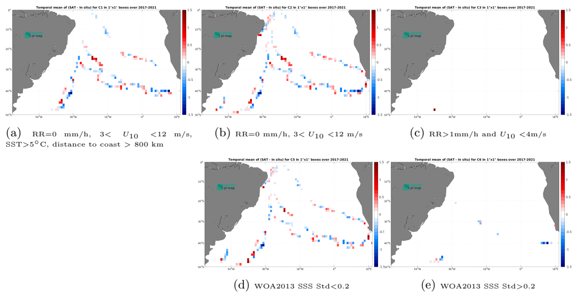
Figure 12: Temporal mean gridded over spatial boxes of size 1^\circ \times 1^\circ of \Delta\text{SSS} (SMAP SSS L2 v5 (RSS) - TSG (GOSUD-Sailing-ship)) for 5 different subdatasets corresponding to:RR=0 mm/h, 3 < U_{10} < 12 m/s, SST >5^\circ\text{C} , distance to coast > 800 km (a), RR=0 mm/h, 3 < U_{10} < 12 m/s (b), RR >1 mm/h and U_{10} < 4 m/s (c), WOA2013 SSS Std <0.2 (d), WOA2013 SSS Std >0.2 (e).
