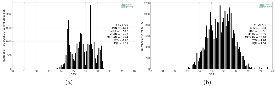
Figure 2: Histograms of SSS from TSG (GOSUD-Sailing-ship) (a) and SMAP SSS L2 v5 (RSS) (b) considering all match-up pairs per bins of 0.1 over the South Atlantic Ocean Pi-MEP region and for the full satellite product period.
