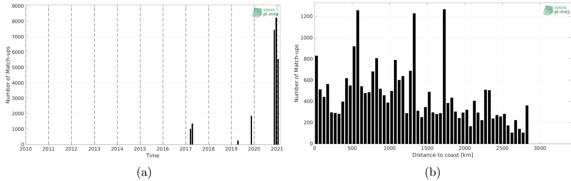
Figure 1: Number of match-ups between TSG (GOSUD-Sailing-ship) and SMAP SSS L2 v5 (RSS) SSS as a function of time (a) and as function of the distance to coast (b) over the South Atlantic Ocean Pi-MEP region and for the full satellite product period.
