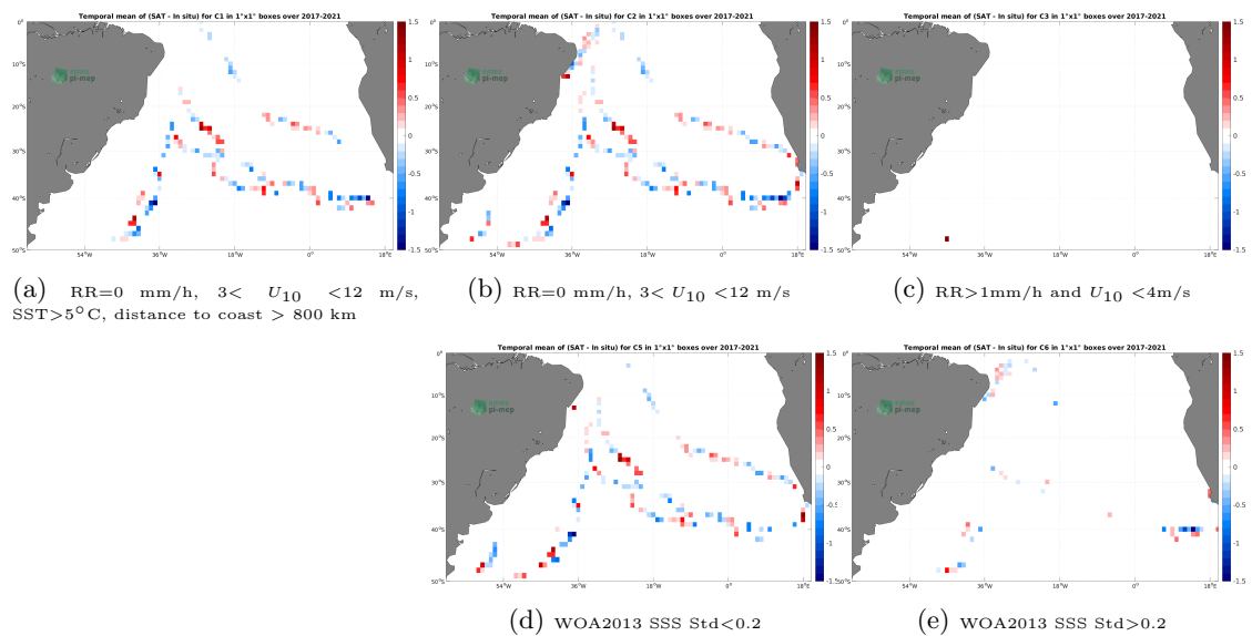
Figure 12: Temporal mean gridded over spatial boxes of size 1^\circ \times 1^\circ of \Delta SSS (SMAP SSS L2 v5 (RSS) - TSG (GOSUD-Sailing-ship)) for 5 different subdatasets corresponding to:RR=0 mm/h, 3 < U_{10} < 12 m/s, SST>5°C, distance to coast > 800 km (a), RR=0 mm/h, 3 < U_{10} < 12 m/s (b), RR>1mm/h and U_{10} < 4 m/s (c), WOA2013 SSS Std<0.2 (d), WOA2013 SSS Std>0.2 (e).
