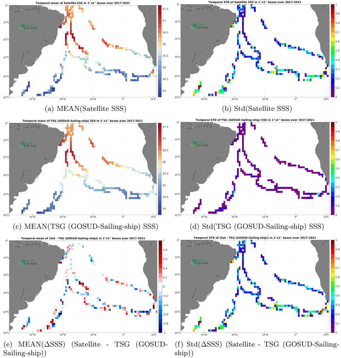
Figure 6: Temporal mean (left) and Std (right) of SSS from SMAP SSS L2 v5 (RSS) (top), TSG (GOSUD-Sailing-ship) (middle), and of \Delta SSS (Satellite - TSG (GOSUD-Sailing-ship)). Only match-up pairs are used to generate these maps.
