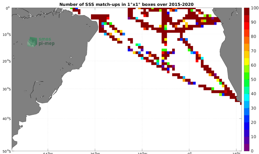
Figure 4: Number of SSS match-ups between TSG (GOSUD-Research-vessel) SSS and the SMAP SSS L2 v5 (RSS) SSS product for the South Atlantic Ocean Pi-MEP region over 1°x1° boxes and for the full satellite product period.
