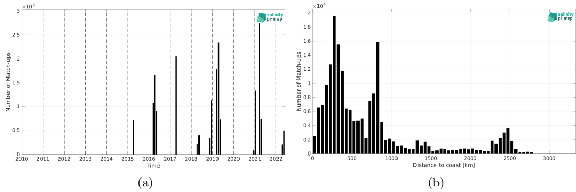
Figure 1: Number of match-ups between TSG (CSIC-UTM) and SMAP SSS L2 v5 (RSS) SSS as a function of time (a) and as function of the distance to coast (b) over the South Atlantic Ocean Pi-MEP region and for the full satellite product period.
