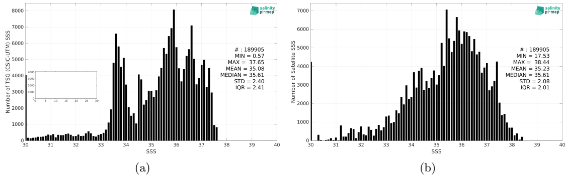
Figure 2: Histograms of SSS from TSG (CSIC-UTM) (a) and SMAP SSS L2 v5 (RSS) (b) considering all match-up pairs per bins of 0.1 over the South Atlantic Ocean Pi-MEP region and for the full satellite product period.
