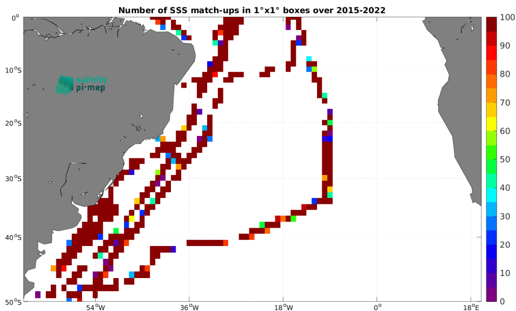
Figure 4: Number of SSS match-ups between TSG (CSIC-UTM) SSS and the SMAP SSS L2 v5 (RSS) SSS product for the South Atlantic Ocean Pi-MEP region over 1^\circ \times 1^\circ boxes and for the full satellite product period.
