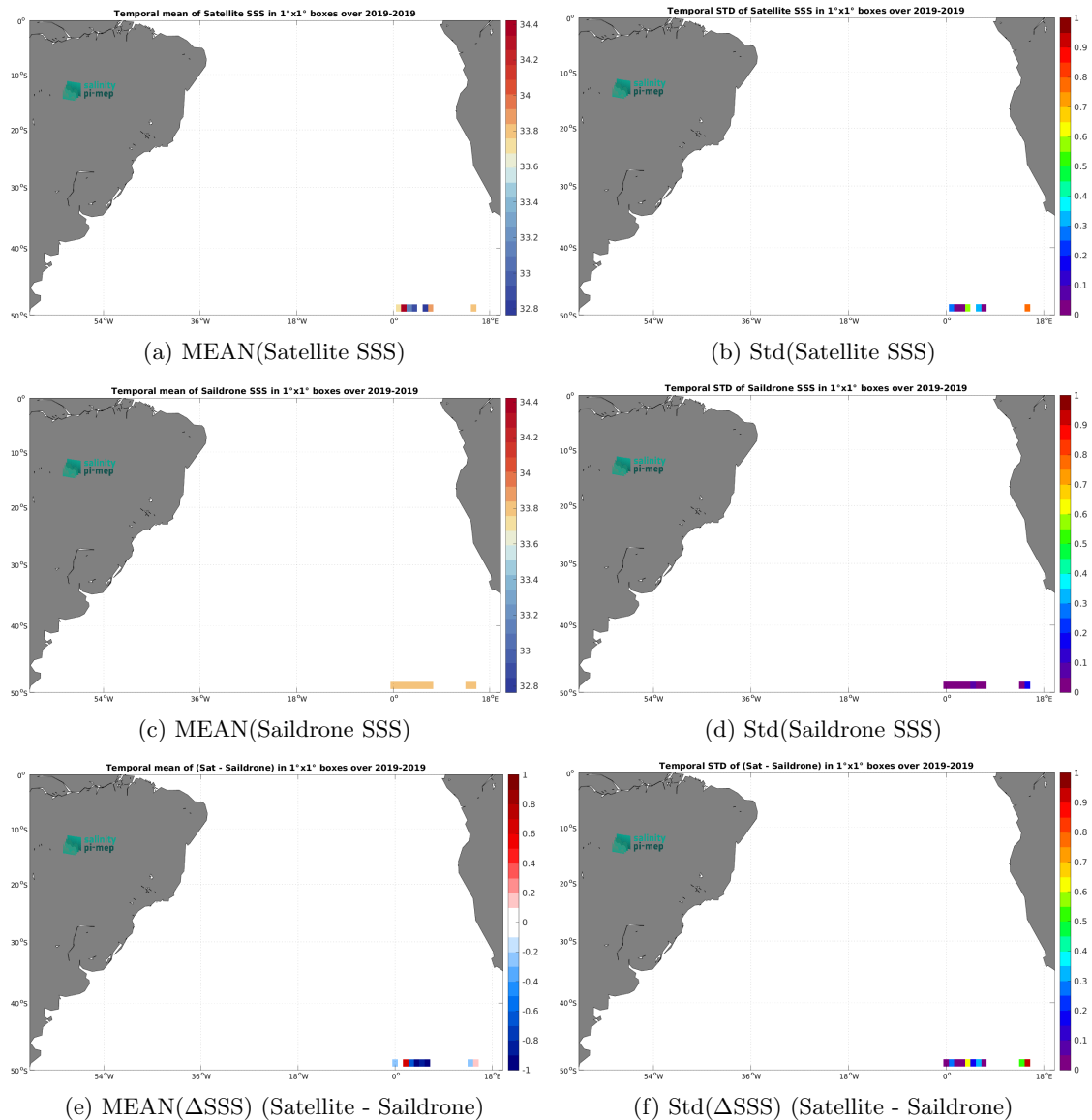
Figure 6: Temporal mean (left) and Std (right) of SSS from SMAP SSS L2 v5 (RSS) (top), Saildrone (middle), and of \Delta SSS (Satellite - Saildrone). Only match-up pairs are used to generate these maps.
