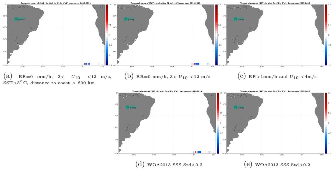
Figure 12: Temporal mean gridded over spatial boxes of size 1^{\circ}\times 1^{\circ} of \Delta\text{SSS} (SMAP SSS L2 v5 (RSS) - Saikrone) for 5 different subdatasets corresponding to:RR=0 mm/h, 3 < U_{10} < 12 m/s, SST >5^{\circ}\text{C} , distance to coast > 800 km (a), RR=0 mm/h, 3 < U_{10} < 12 m/s (b), RR >1 mm/h and U_{10} < 4 m/s (c), WOA2013 SSS Std <0.2 (d), WOA2013 SSS Std >0.2 (e).
