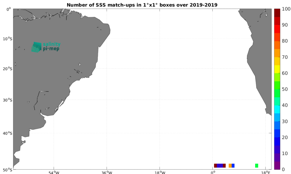
Figure 4: Number of SSS match-ups between Saildrone SSS and the SMAP SSS L2 v5 (RSS) SSS product for the South Atlantic Ocean Pi-MEP region over 1^\circ \times 1^\circ boxes and for the full satellite product period.
