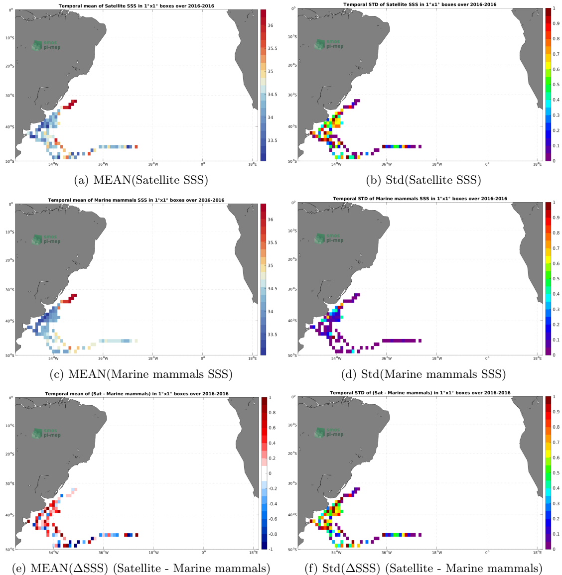
Figure 6: Temporal mean (left) and Std (right) of SSS from SMAP SSS L2 v5 (RSS) (top), Marine mammals (middle), and of \Delta SSS (Satellite - Marine mammals). Only match-up pairs are used to generate these maps.
