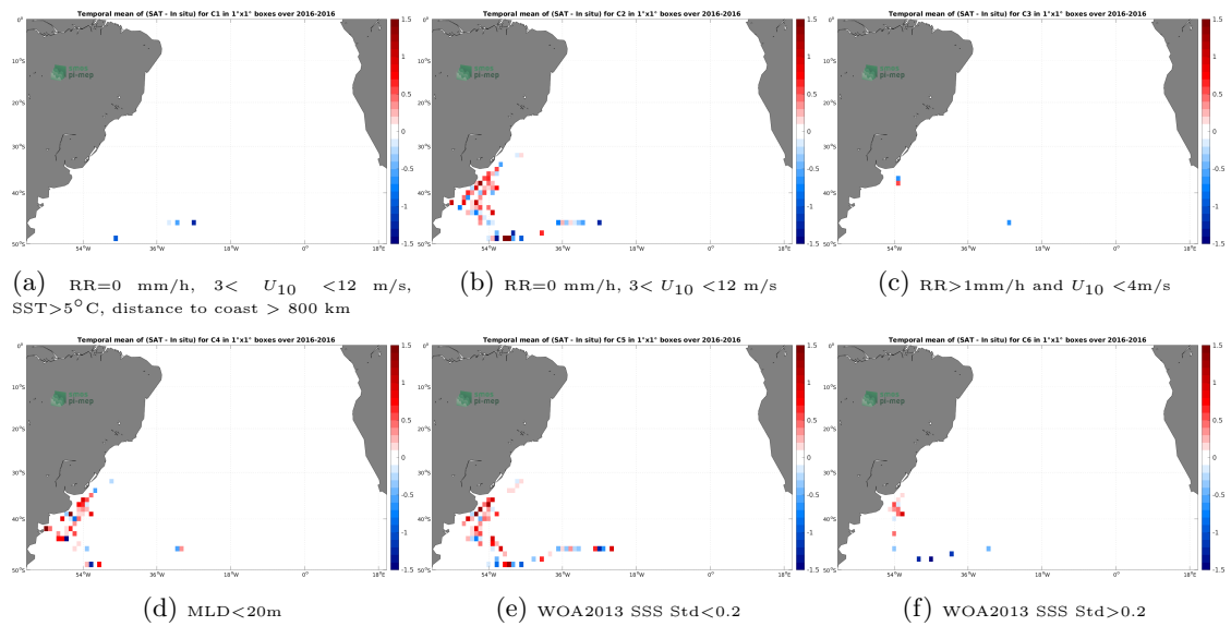
Figure 12: Temporal mean gridded over spatial boxes of size 1^\circ \times 1^\circ of \Delta SSS (SMAP SSS L2 v5 (RSS) - Marine mammals) for 6 different subdatasets corresponding to:RR=0 mm/h, 3 < U_{10} < 12 m/s, SST >5^\circ\text{C} , distance to coast > 800 km (a), RR=0 mm/h, 3 < U_{10} < 12 m/s (b), RR >1 mm/h and U_{10} < 4 m/s (c),MLD <20 m (d),WOA2013 SSS Std <0.2 (e),WOA2013 SSS Std >0.2 (f).
