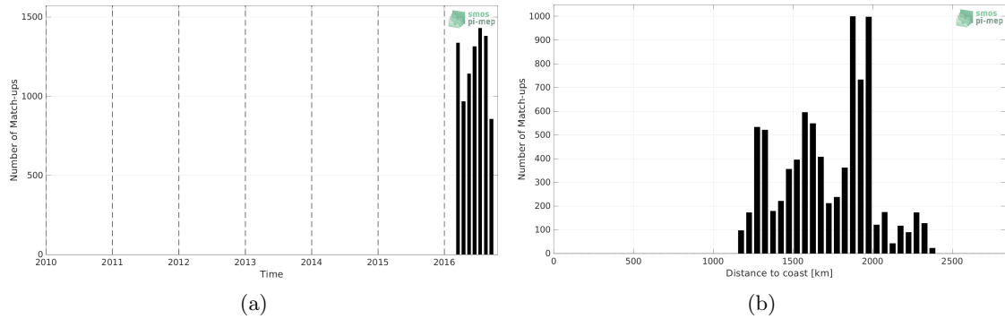
Figure 1: Number of match-ups between Surface drifters and SMAP SSS L2 v5 (RSS) SSS as a function of time (a) and as function of the distance to the coast (b) over the South Atlantic Ocean Pi-MEP region and for the full satellite product period.
