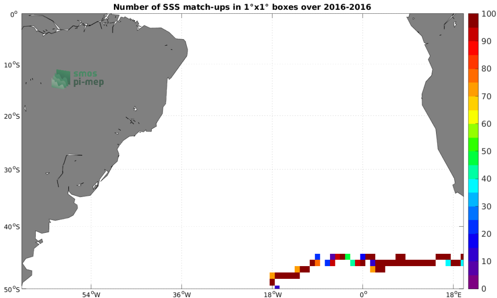
Figure 3: Number of SSS match-ups between Surface drifters SSS and the SMAP SSS L2 v5 (RSS) SSS product for the South Atlantic Ocean Pi-MEP region over 1^\circ \times 1^\circ boxes and for the full satellite product period.
