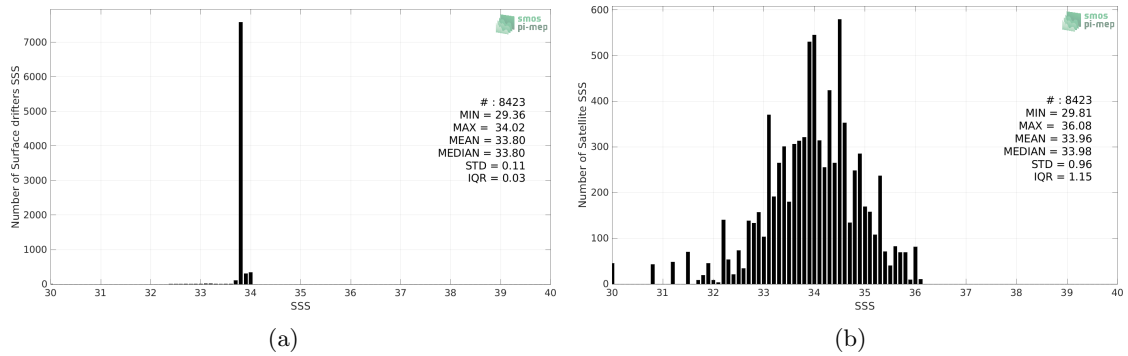
Figure 2: Histograms of SSS from Surface drifters (a) and SMAP SSS L2 v5 (RSS) (b) considering all match-up pairs per bins of 0.1 over the South Atlantic Ocean Pi-MEP region and for the full satellite product period.
