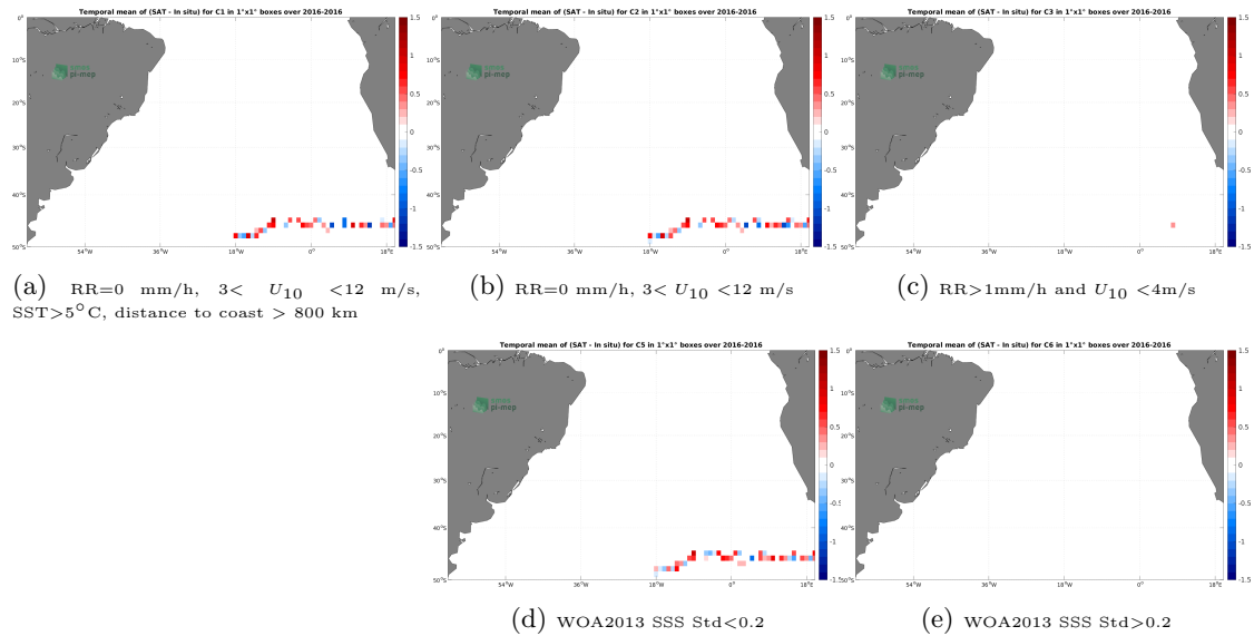
Figure 11: Temporal mean gridded over spatial boxes of size 1^{\circ}\times 1^{\circ} of \Delta\text{SSS} (SMAP SSS L2 v5 (RSS) - Surface drifters) for 5 different subdatasets corresponding to: \text{RR}=0 mm/h, 3 < U_{10} < 12 m/s, \text{SST} > 5^{\circ}\text{C} , distance to coast > 800 km (a), \text{RR}=0 mm/h, 3 < U_{10} < 12 m/s (b), \text{RR} > 1\text{mm/h} and U_{10} < 4\text{m/s} (c), WOA2013 SSS Std < 0.2 (d), WOA2013 SSS Std > 0.2 (e).
