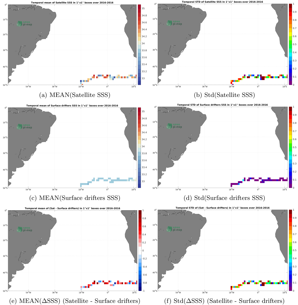
Figure 5: Temporal mean (left) and Std (right) of SSS from SMAP SSS L2 v5 (RSS) (top), Surface drifters (middle), and of \Delta SSS (Satellite - Surface drifters). Only match-up pairs are used to generate these maps.
