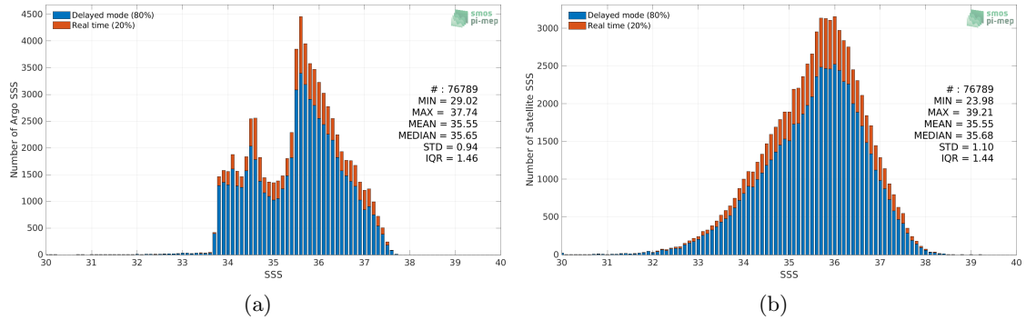
Figure 2: Histograms of SSS from Argo (a) and SMAP SSS L2 v5 (RSS) (b) considering all match-up pairs per bins of 0.1 over the South Atlantic Ocean Pi-MEP region and for the full satellite product period.
