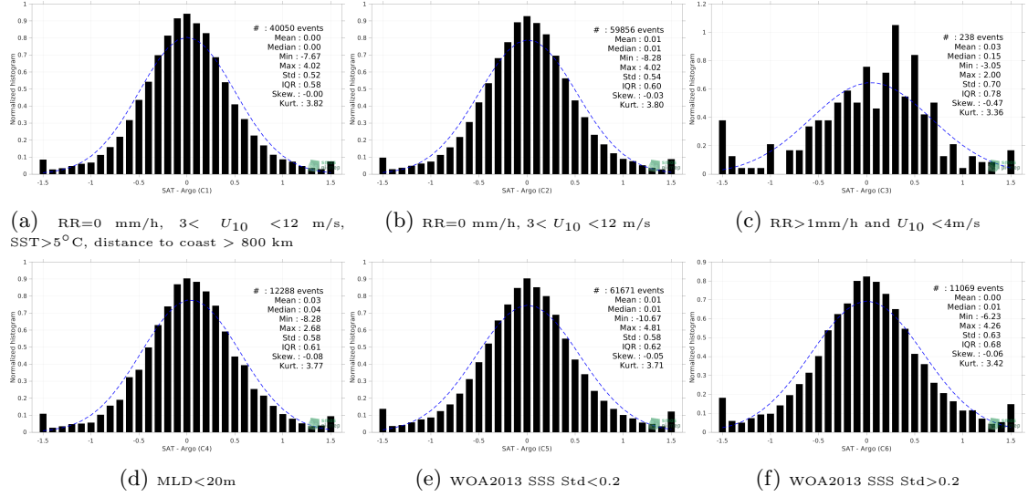
Figure 13: Normalized histogram of \Delta\text{SSS} (SMAP SSS L2 v5 (RSS) - Argo) for 6 different subdatasets corresponding to: RR=0 mm/h, 3 < U_{10} < 12 m/s, SST>5°C, distance to coast > 800 km (a), RR=0 mm/h, 3 < U_{10} < 12 m/s (b), RR>1mm/h and U_{10} < 4 m/s (c), MLD<20m (d), WOA2013 SSS Std<0.2 (e), WOA2013 SSS Std>0.2 (f).
