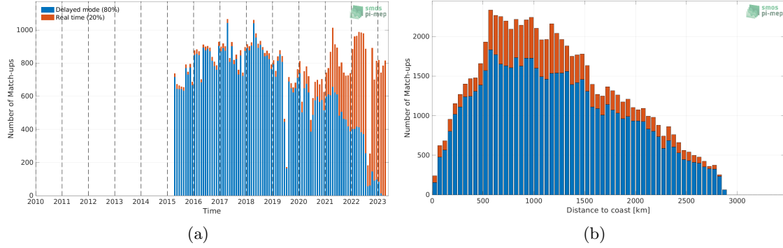
Figure 1: Number of match-ups between Argo and SMAP SSS L2 v5 (RSS) SSS as a function of time (a) and as function of the distance to coast (b) over the South Atlantic Ocean Pi-MEP region and for the full satellite product period.
