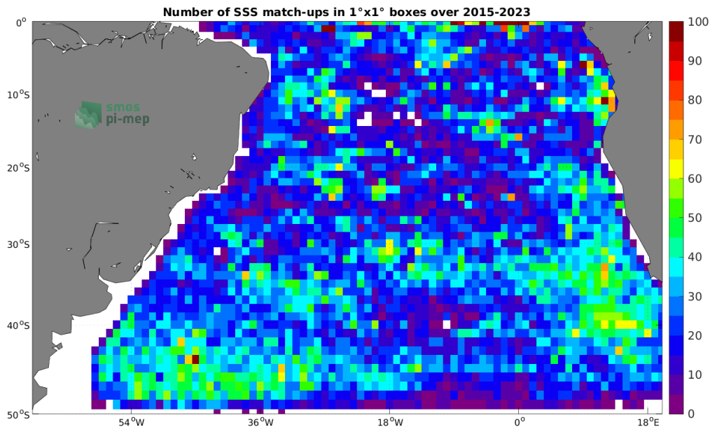
Figure 4: Number of SSS match-ups between Argo SSS and the SMAP SSS L2 v5 (RSS) SSS product for the South Atlantic Ocean Pi-MEP region over 1^\circ \times 1^\circ boxes and for the full satellite product period.
