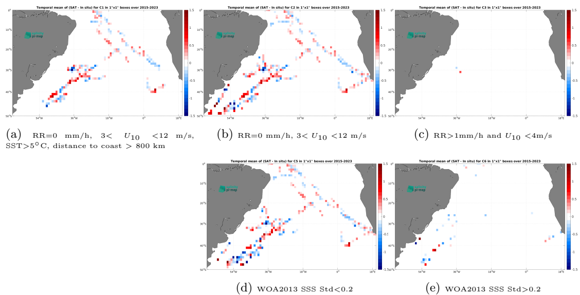
Figure 14: Temporal mean gridded over spatial boxes of size 1^\circ \times 1^\circ of \Delta SSS (SMAP SSS L2 v5.3 (RSS) - TSG (SAMOS)) for 5 different subdatasets corresponding to:RR=0 mm/h, 3 < U_{10} < 12 m/s, SST>5°C, distance to coast > 800 km (a), RR=0 mm/h, 3 < U_{10} < 12 m/s (b), RR>1mm/h and U_{10} < 4 m/s (c), WOA2013 SSS Std<0.2 (d), WOA2013 SSS Std>0.2 (e).
