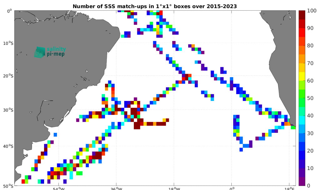
Figure 5: Number of SSS match-ups between TSG (SAMOS) SSS and the SMAP SSS L2 v5.3 (RSS) SSS product for the South Atlantic Ocean Pi-MEP region over 1^\circ \times 1^\circ boxes and for the full satellite product period.
