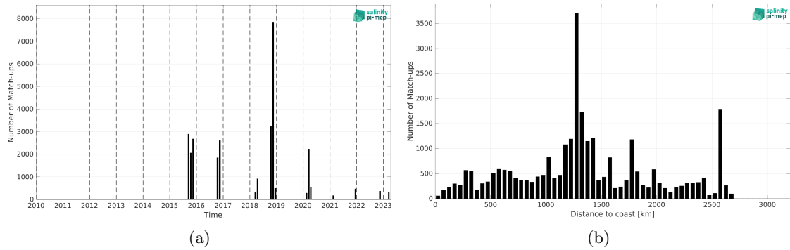
Figure 2: Number of match-ups between TSG (SAMOS) and SMAP SSS L2 v5.3 (RSS) SSS as a function of time (a) and as function of the distance to coast (b) over the South Atlantic Ocean Pi-MEP region and for the full satellite product period.
