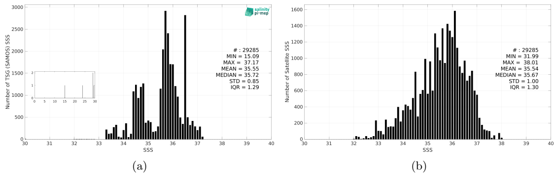
Figure 3: Histograms of SSS from TSG (SAMOS) (a) and SMAP SSS L2 v5.3 (RSS) (b) considering all match-up pairs per bins of 0.1 over the South Atlantic Ocean Pi-MEP region and for the full satellite product period.
