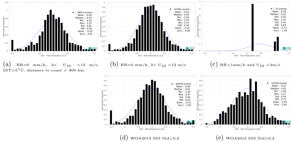
Figure 15: Normalized histogram of \Delta SSS (SMAP SSS L2 v5.3 (RSS) - TSG (Polarstern)) for 5 different subdatasets corresponding to: RR=0 mm/h, 3 < U_{10} < 12 m/s, SST > 5°C, distance to coast > 800 km (a), RR=0 mm/h, 3 < U_{10} < 12 m/s (b), RR > 1 mm/h and U_{10} < 4 m/s (c), WOA2013 SSS Std < 0.2 (d), WOA2013 SSS Std > 0.2 (e).
