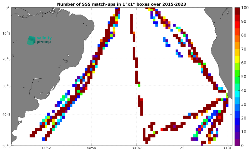
Figure 5: Number of SSS match-ups between TSG (Polarstern) SSS and the SMAP SSS L2 v5.3 (RSS) SSS product for the South Atlantic Ocean Pi-MEP region over 1^\circ \times 1^\circ boxes and for the full satellite product period.
