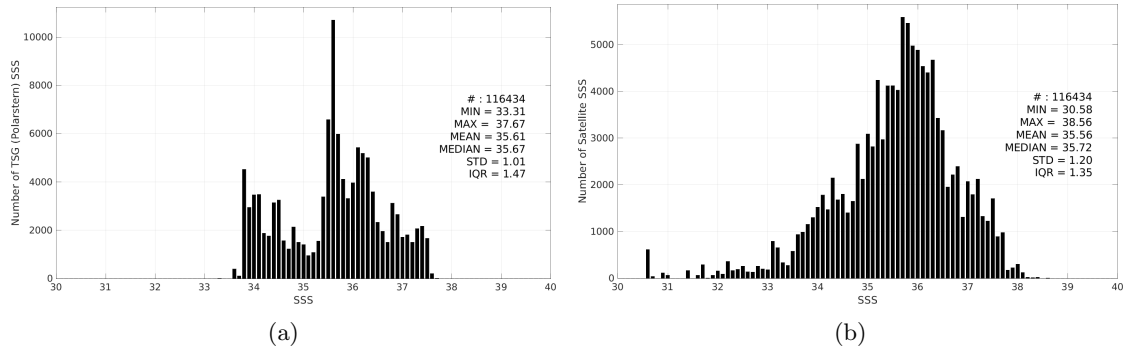
Figure 3: Histograms of SSS from TSG (Polarstern) (a) and SMAP SSS L2 v5.3 (RSS) (b) considering all match-up pairs per bins of 0.1 over the South Atlantic Ocean Pi-MEP region and for the full satellite product period.
