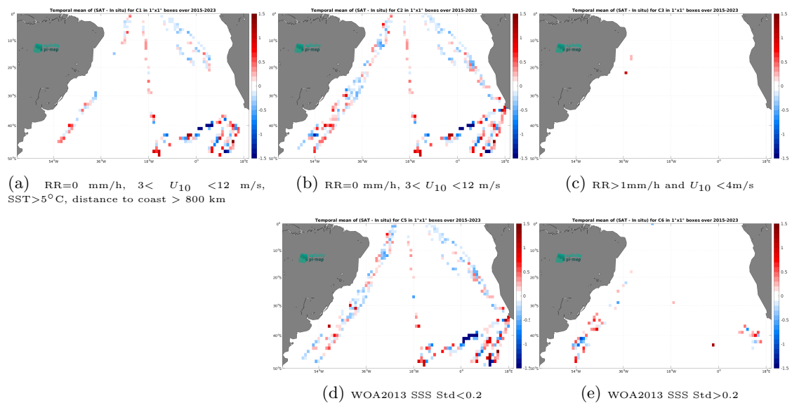
Figure 14: Temporal mean gridded over spatial boxes of size 1^\circ \times 1^\circ of \Delta SSS (SMAP SSS L2 v5.3 (RSS) - TSG (Polarstern)) for 5 different subdatasets corresponding to:RR=0 mm/h, 3 < U_{10} < 12 m/s, SST>5°C, distance to coast > 800 km (a), RR=0 mm/h, 3 < U_{10} < 12 m/s (b), RR>1mm/h and U_{10} < 4 m/s (c), WOA2013 SSS Std<0.2 (d), WOA2013 SSS Std>0.2 (e).
