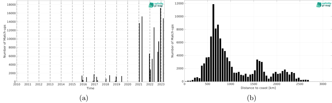
Figure 2: Number of match-ups between TSG (Polarstern) and SMAP SSS L2 v5.3 (RSS) SSS as a function of time (a) and as function of the distance to coast (b) over the South Atlantic Ocean Pi-MEP region and for the full satellite product period.
