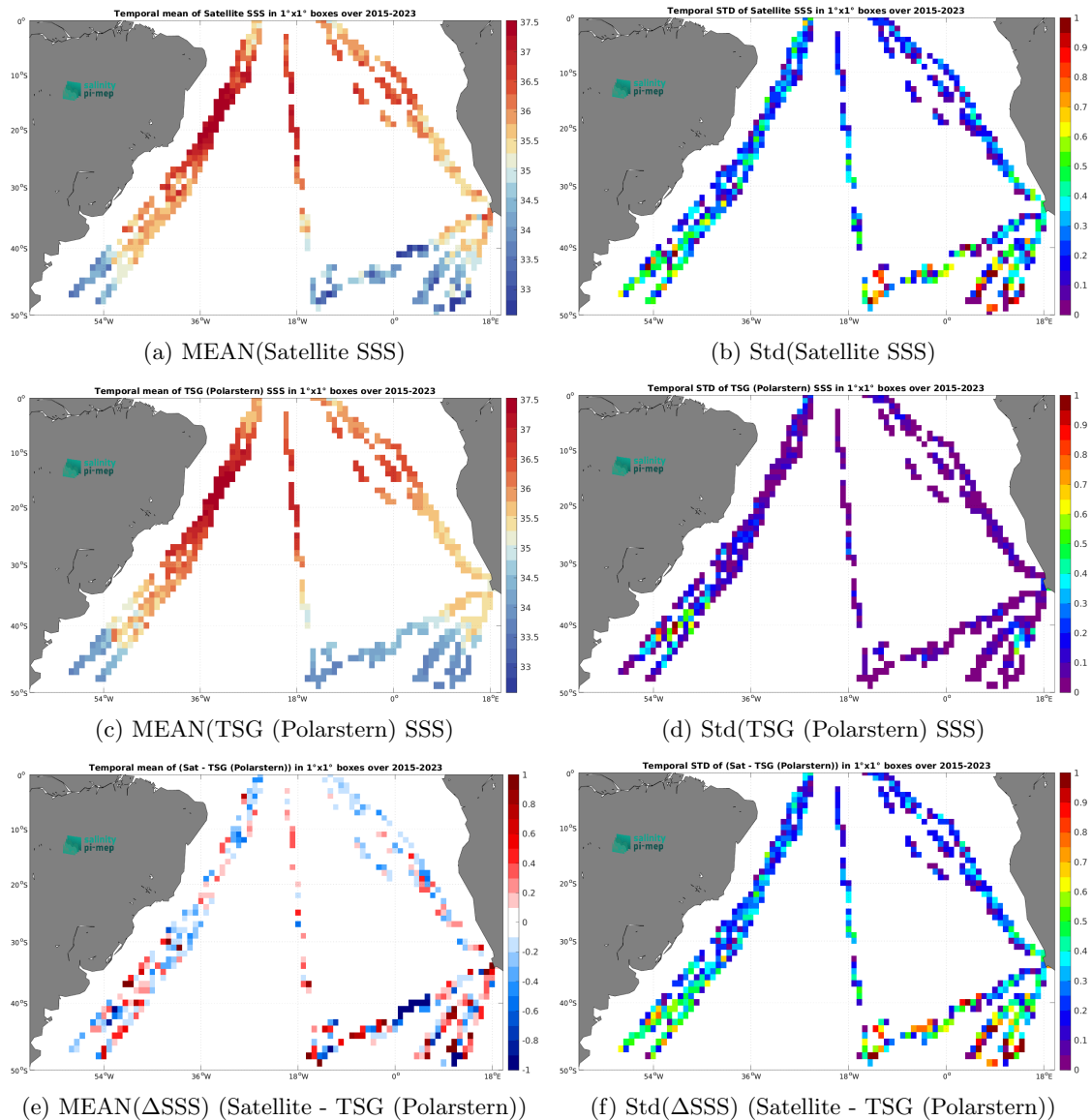
Figure 7: Temporal mean (left) and Std (right) of SSS from SMAP SSS L2 v5.3 (RSS) (top), TSG (Polarstern) (middle), and of \Delta SSS (Satellite - TSG (Polarstern)). Only match-up pairs are used to generate these maps.
