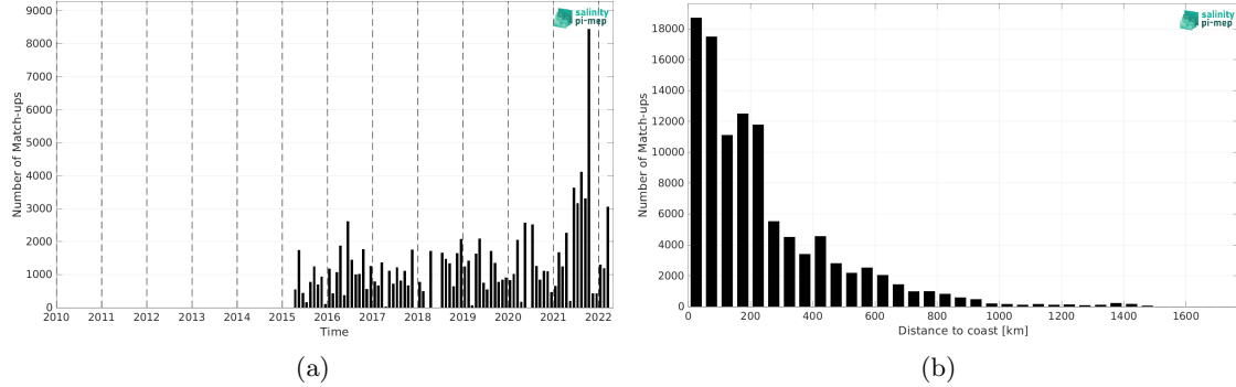
Figure 2: Number of match-ups between TSG (LEGOS-DM) and SMAP SSS L2 v5.3 (RSS) SSS as a function of time (a) and as function of the distance to coast (b) over the South Atlantic Ocean Pi-MEP region and for the full satellite product period.
