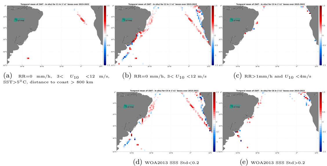
Figure 14: Temporal mean gridded over spatial boxes of size 1^\circ \times 1^\circ of \Delta SSS (SMAP SSS L2 v5.3 (RSS) - TSG (LEGOS-DM)) for 5 different subdatasets corresponding to:RR=0 mm/h, 3 < U_{10} < 12 m/s, SST>5°C, distance to coast > 800 km (a), RR=0 mm/h, 3 < U_{10} < 12 m/s (b), RR>1mm/h and U_{10} < 4 m/s (c), WOA2013 SSS Std<0.2 (d), WOA2013 SSS Std>0.2 (e).
