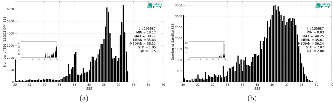
Figure 3: Histograms of SSS from TSG (LEGOS-DM) (a) and SMAP SSS L2 v5.3 (RSS) (b) considering all match-up pairs per bins of 0.1 over the South Atlantic Ocean Pi-MEP region and for the full satellite product period.
