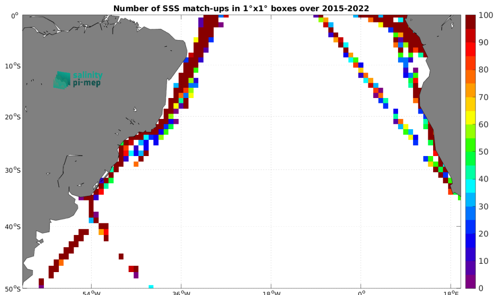
Figure 5: Number of SSS match-ups between TSG (LEGOS-DM) SSS and the SMAP SSS L2 v5.3 (RSS) SSS product for the South Atlantic Ocean Pi-MEP region over 1^\circ \times 1^\circ boxes and for the full satellite product period.
