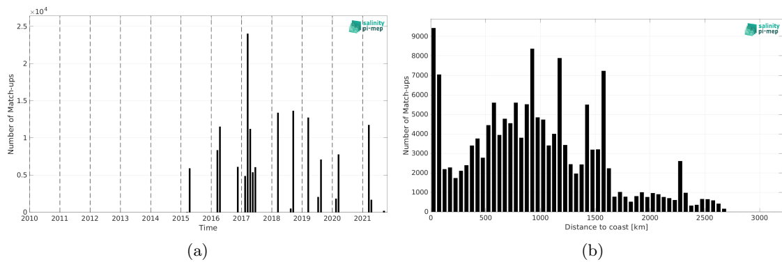
Figure 2: Number of match-ups between TSG (GOSUD-Research-vessel) and SMAP SSS L2 v5.3 (RSS) SSS as a function of time (a) and as function of the distance to coast (b) over the South Atlantic Ocean Pi-MEP region and for the full satellite product period.
