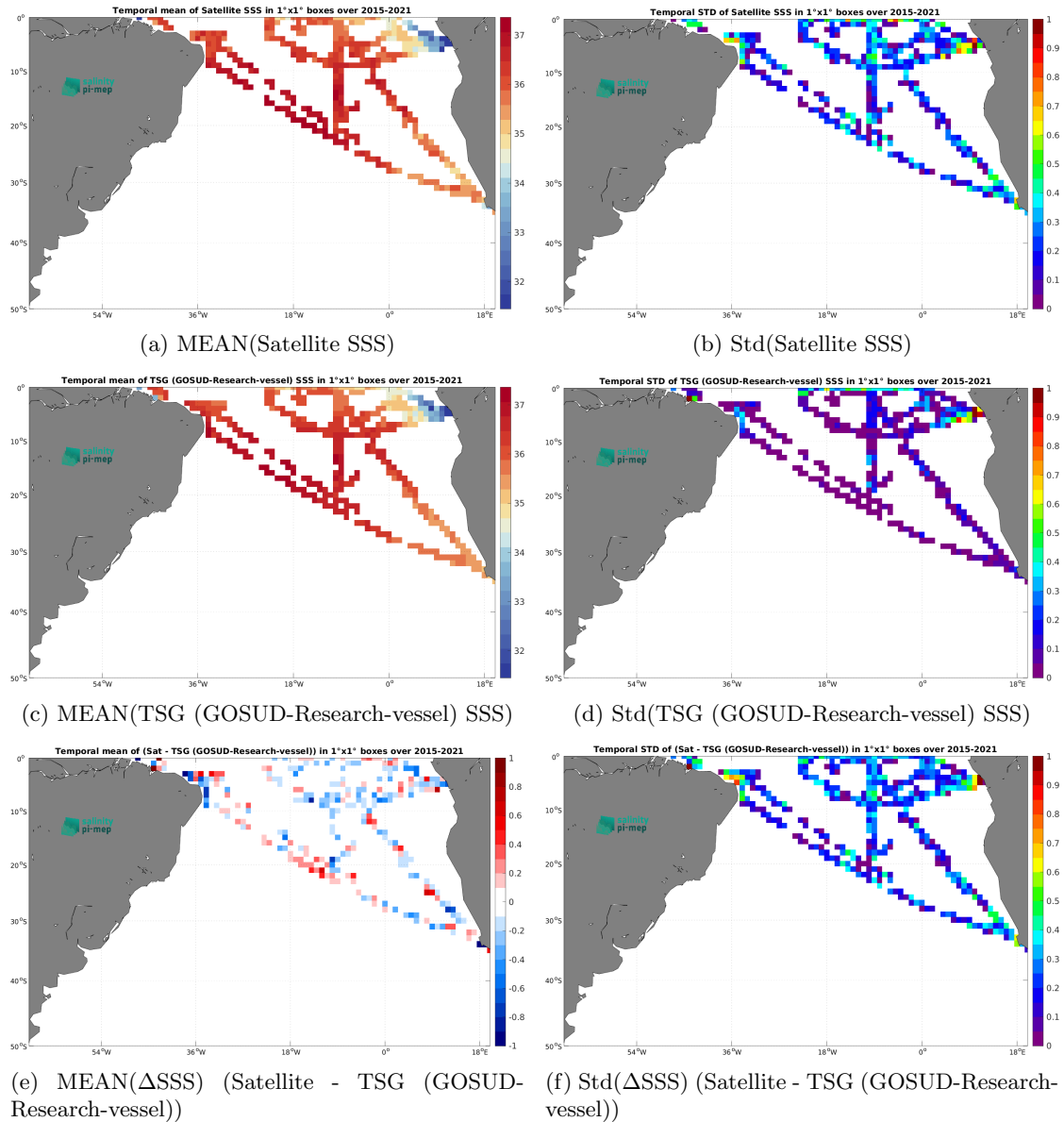
Figure 7: Temporal mean (left) and Std (right) of SSS from SMAP SSS L2 v5.3 (RSS) (top), TSG (GOSUD-Research-vessel) (middle), and of \Delta SSS (Satellite - TSG (GOSUD-Research-vessel)). Only match-up pairs are used to generate these maps.
