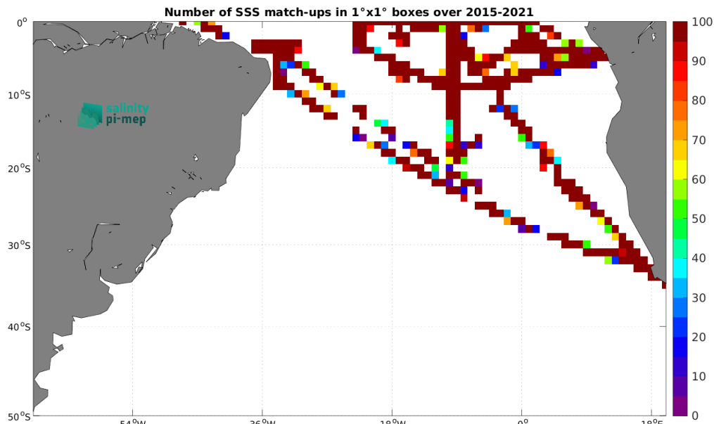
Figure 5: Number of SSS match-ups between TSG (GOSUD-Research-vessel) SSS and the SMAP SSS L2 v5.3 (RSS) SSS product for the South Atlantic Ocean Pi-MEP region over 1^\circ \times 1^\circ boxes and for the full satellite product period.
