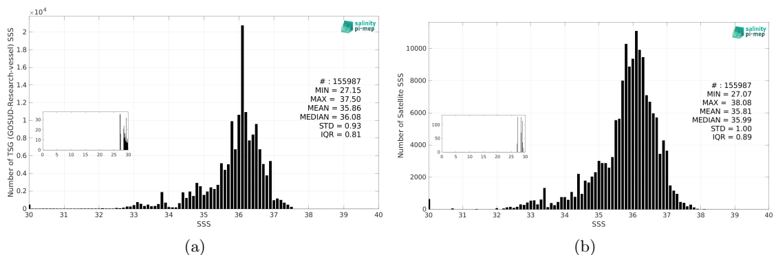
Figure 3: Histograms of SSS from TSG (GOSUD-Research-vessel) (a) and SMAP SSS L2 v5.3 (RSS) (b) considering all match-up pairs per bins of 0.1 over the South Atlantic Ocean Pi-MEP region and for the full satellite product period.
