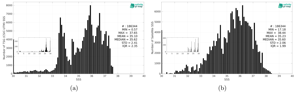
Figure 3: Histograms of SSS from TSG (CSIC-UTM) (a) and SMAP SSS L2 v5.3 (RSS) (b) considering all match-up pairs per bins of 0.1 over the South Atlantic Ocean Pi-MEP region and for the full satellite product period.
