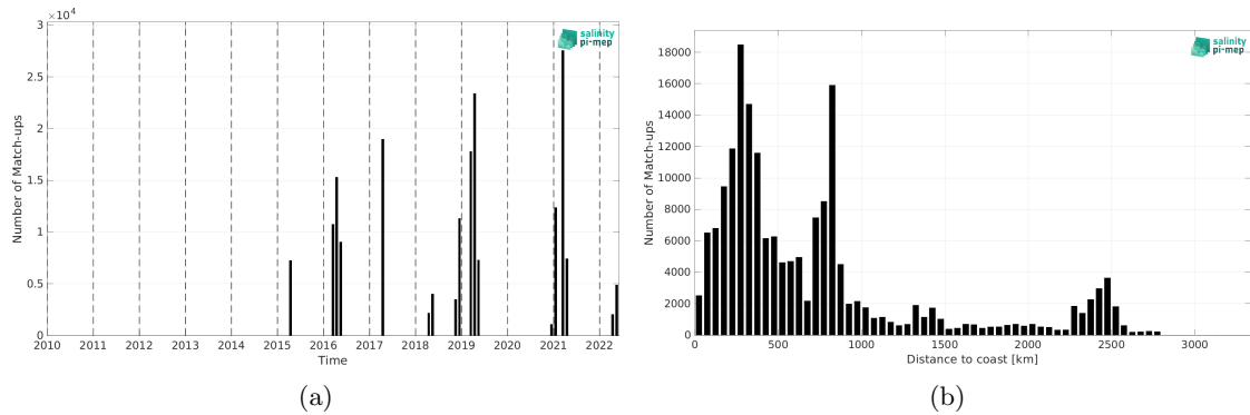
Figure 2: Number of match-ups between TSG (CSIC-UTM) and SMAP SSS L2 v5.3 (RSS) SSS as a function of time (a) and as function of the distance to coast (b) over the South Atlantic Ocean Pi-MEP region and for the full satellite product period.
