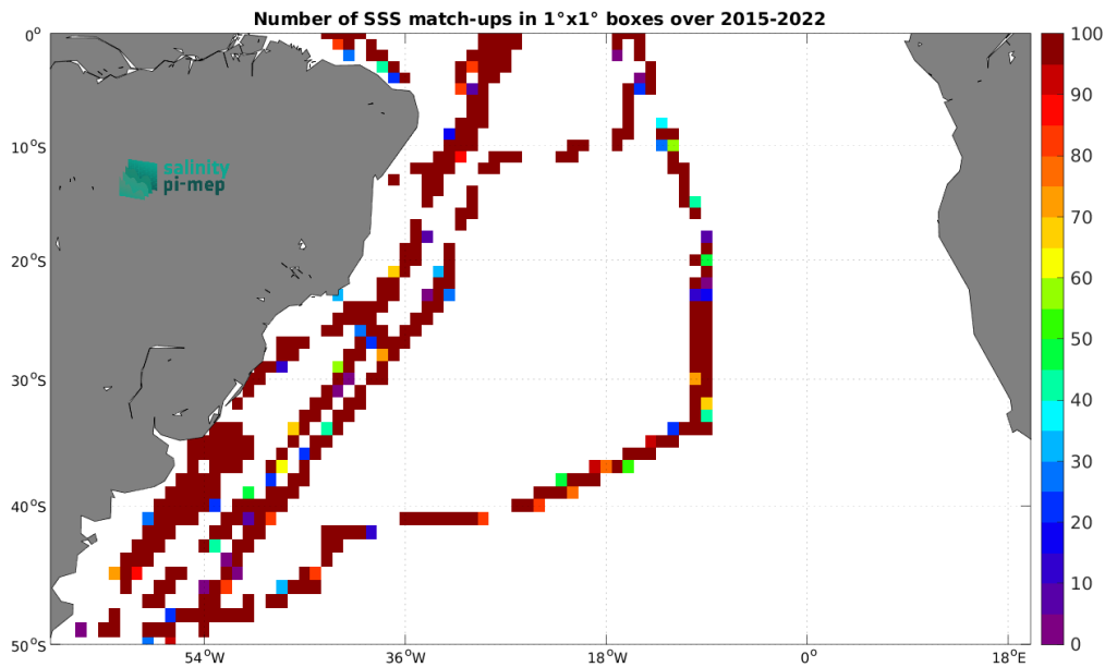
Figure 5: Number of SSS match-ups between TSG (CSIC-UTM) SSS and the SMAP SSS L2 v5.3 (RSS) SSS product for the South Atlantic Ocean Pi-MEP region over 1^\circ \times 1^\circ boxes and for the full satellite product period.
