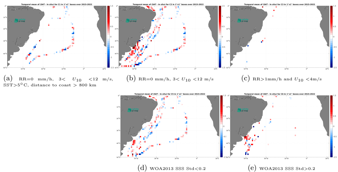
Figure 14: Temporal mean gridded over spatial boxes of size 1^\circ \times 1^\circ of \Delta SSS (SMAP SSS L2 v5.3 (RSS) - TSG (CSIC-UTM)) for 5 different subdatasets corresponding to:RR=0 mm/h, 3 < U_{10} < 12 m/s, SST>5°C, distance to coast > 800 km (a), RR=0 mm/h, 3 < U_{10} < 12 m/s (b), RR>1mm/h and U_{10} < 4 m/s (c), WOA2013 SSS Std<0.2 (d), WOA2013 SSS Std>0.2 (e).
