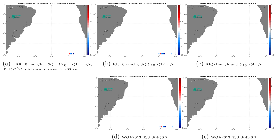
Figure 14: Temporal mean gridded over spatial boxes of size 1^\circ \times 1^\circ of \Delta SSS (SMAP SSS L2 v5.3 (RSS) - Saldrone) for 5 different subdatasets corresponding to:RR=0 mm/h, 3 < U_{10} < 12 m/s, SST >5^\circ\text{C} , distance to coast > 800 km (a), RR=0 mm/h, 3 < U_{10} < 12 m/s (b), RR >1 mm/h and U_{10} < 4 m/s (c), WOA2013 SSS Std <0.2 (d), WOA2013 SSS Std >0.2 (e).
