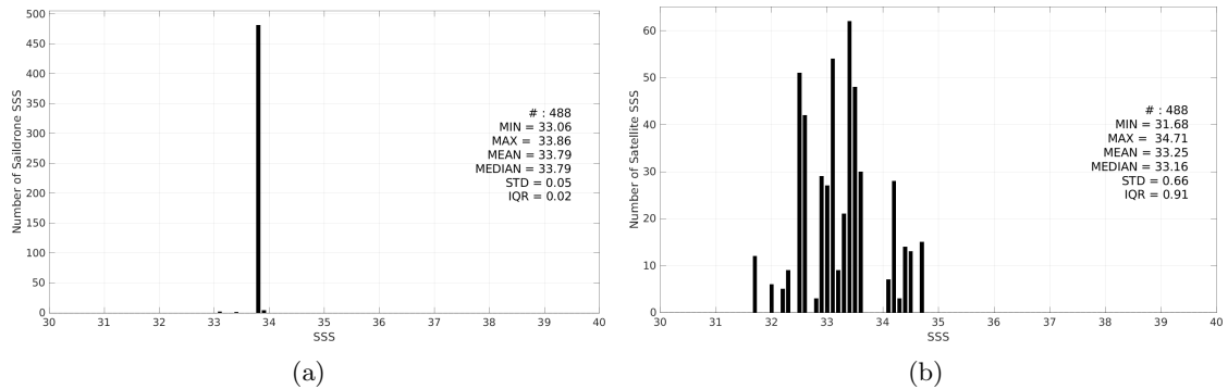
Figure 3: Histograms of SSS from Saildrone (a) and SMAP SSS L2 v5.3 (RSS) (b) considering all match-up pairs per bins of 0.1 over the South Atlantic Ocean Pi-MEP region and for the full satellite product period.
