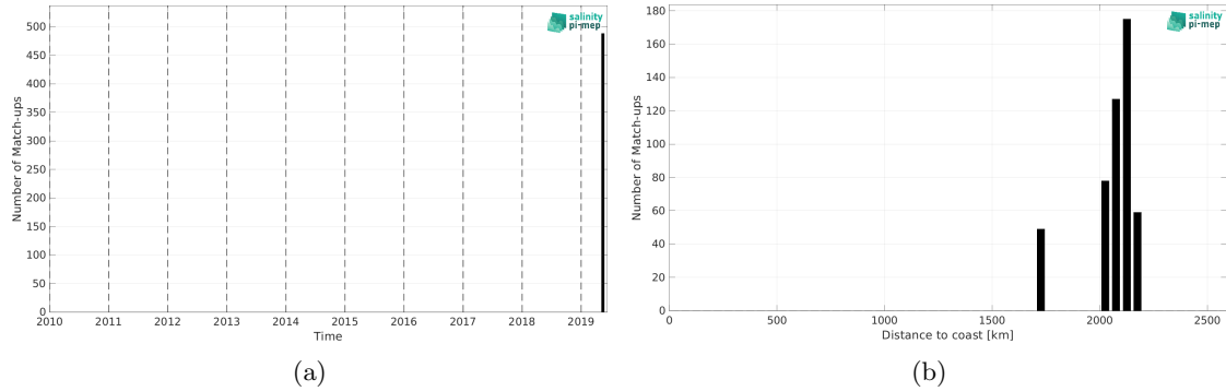
Figure 2: Number of match-ups between Saildrone and SMAP SSS L2 v5.3 (RSS) SSS as a function of time (a) and as function of the distance to coast (b) over the South Atlantic Ocean Pi-MEP region and for the full satellite product period.
