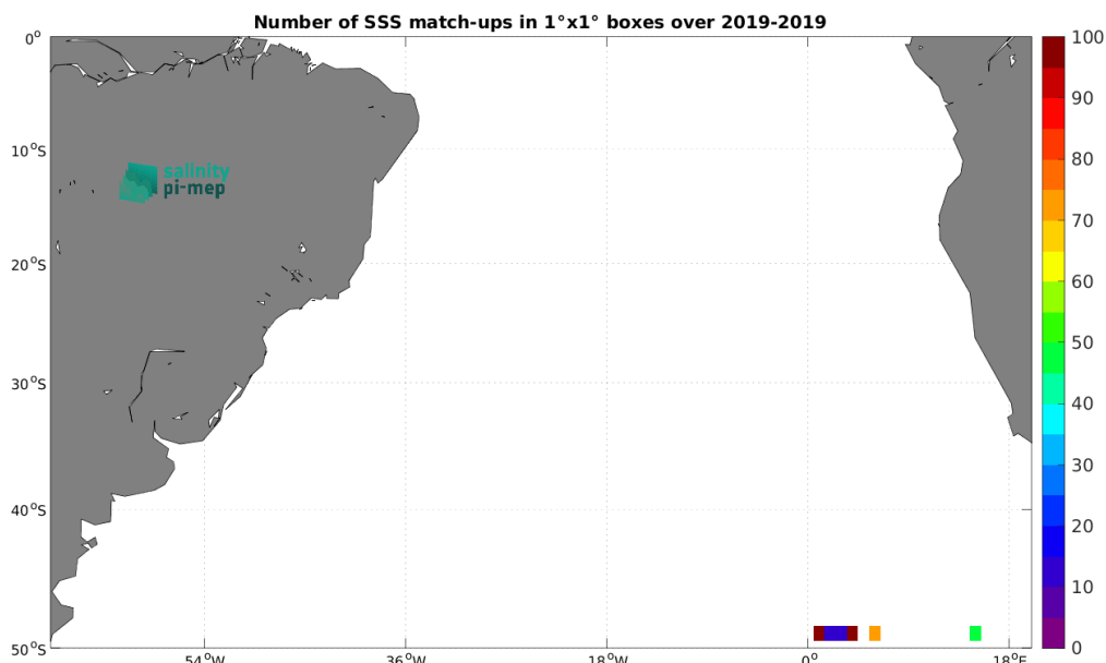
Figure 5: Number of SSS match-ups between Saildrone SSS and the SMAP SSS L2 v5.3 (RSS) SSS product for the South Atlantic Ocean Pi-MEP region over 1^\circ \times 1^\circ boxes and for the full satellite product period.
