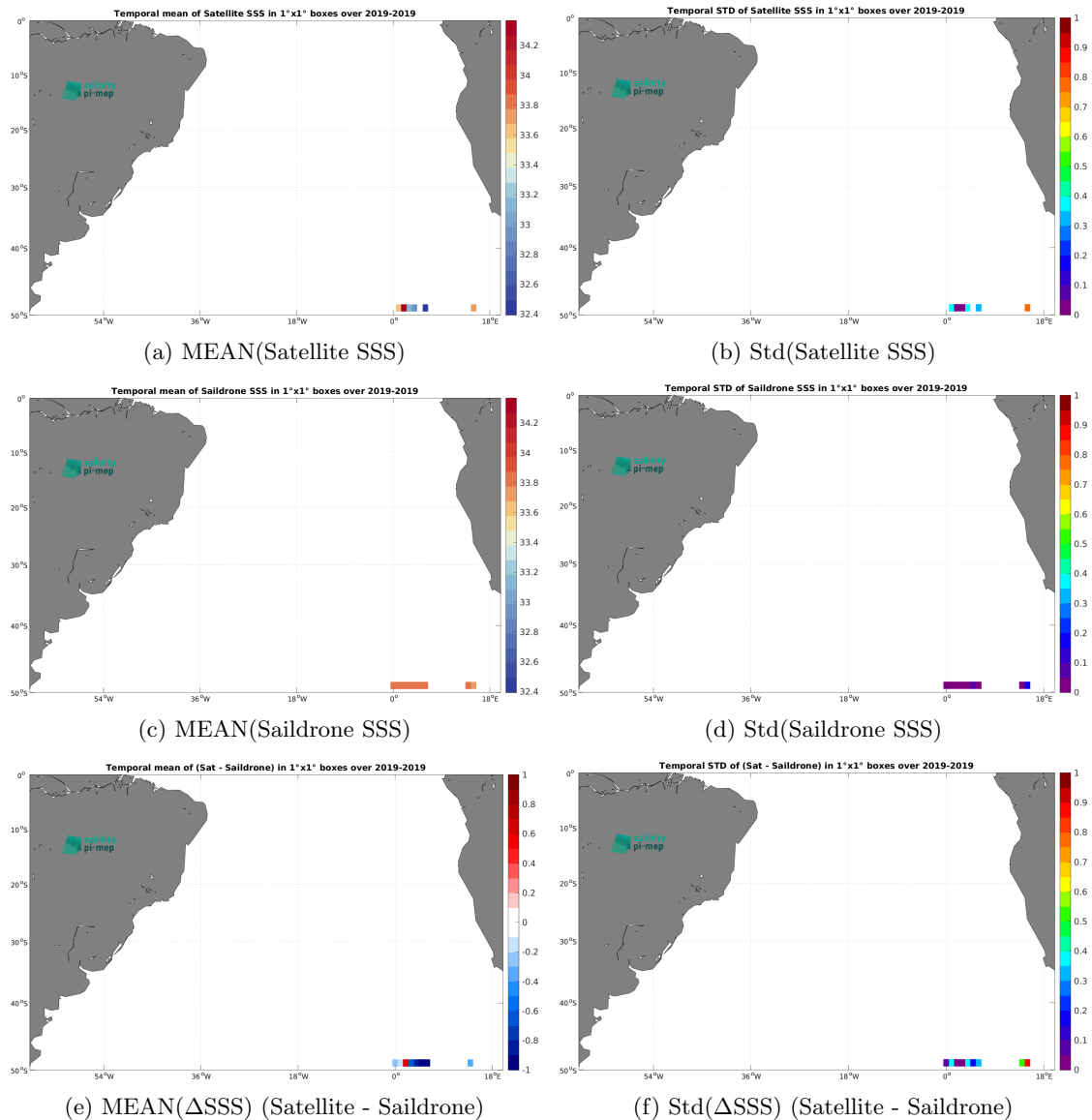
Figure 7: Temporal mean (left) and Std (right) of SSS from SMAP SSS L2 v5.3 (RSS) (top), Saildrone (middle), and of \Delta SSS (Satellite - Saildrone). Only match-up pairs are used to generate these maps.
