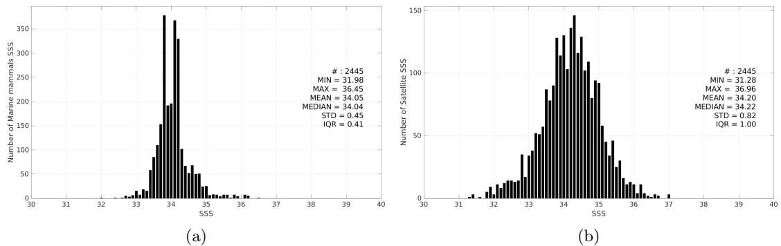
Figure 3: Histograms of SSS from Marine mammals (a) and SMAP SSS L2 v5.3 (RSS) (b) considering all match-up pairs per bins of 0.1 over the South Atlantic Ocean Pi-MEP region and for the full satellite product period.
