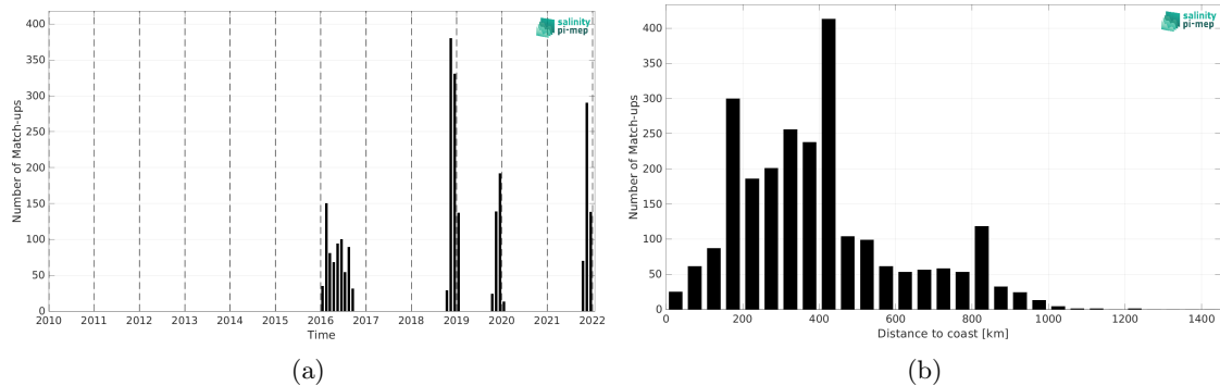
Figure 2: Number of match-ups between Marine mammals and SMAP SSS L2 v5.3 (RSS) SSS as a function of time (a) and as function of the distance to coast (b) over the South Atlantic Ocean Pi-MEP region and for the full satellite product period.
