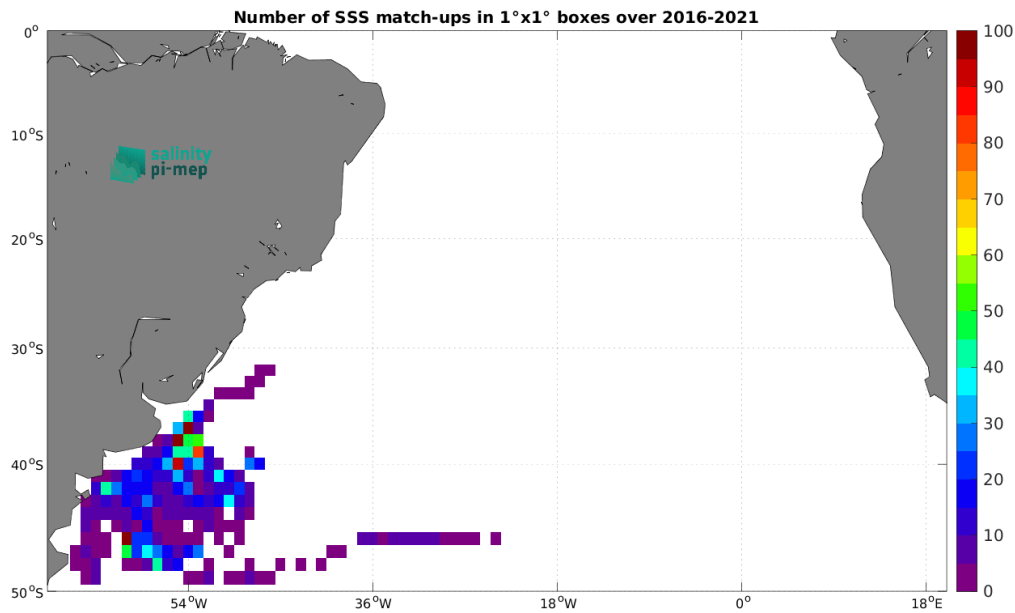
Figure 5: Number of SSS match-ups between Marine mammals SSS and the SMAP SSS L2 v5.3 (RSS) SSS product for the South Atlantic Ocean Pi-MEP region over 1^\circ \times 1^\circ boxes and for the full satellite product period.
