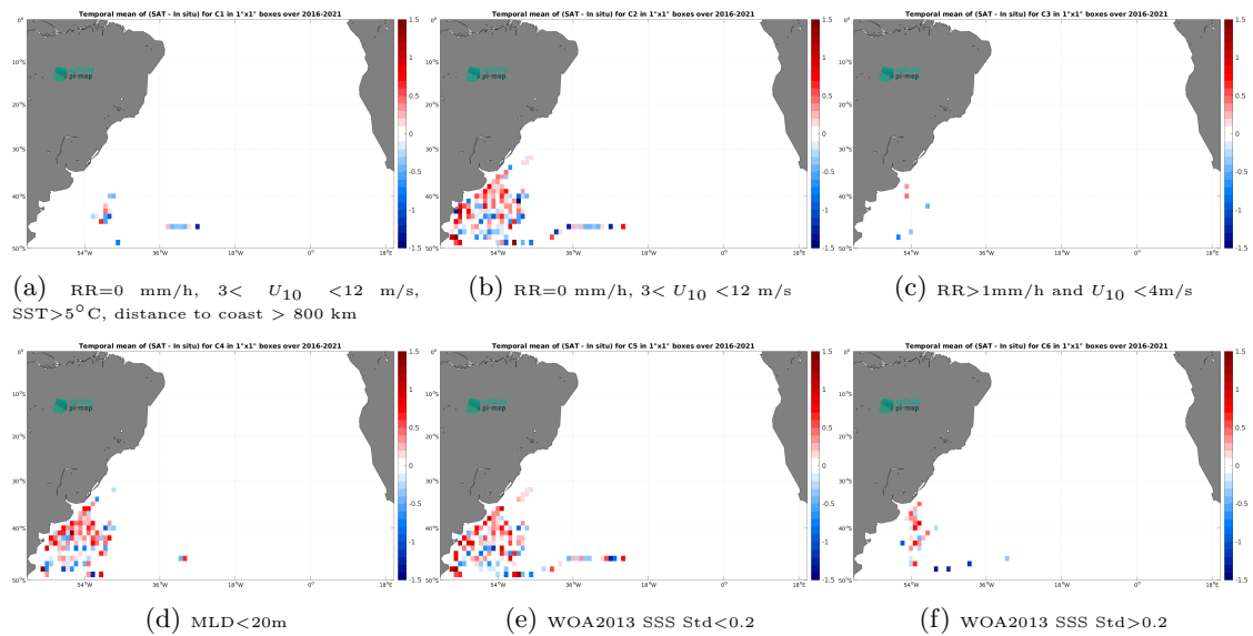
Figure 14: Temporal mean gridded over spatial boxes of size 1^\circ \times 1^\circ of \Delta SSS (SMAP SSS L2 v5.3 (RSS) - Marine mammals) for 6 different subdatasets corresponding to:RR=0 mm/h, 3 < U_{10} < 12 m/s, SST >5^\circ C, distance to coast > 800 km (a), RR=0 mm/h, 3 < U_{10} < 12 m/s (b), RR >1 mm/h and U_{10} < 4 m/s (c),MLD <20 m (d),WOA2013 SSS Std <0.2 (e),WOA2013 SSS Std >0.2 (f).
