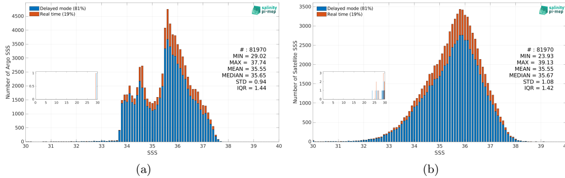
Figure 3: Histograms of SSS from Argo (a) and SMAP SSS L2 v5.3 (RSS) (b) considering all match-up pairs per bins of 0.1 over the South Atlantic Ocean Pi-MEP region and for the full satellite product period.
