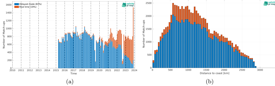
Figure 2: Number of match-ups between Argo and SMAP SSS L2 v5.3 (RSS) SSS as a function of time (a) and as function of the distance to coast (b) over the South Atlantic Ocean Pi-MEP region and for the full satellite product period.
