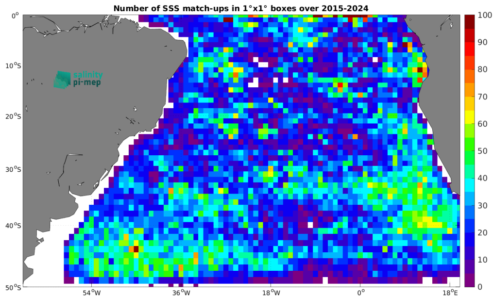
Figure 5: Number of SSS match-ups between Argo SSS and the SMAP SSS L2 v5.3 (RSS) SSS product for the South Atlantic Ocean Pi-MEP region over 1^\circ \times 1^\circ boxes and for the full satellite product period.
