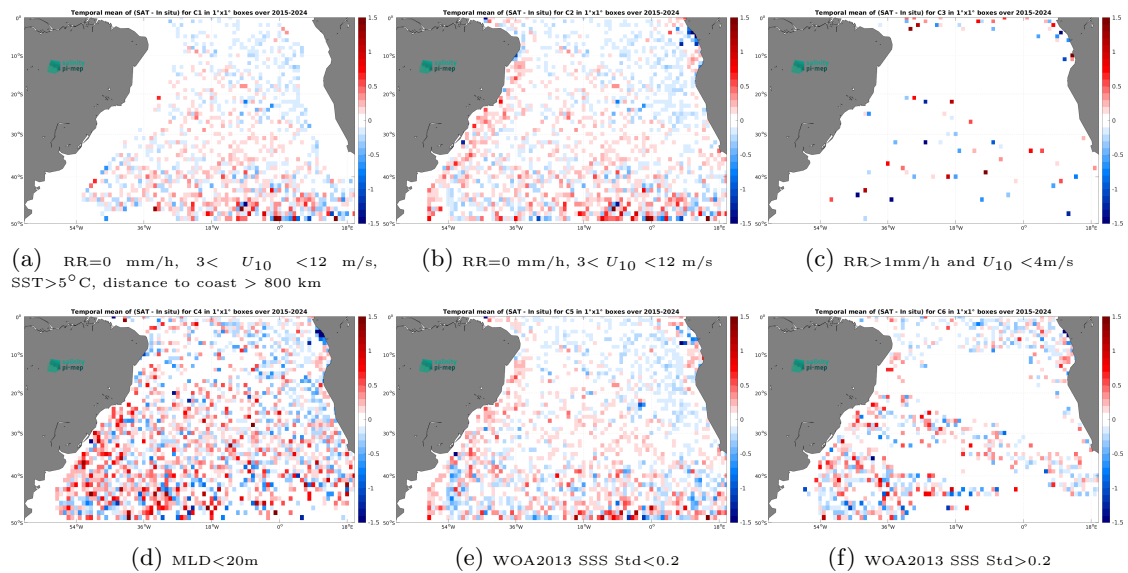
Figure 14: Temporal mean gridded over spatial boxes of size 1^\circ \times 1^\circ of \Delta\text{SSS} (SMAP SSS L2 v5.3 (RSS) - Argo) for 6 different subdatasets corresponding to:RR=0 mm/h, 3 < U_{10} < 12 m/s, SST>5°C, distance to coast > 800 km (a), RR=0 mm/h, 3 < U_{10} < 12 m/s (b), RR>1mm/h and U_{10} < 4 m/s (c),MLD<20m (d),WOA2013 SSS Std<0.2 (e),WOA2013 SSS Std>0.2 (f).
