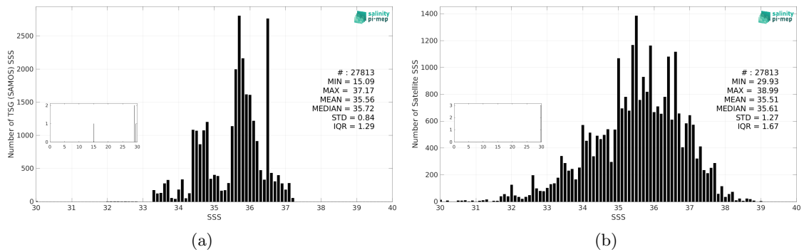
Figure 3: Histograms of SSS from TSG (SAMOS) (a) and SMAP SSS L2 v5.3 - 40 km (RSS) (b) considering all match-up pairs per bins of 0.1 over the South Atlantic Ocean Pi-MEP region and for the full satellite product period.
