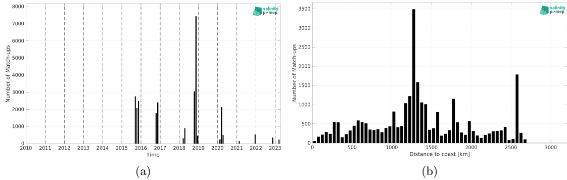
Figure 2: Number of match-ups between TSG (SAMOS) and SMAP SSS L2 v5.3 - 40 km (RSS) SSS as a function of time (a) and as function of the distance to coast (b) over the South Atlantic Ocean Pi-MEP region and for the full satellite product period.
