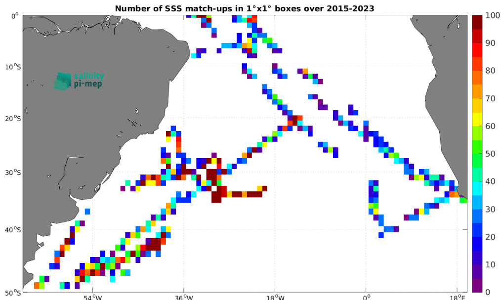
Figure 5: Number of SSS match-ups between TSG (SAMOS) SSS and the SMAP SSS L2 v5.3 - 40 km (RSS) SSS product for the South Atlantic Ocean Pi-MEP region over 1^\circ \times 1^\circ boxes and for the full satellite product period.
