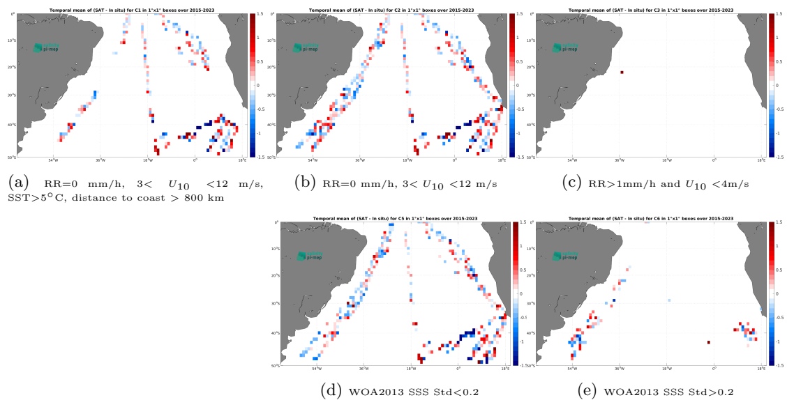
Figure 14: Temporal mean gridded over spatial boxes of size 1^\circ \times 1^\circ of \Delta SSS (SMAP SSS L2 v5.3 - 40 km (RSS) - TSG (Polarstern)) for 5 different subdatasets corresponding to:RR=0 mm/h, 3 < U_{10} < 12 m/s, SST >5^\circ\text{C} , distance to coast > 800 km (a), RR=0 mm/h, 3 < U_{10} < 12 m/s (b), RR >1 mm/h and U_{10} < 4 m/s (c), WOA2013 SSS Std <0.2 (d), WOA2013 SSS Std >0.2 (e).
