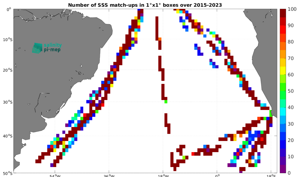
Figure 5: Number of SSS match-ups between TSG (Polarstern) SSS and the SMAP SSS L2 v5.3 - 40 km (RSS) SSS product for the South Atlantic Ocean Pi-MEP region over 1^\circ \times 1^\circ boxes and for the full satellite product period.
