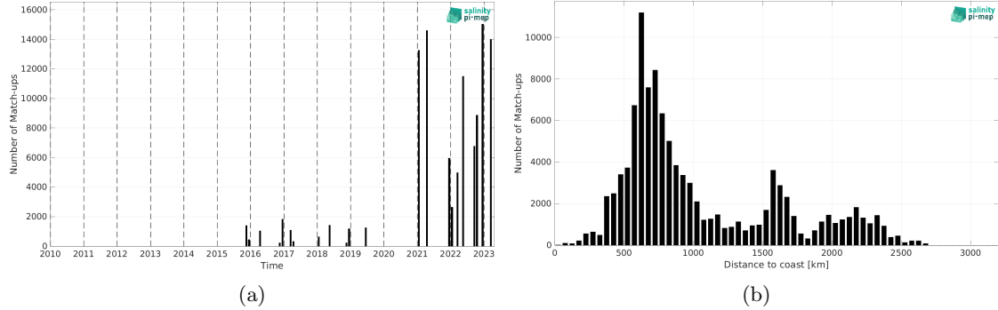
Figure 2: Number of match-ups between TSG (Polarstern) and SMAP SSS L2 v5.3 - 40 km (RSS) SSS as a function of time (a) and as function of the distance to coast (b) over the South Atlantic Ocean Pi-MEP region and for the full satellite product period.
