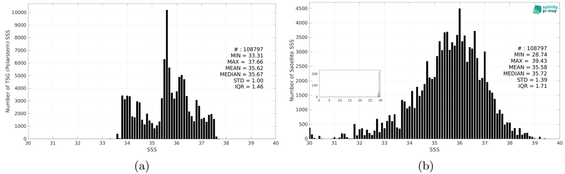
Figure 3: Histograms of SSS from TSG (Polarstern) (a) and SMAP SSS L2 v5.3 - 40 km (RSS) (b) considering all match-up pairs per bins of 0.1 over the South Atlantic Ocean Pi-MEP region and for the full satellite product period.
