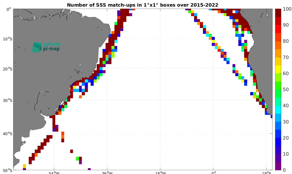
Figure 5: Number of SSS match-ups between TSG (LEGOS-DM) SSS and the SMAP SSS L2 v5.3 - 40 km (RSS) SSS product for the South Atlantic Ocean Pi-MEP region over 1^\circ \times 1^\circ boxes and for the full satellite product period.
