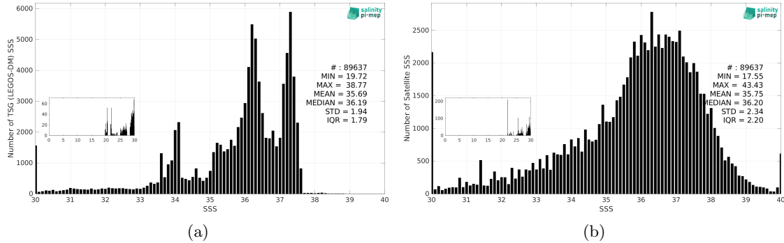
Figure 3: Histograms of SSS from TSG (LEGOS-DM) (a) and SMAP SSS L2 v5.3 - 40 km (RSS) (b) considering all match-up pairs per bins of 0.1 over the South Atlantic Ocean Pi-MEP region and for the full satellite product period.
