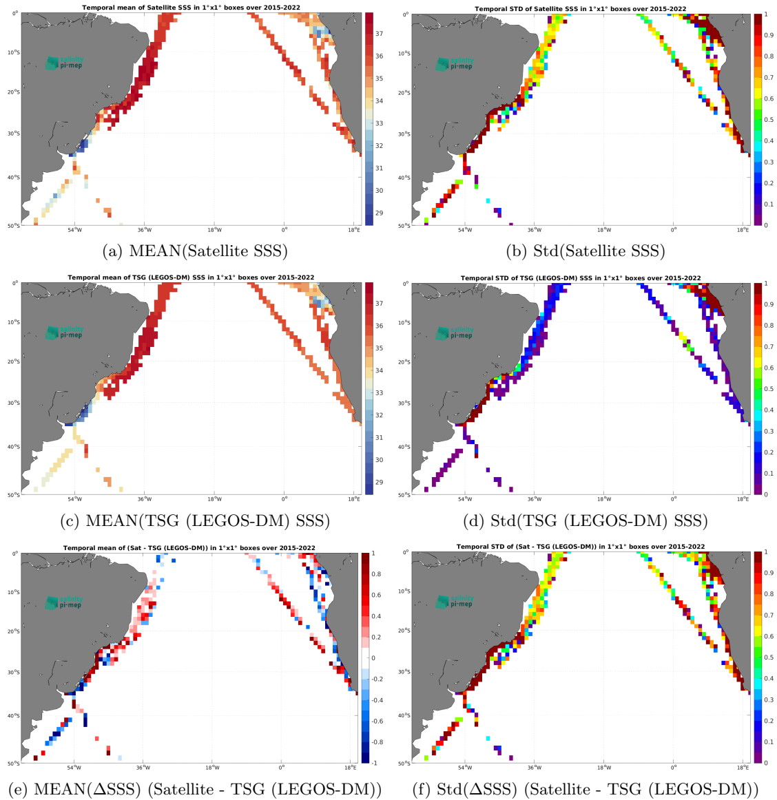
Figure 7: Temporal mean (left) and Std (right) of SSS from SMAP SSS L2 v5.3 - 40 km (RSS) (top), TSG (LEGOS-DM) (middle), and of \Delta SSS (Satellite - TSG (LEGOS-DM)). Only match-up pairs are used to generate these maps.
