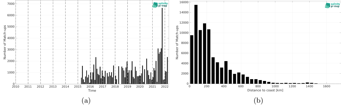
Figure 2: Number of match-ups between TSG (LEGOS-DM) and SMAP SSS L2 v5.3 - 40 km (RSS) SSS as a function of time (a) and as function of the distance to coast (b) over the South Atlantic Ocean Pi-MEP region and for the full satellite product period.
