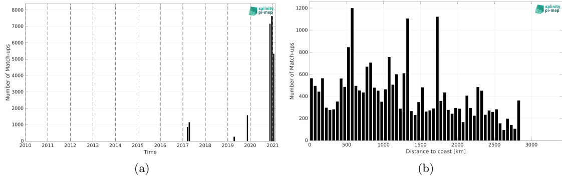
Figure 2: Number of match-ups between TSG (GOSUD-Sailing-ship) and SMAP SSS L2 v5.3 - 40 km (RSS) SSS as a function of time (a) and as function of the distance to coast (b) over the South Atlantic Ocean Pi-MEP region and for the full satellite product period.
