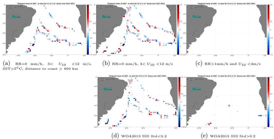
Figure 14: Temporal mean gridded over spatial boxes of size 1^\circ \times 1^\circ of \Delta\text{SSS} (SMAP SSS L2 v5.3 - 40 km (RSS) - TSG (GOSUD-Sailing-ship)) for 5 different subdatasets corresponding to:RR=0 mm/h, 3 < U_{10} < 12 m/s, SST>5°C, distance to coast > 800 km (a), RR=0 mm/h, 3 < U_{10} < 12 m/s (b), RR>1mm/h and U_{10} < 4 m/s (c), WOA2013 SSS Std<0.2 (d), WOA2013 SSS Std>0.2 (e).
