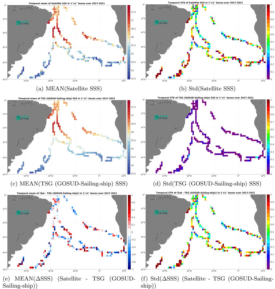
Figure 7: Temporal mean (left) and Std (right) of SSS from SMAP SSS L2 v5.3 - 40 km (RSS) (top), TSG (GOSUD-Sailing-ship) (middle), and of \Delta SSS (Satellite - TSG (GOSUD-Sailing-ship)). Only match-up pairs are used to generate these maps.
