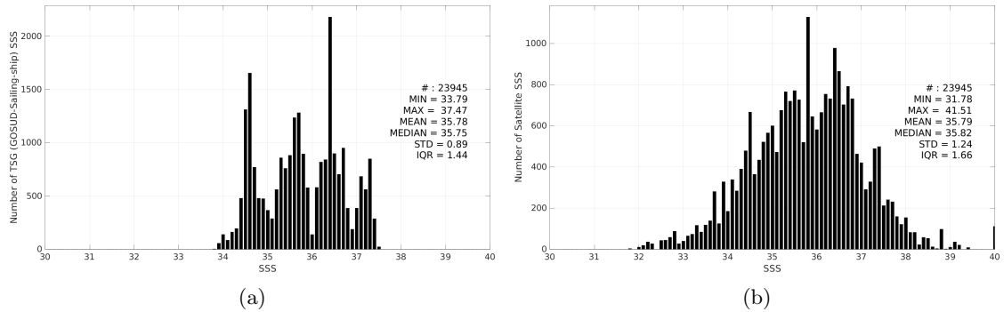
Figure 3: Histograms of SSS from TSG (GOSUD-Sailing-ship) (a) and SMAP SSS L2 v5.3 - 40 km (RSS) (b) considering all match-up pairs per bins of 0.1 over the South Atlantic Ocean Pi-MEP region and for the full satellite product period.
