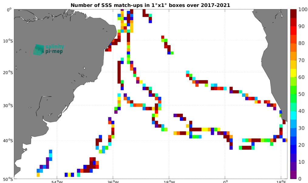
Figure 5: Number of SSS match-ups between TSG (GOSUD-Sailing-ship) SSS and the SMAP SSS L2 v5.3 - 40 km (RSS) SSS product for the South Atlantic Ocean Pi-MEP region over 1^\circ \times 1^\circ boxes and for the full satellite product period.
