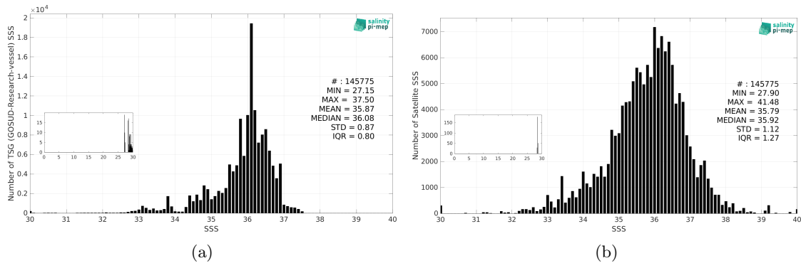
Figure 3: Histograms of SSS from TSG (GOSUD-Research-vessel) (a) and SMAP SSS L2 v5.3 - 40 km (RSS) (b) considering all match-up pairs per bins of 0.1 over the South Atlantic Ocean Pi-MEP region and for the full satellite product period.
