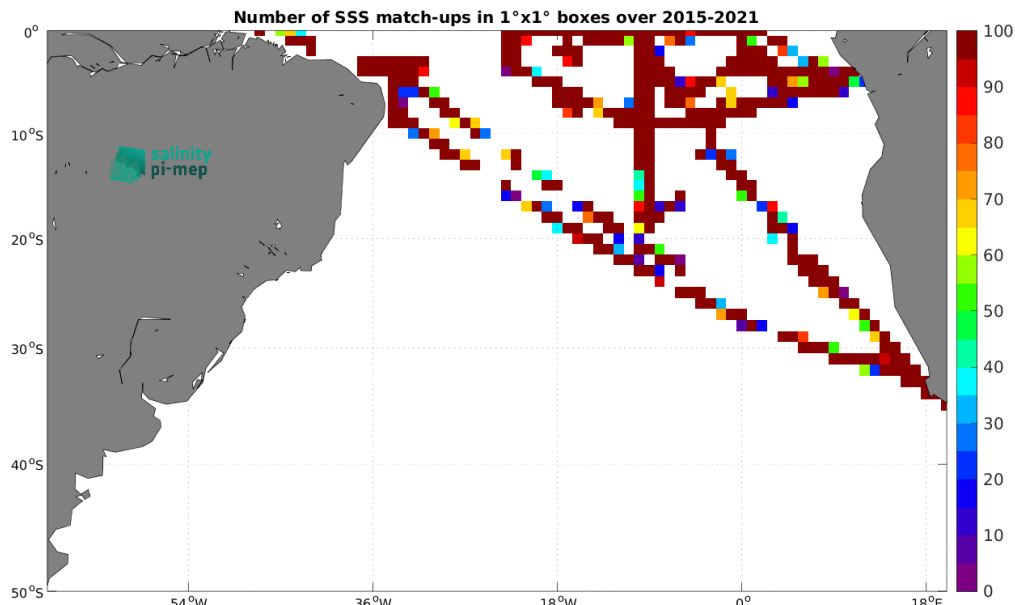
Figure 5: Number of SSS match-ups between TSG (GOSUD-Research-vessel) SSS and the SMAP SSS L2 v5.3 - 40 km (RSS) SSS product for the South Atlantic Ocean Pi-MEP region over 1^\circ \times 1^\circ boxes and for the full satellite product period.
