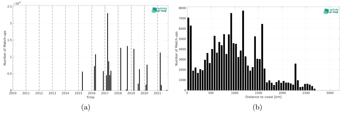
Figure 2: Number of match-ups between TSG (GOSUD-Research-vessel) and SMAP SSS L2 v5.3 - 40 km (RSS) SSS as a function of time (a) and as function of the distance to coast (b) over the South Atlantic Ocean Pi-MEP region and for the full satellite product period.
