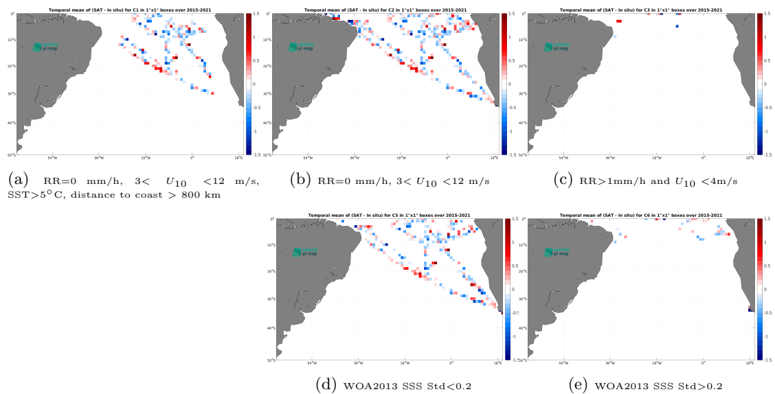
Figure 14: Temporal mean gridded over spatial boxes of size 1^\circ \times 1^\circ of \Delta SSS (SMAP SSS L2 v5.3 - 40 km (RSS) - TSG (GOSUD-Research-vessel)) for 5 different subdatasets corresponding to:RR=0 mm/h, 3 < U_{10} < 12 m/s, SST>5°C, distance to coast > 800 km (a), RR=0 mm/h, 3 < U_{10} < 12 m/s (b), RR>1mm/h and U_{10} < 4 m/s (c), WOA2013 SSS Std<0.2 (d), WOA2013 SSS Std>0.2 (e).
