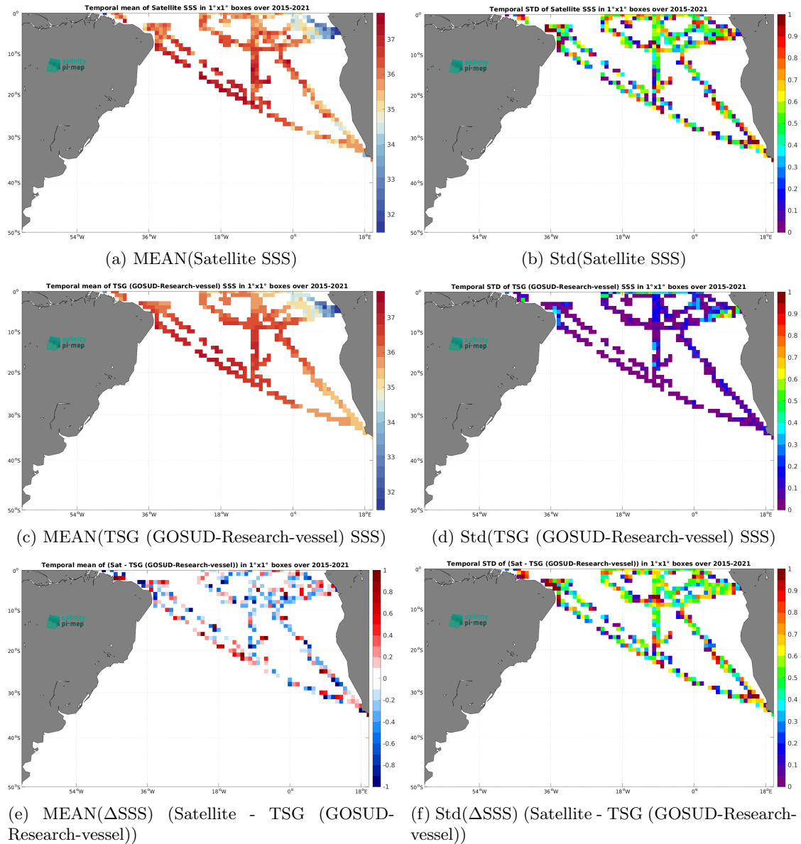
Figure 7: Temporal mean (left) and Std (right) of SSS from SMAP SSS L2 v5.3 - 40 km (RSS) (top), TSG (GOSUD-Research-vessel) (middle), and of \Delta SSS (Satellite - TSG (GOSUD-Research-vessel)). Only match-up pairs are used to generate these maps.
