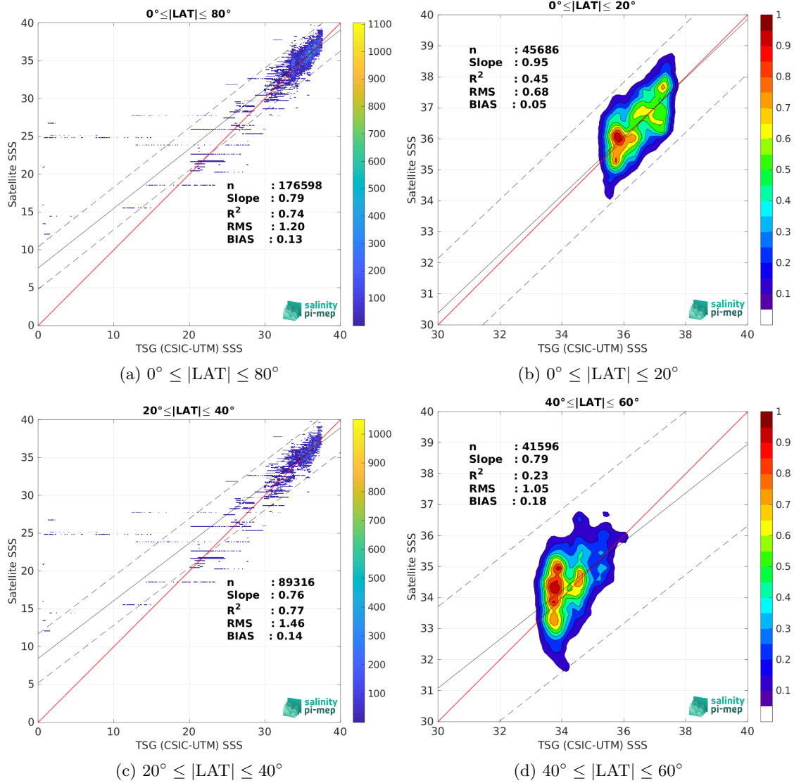
Figure 10: Contour maps of the concentration of SMAP SSS L2 v5.3 - 40 km (RSS) SSS ( y -axis) versus TSG (CSIC-UTM) SSS ( x -axis) at match-up pairs for different latitude bands. For each plot, the red line shows x=y . The black thin and dashed lines indicate a linear fit through the data cloud and the \pm 95\% confidence levels, respectively. The number match-up pairs n , the slope and R^2 coefficient of the linear fit, the root mean square (RMS) and the mean bias between satellite and in situ data are indicated for each latitude band in each plots.
