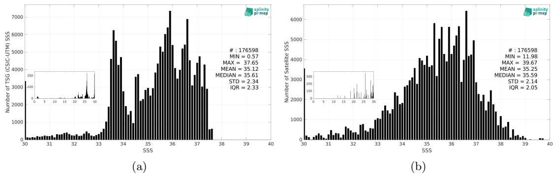
Figure 3: Histograms of SSS from TSG (CSIC-UTM) (a) and SMAP SSS L2 v5.3 - 40 km (RSS) (b) considering all match-up pairs per bins of 0.1 over the South Atlantic Ocean Pi-MEP region and for the full satellite product period.
