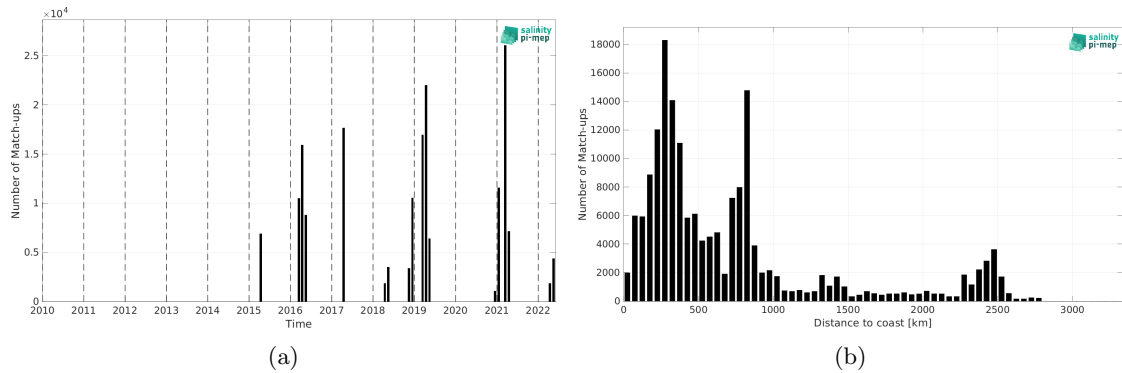
Figure 2: Number of match-ups between TSG (CSIC-UTM) and SMAP SSS L2 v5.3 - 40 km (RSS) SSS as a function of time (a) and as function of the distance to coast (b) over the South Atlantic Ocean Pi-MEP region and for the full satellite product period.
