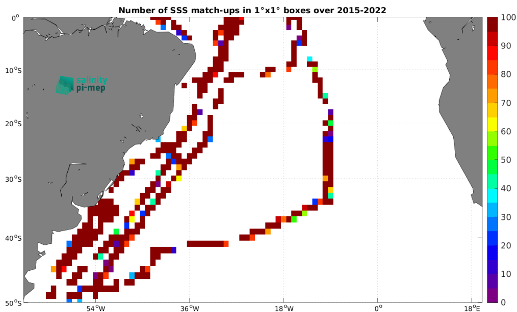
Figure 5: Number of SSS match-ups between TSG (CSIC-UTM) SSS and the SMAP SSS L2 v5.3 - 40 km (RSS) SSS product for the South Atlantic Ocean Pi-MEP region over 1^\circ \times 1^\circ boxes and for the full satellite product period.
