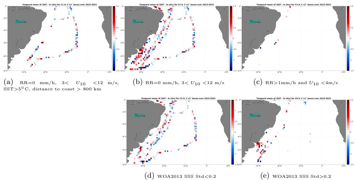
Figure 14: Temporal mean gridded over spatial boxes of size 1^\circ \times 1^\circ of \Delta\text{SSS} (SMAP SSS L2 v5.3 - 40 km (RSS) - TSG (CSIC-UTM)) for 5 different subdatasets corresponding to:RR=0 mm/h, 3 < U_{10} < 12 m/s, SST>5°C, distance to coast > 800 km (a), RR=0 mm/h, 3 < U_{10} < 12 m/s (b), RR>1mm/h and U_{10} < 4 m/s (c), WOA2013 SSS Std<0.2 (d), WOA2013 SSS Std>0.2 (e).
