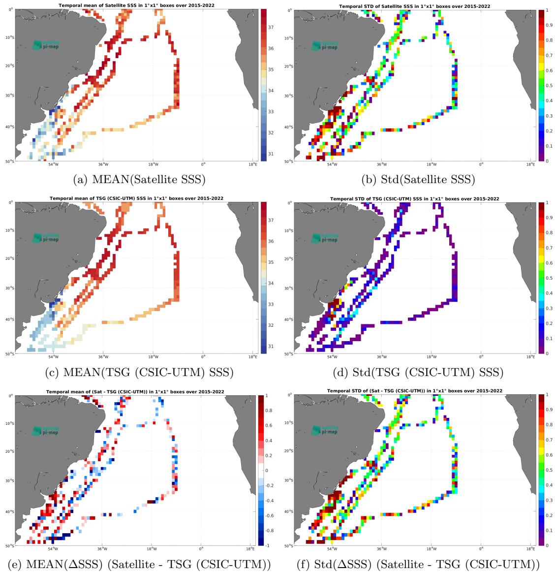
Figure 7: Temporal mean (left) and Std (right) of SSS from SMAP SSS L2 v5.3 - 40 km (RSS) (top), TSG (CSIC-UTM) (middle), and of \Delta SSS (Satellite - TSG (CSIC-UTM)). Only match-up pairs are used to generate these maps.
