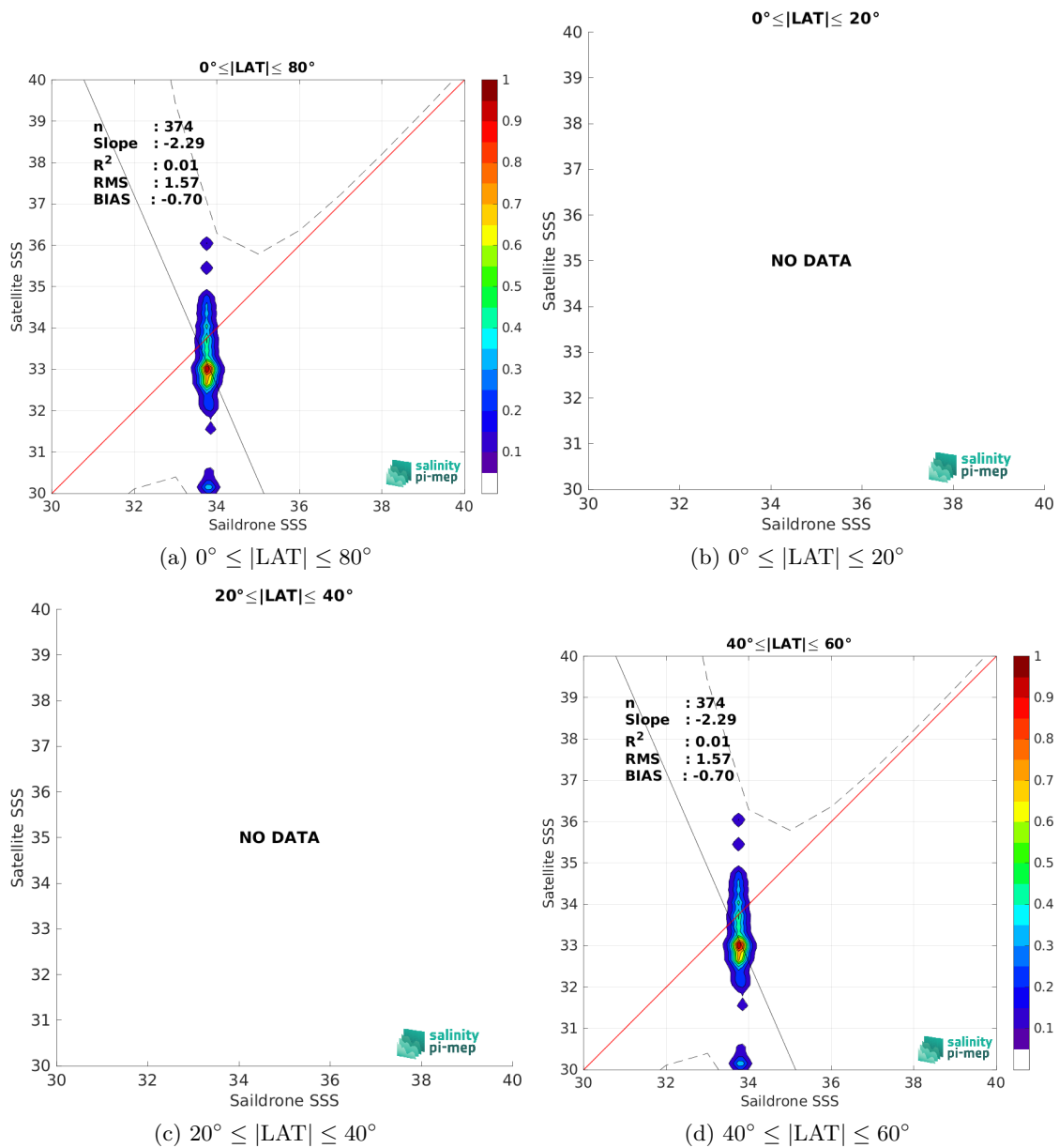
Figure 10: Contour maps of the concentration of SMAP SSS L2 v5.3 - 40 km (RSS) SSS (y-axis) versus Saildrone SSS (x-axis) at match-up pairs for different latitude bands. For each plot, the red line shows x=y . The black thin and dashed lines indicate a linear fit through the data cloud and the \pm 95\% confidence levels, respectively. The number match-up pairs n , the slope and R^2 coefficient of the linear fit, the root mean square (RMS) and the mean bias between satellite and in situ data are indicated for each latitude band in each plots.
