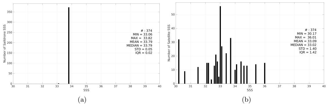
Figure 3: Histograms of SSS from Saildrone (a) and SMAP SSS L2 v5.3 - 40 km (RSS) (b) considering all match-up pairs per bins of 0.1 over the South Atlantic Ocean Pi-MEP region and for the full satellite product period.
