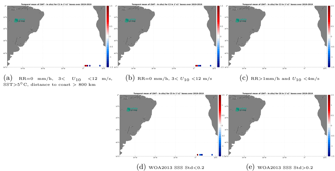
Figure 14: Temporal mean gridded over spatial boxes of size 1^\circ \times 1^\circ of \Delta SSS (SMAP SSS L2 v5.3 - 40 km (RSS) - Sailability) for 5 different subdatasets corresponding to:RR=0 mm/h, 3 < U_{10} < 12 m/s, SST >5^\circ\text{C} , distance to coast > 800 km (a), RR=0 mm/h, 3 < U_{10} < 12 m/s (b), RR >1 mm/h and U_{10} < 4 m/s (c), WOA2013 SSS Std <0.2 (d), WOA2013 SSS Std >0.2 (e).
