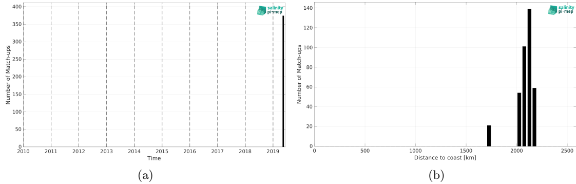
Figure 2: Number of match-ups between Saildrone and SMAP SSS L2 v5.3 - 40 km (RSS) SSS as a function of time (a) and as function of the distance to coast (b) over the South Atlantic Ocean Pi-MEP region and for the full satellite product period.
