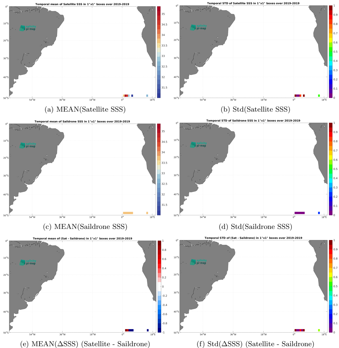
Figure 7: Temporal mean (left) and Std (right) of SSS from SMAP SSS L2 v5.3 - 40 km (RSS) (top), Saildrone (middle), and of \Delta SSS (Satellite - Saildrone). Only match-up pairs are used to generate these maps.
