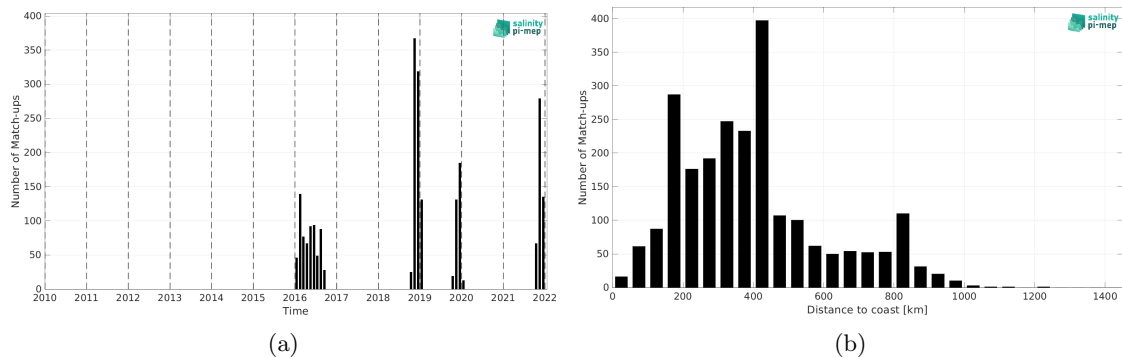
Figure 2: Number of match-ups between Marine mammals and SMAP SSS L2 v5.3 - 40 km (RSS) SSS as a function of time (a) and as function of the distance to coast (b) over the South Atlantic Ocean Pi-MEP region and for the full satellite product period.
