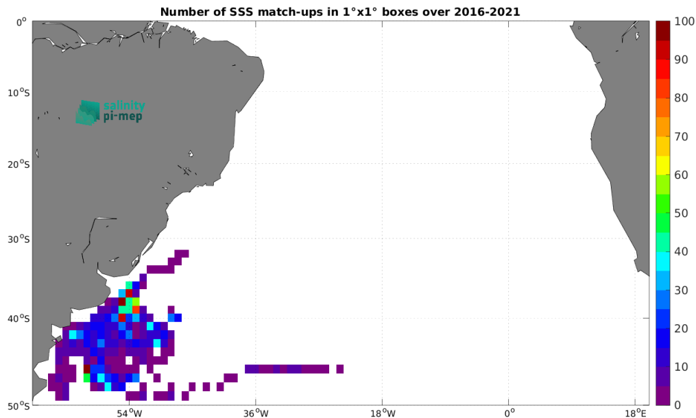
Figure 5: Number of SSS match-ups between Marine mammals SSS and the SMAP SSS L2 v5.3 - 40 km (RSS) SSS product for the South Atlantic Ocean Pi-MEP region over 1^\circ \times 1^\circ boxes and for the full satellite product period.
