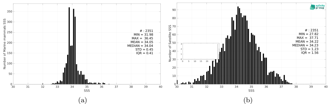
Figure 3: Histograms of SSS from Marine mammals (a) and SMAP SSS L2 v5.3 - 40 km (RSS) (b) considering all match-up pairs per bins of 0.1 over the South Atlantic Ocean Pi-MEP region and for the full satellite product period.
