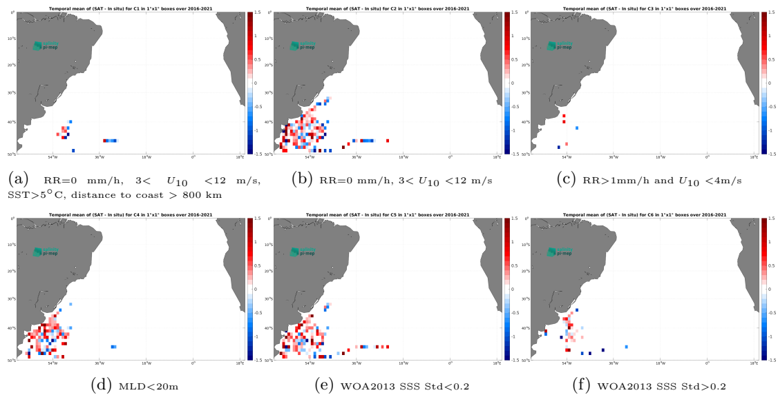
Figure 14: Temporal mean gridded over spatial boxes of size 1^\circ \times 1^\circ of \Delta SSS (SMAP SSS L2 v5.3 - 40 km (RSS) - Marine mammals) for 6 different subdatasets corresponding to:RR=0 mm/h, 3 < U_{10} < 12 m/s, SST > 5^\circ\text{C} , distance to coast > 800 km (a), RR=0 mm/h, 3 < U_{10} < 12 m/s (b), RR > 1 mm/h and U_{10} < 4 m/s (c),MLD < 20 m (d),WOA2013 SSS Std < 0.2 (e),WOA2013 SSS Std > 0.2 (f).
