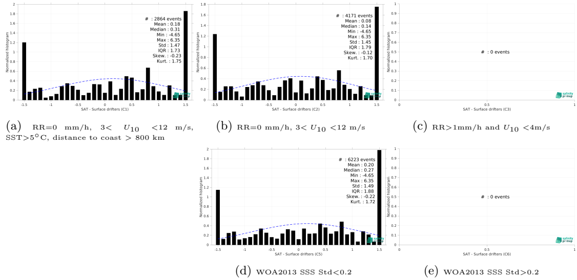
Figure 14: Normalized histogram of \Delta SSS (SMAP SSS L2 v5.3 - 40 km (RSS) - Surface drifters) for 5 different subdatasets corresponding to: RR=0 mm/h, 3 < U_{10} < 12 m/s, SST > 5°C, distance to coast > 800 km (a), RR=0 mm/h, 3 < U_{10} < 12 m/s (b), RR > 1mm/h and U_{10} < 4 m/s (c), WOA2013 SSS Std < 0.2 (d), WOA2013 SSS Std > 0.2 (e).
