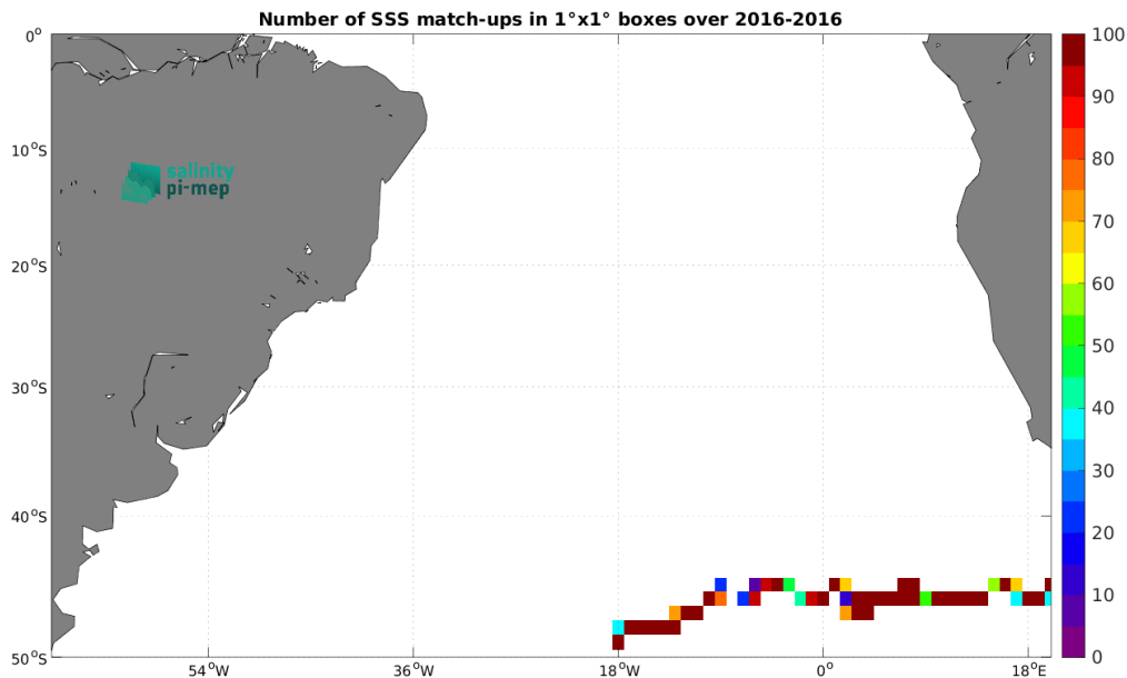
Figure 4: Number of SSS match-ups between Surface drifters SSS and the SMAP SSS L2 v5.3 - 40 km (RSS) SSS product for the South Atlantic Ocean Pi-MEP region over 1^\circ \times 1^\circ boxes and for the full satellite product period.
