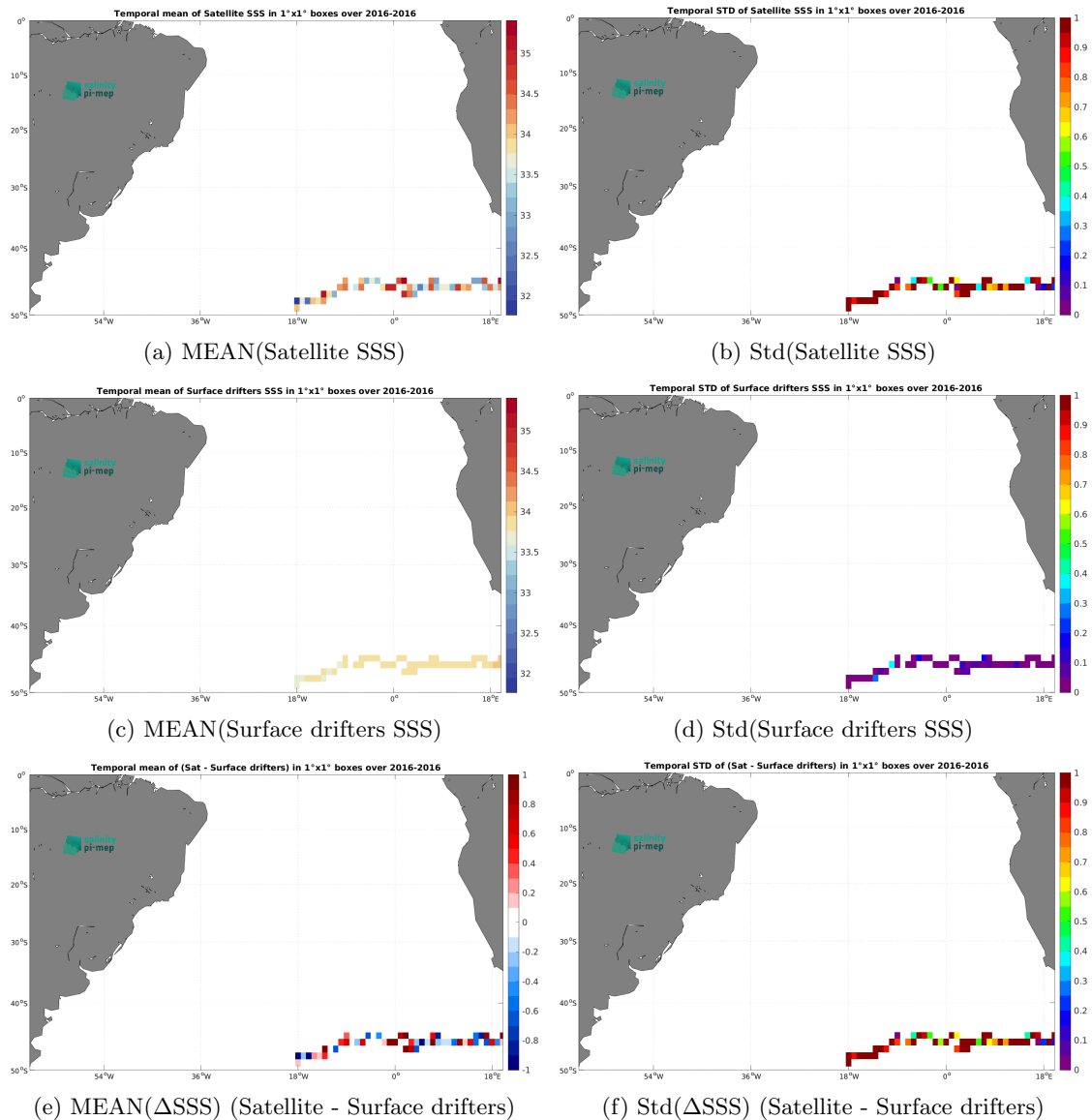
Figure 6: Temporal mean (left) and Std (right) of SSS from SMAP SSS L2 v5.3 - 40 km (RSS) (top), Surface drifters (middle), and of \Delta SSS (Satellite - Surface drifters). Only match-up pairs are used to generate these maps.
