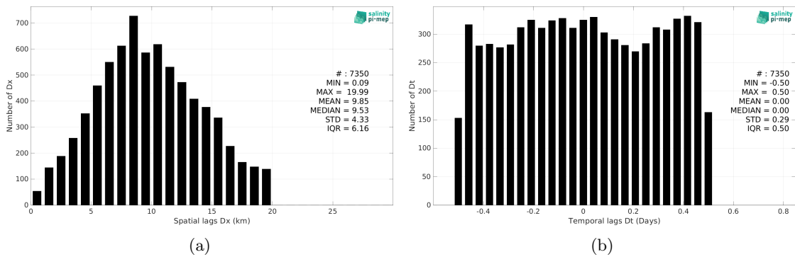
Figure 5: Histograms of the spatial (a) and temporal (b) lags between the location/time of the Surface drifters measurement and the date of the corresponding SMAP SSS L2 v5.3 - 40 km (RSS) SSS pixel.
