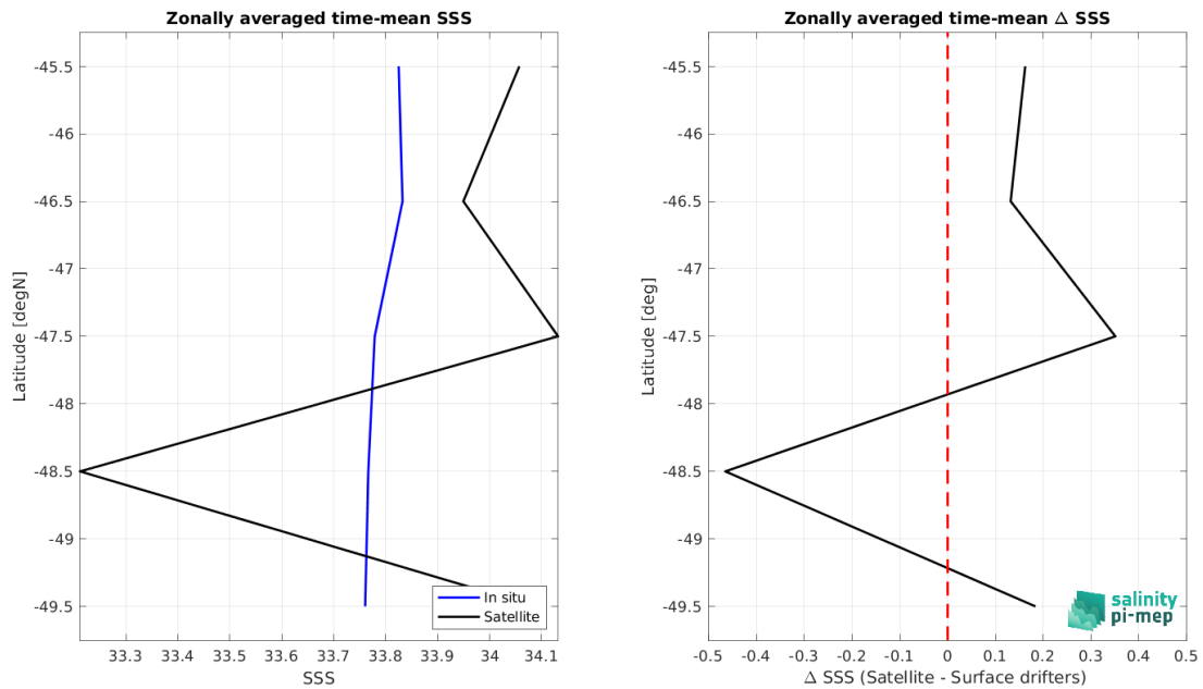
Figure 8: Left panel: Zonal mean SSS from SMAP SSS L2 v5.3 - 40 km (RSS) satellite product (black) and from Surface drifters (blue). Right panel: Zonal mean of \Delta SSS (Satellite - Surface drifters) for all the collected Pi-MEP match-up pairs estimated over the full satellite product period.
