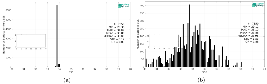
Figure 3: Histograms of SSS from Surface drifters (a) and SMAP SSS L2 v5.3 - 40 km (RSS) (b) considering all match-up pairs per bins of 0.1 over the South Atlantic Ocean Pi-MEP region and for the full satellite product period.
