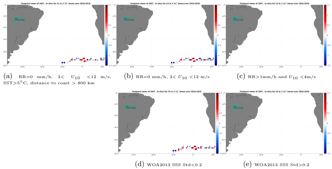
Figure 13: Temporal mean gridded over spatial boxes of size 1^\circ \times 1^\circ of \Delta SSS (SMAP SSS L2 v5.3 - 40 km (RSS) - Surface drifters) for 5 different subdatasets corresponding to:RR=0 mm/h, 3 < U_{10} < 12 m/s, SST >5^\circ\text{C} , distance to coast > 800 km (a), RR=0 mm/h, 3 < U_{10} < 12 m/s (b), RR >1 mm/h and U_{10} < 4 m/s (c), WOA2013 SSS Std <0.2 (d), WOA2013 SSS Std >0.2 (e).
