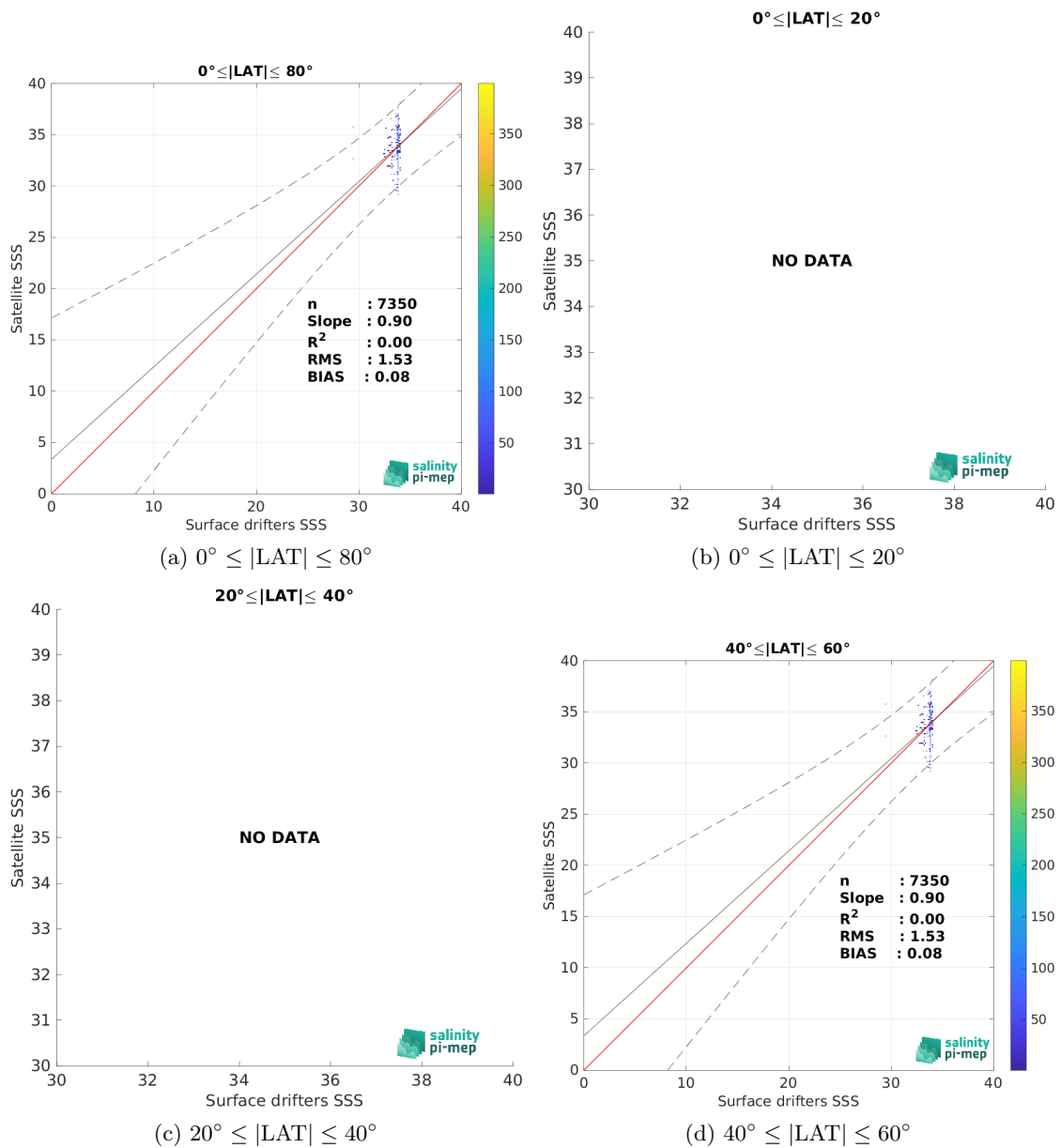
Figure 9: Contour maps of the concentration of SMAP SSS L2 v5.3 - 40 km (RSS) SSS (y-axis) versus Surface drifters SSS (x-axis) at match-up pairs for different latitude bands. For each plot, the red line shows x=y . The black thin and dashed lines indicate a linear fit through the data cloud and the \pm 95\% confidence levels, respectively. The number match-up pairs n , the slope and R^2 coefficient of the linear fit, the root mean square (RMS) and the mean bias between satellite and in situ data are indicated for each latitude band in each plots.
