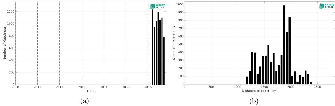
Figure 2: Number of match-ups between Surface drifters and SMAP SSS L2 v5.3 - 40 km (RSS) SSS as a function of time (a) and as function of the distance to coast (b) over the South Atlantic Ocean Pi-MEP region and for the full satellite product period.
