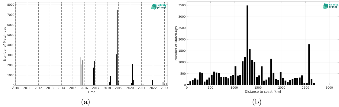
Figure 1: Number of match-ups between TSG (SAMOS) and SMAP SSS L2 v5 - 40 km (RSS) SSS as a function of time (a) and as function of the distance to coast (b) over the South Atlantic Ocean Pi-MEP region and for the full satellite product period.
