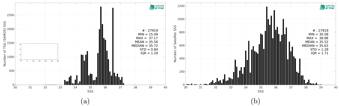
Figure 2: Histograms of SSS from TSG (SAMOS) (a) and SMAP SSS L2 v5 - 40 km (RSS) (b) considering all match-up pairs per bins of 0.1 over the South Atlantic Ocean Pi-MEP region and for the full satellite product period.
