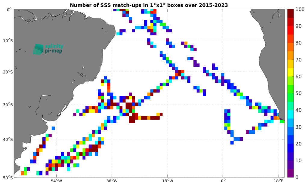
Figure 4: Number of SSS match-ups between TSG (SAMOS) SSS and the SMAP SSS L2 v5 - 40 km (RSS) SSS product for the South Atlantic Ocean Pi-MEP region over 1^\circ \times 1^\circ boxes and for the full satellite product period.
