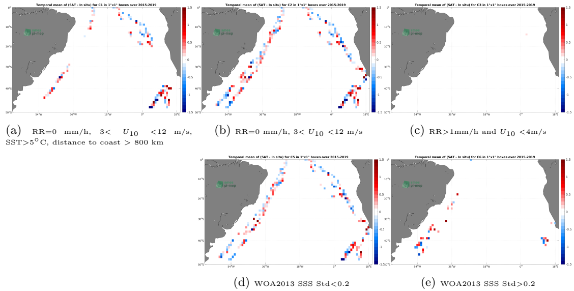
Figure 12: Temporal mean gridded over spatial boxes of size 1^\circ \times 1^\circ of \Delta\text{SSS} (SMAP SSS L2 v5 - 40 km (RSS) - TSG (Polarstern)) for 5 different subdatasets corresponding to:RR=0 mm/h, 3 < U_{10} < 12 m/s, SST >5^\circ\text{C} , distance to coast > 800 km (a), RR=0 mm/h, 3 < U_{10} < 12 m/s (b), RR >1 mm/h and U_{10} < 4 m/s (c), WOA2013 SSS Std <0.2 (d), WOA2013 SSS Std >0.2 (e).
