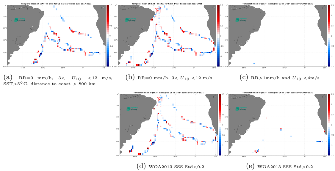
Figure 12: Temporal mean gridded over spatial boxes of size 1^\circ \times 1^\circ of \Delta\text{SSS} (SMAP SSS L2 v5 - 40 km (RSS) - TSG (GOSUD-Sailing-ship)) for 5 different subdatasets corresponding to:RR=0 mm/h, 3 < U_{10} < 12 m/s, SST>5°C, distance to coast > 800 km (a), RR=0 mm/h, 3 < U_{10} < 12 m/s (b), RR>1mm/h and U_{10} < 4 m/s (c), WOA2013 SSS Std<0.2 (d), WOA2013 SSS Std>0.2 (e).
