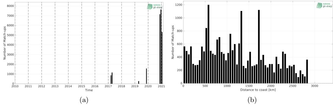
Figure 1: Number of match-ups between TSG (GOSUD-Sailing-ship) and SMAP SSS L2 v5 - 40 km (RSS) SSS as a function of time (a) and as function of the distance to coast (b) over the South Atlantic Ocean Pi-MEP region and for the full satellite product period.
