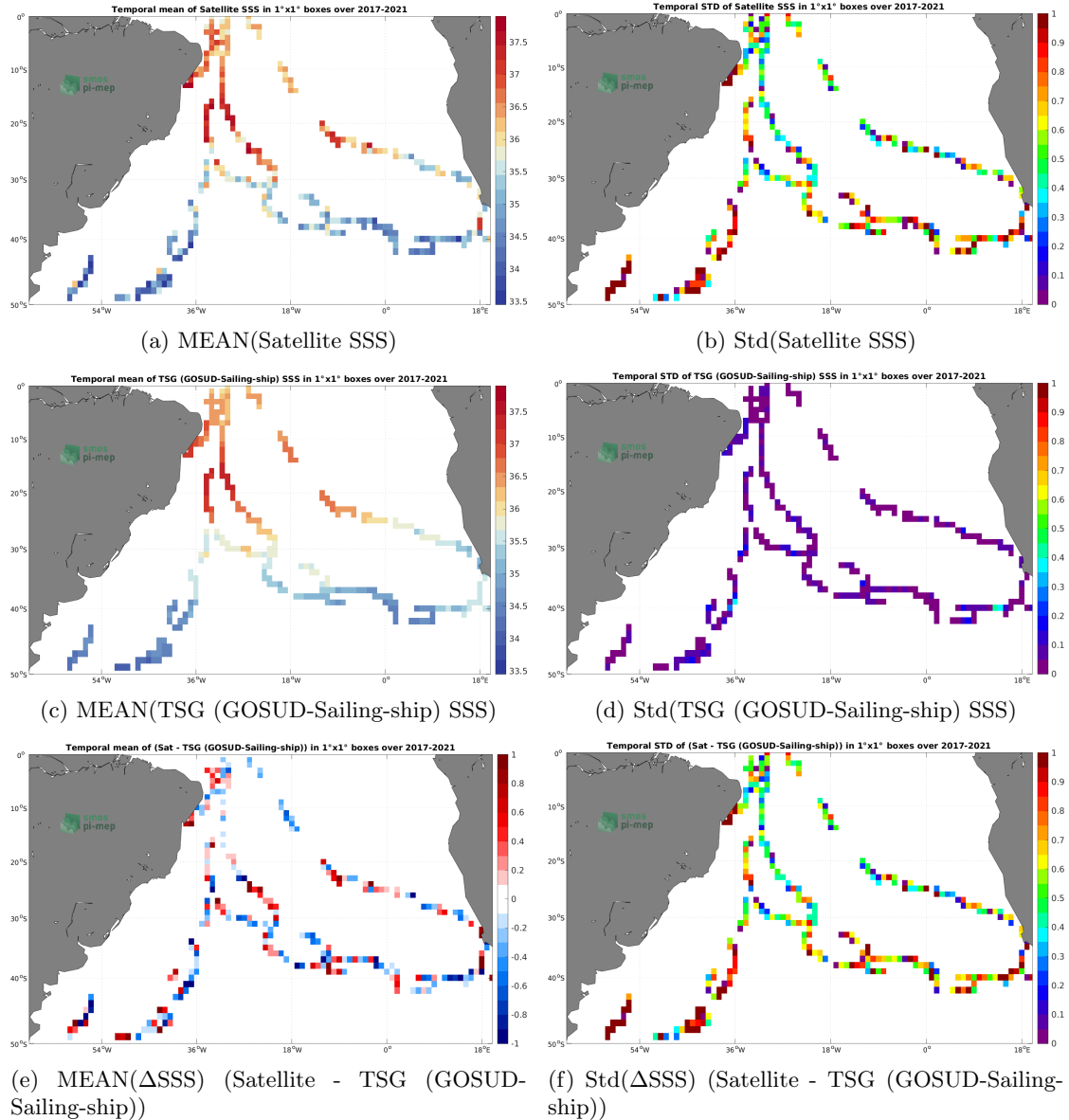
Figure 6: Temporal mean (left) and Std (right) of SSS from SMAP SSS L2 v5 - 40 km (RSS) (top), TSG (GOSUD-Sailing-ship) (middle), and of \Delta SSS (Satellite - TSG (GOSUD-Sailing-ship)). Only match-up pairs are used to generate these maps.
