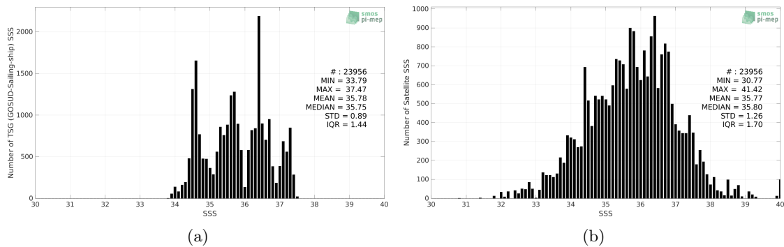
Figure 2: Histograms of SSS from TSG (GOSUD-Sailing-ship) (a) and SMAP SSS L2 v5 - 40 km (RSS) (b) considering all match-up pairs per bins of 0.1 over the South Atlantic Ocean Pi-MEP region and for the full satellite product period.
