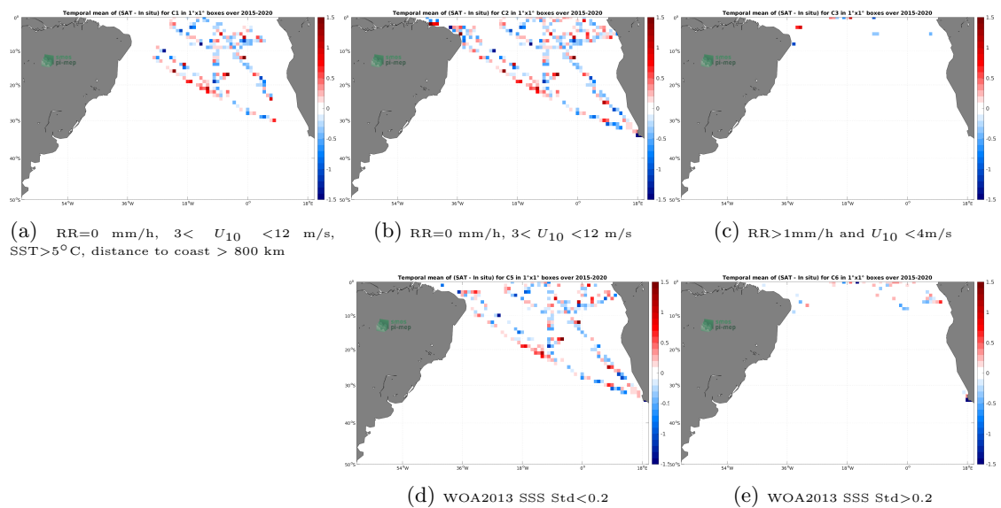
Figure 12: Temporal mean gridded over spatial boxes of size 1^\circ \times 1^\circ of \Delta SSS (SMAP SSS L2 v5 - 40 km (RSS) - TSG (GOSUD-Research-vessel)) for 5 different subdatasets corresponding to:RR=0 mm/h, 3 < U_{10} < 12 m/s, SST > 5°C, distance to coast > 800 km (a), RR=0 mm/h, 3 < U_{10} < 12 m/s (b), RR > 1mm/h and U_{10} < 4 m/s (c), WOA2013 SSS Std < 0.2 (d), WOA2013 SSS Std > 0.2 (e).
