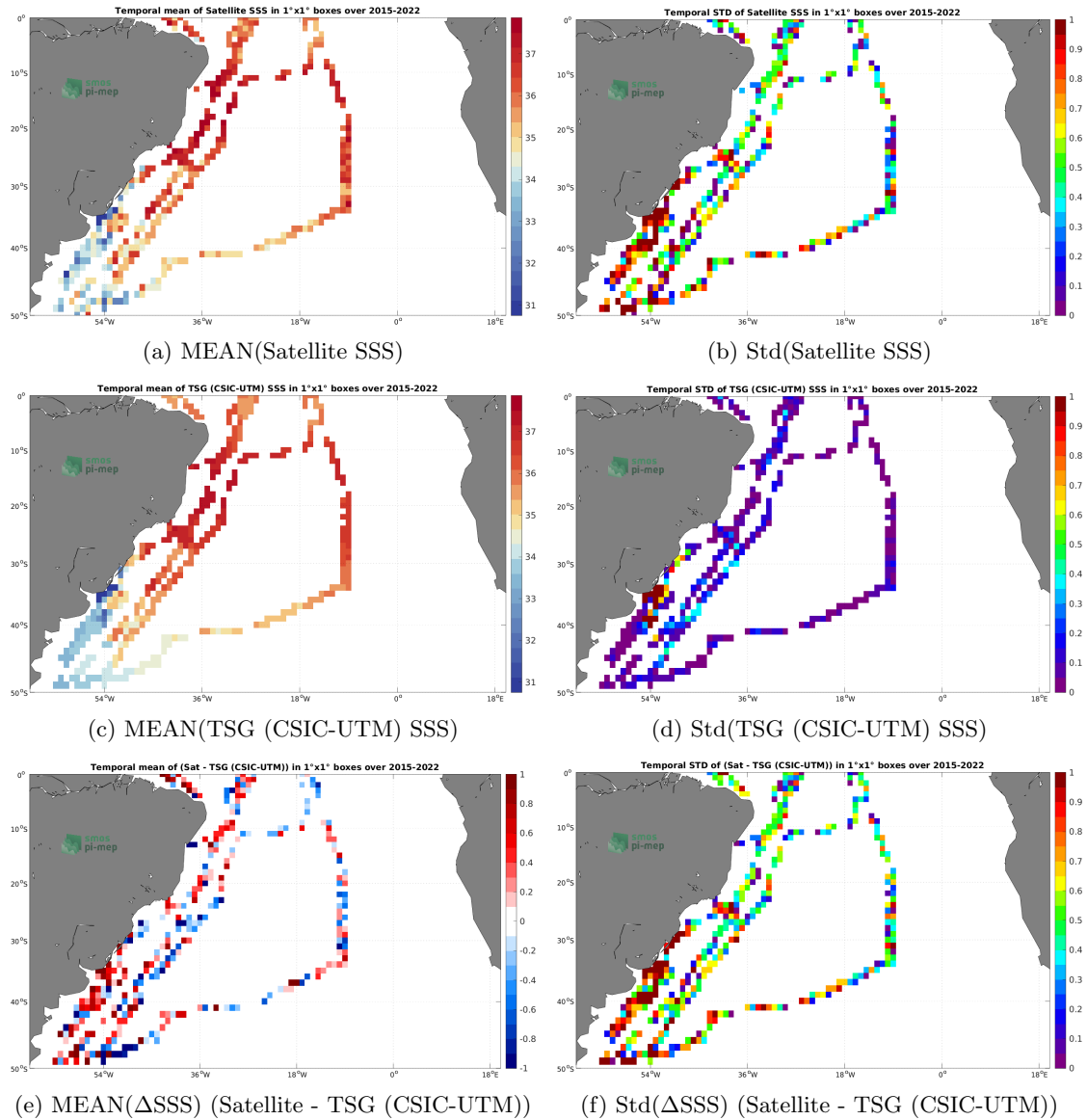
Figure 6: Temporal mean (left) and Std (right) of SSS from SMAP SSS L2 v5 - 40 km (RSS) (top), TSG (CSIC-UTM) (middle), and of \Delta SSS (Satellite - TSG (CSIC-UTM)). Only match-up pairs are used to generate these maps.
