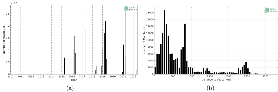
Figure 1: Number of match-ups between TSG (CSIC-UTM) and SMAP SSS L2 v5 - 40 km (RSS) SSS as a function of time (a) and as function of the distance to coast (b) over the South Atlantic Ocean Pi-MEP region and for the full satellite product period.
