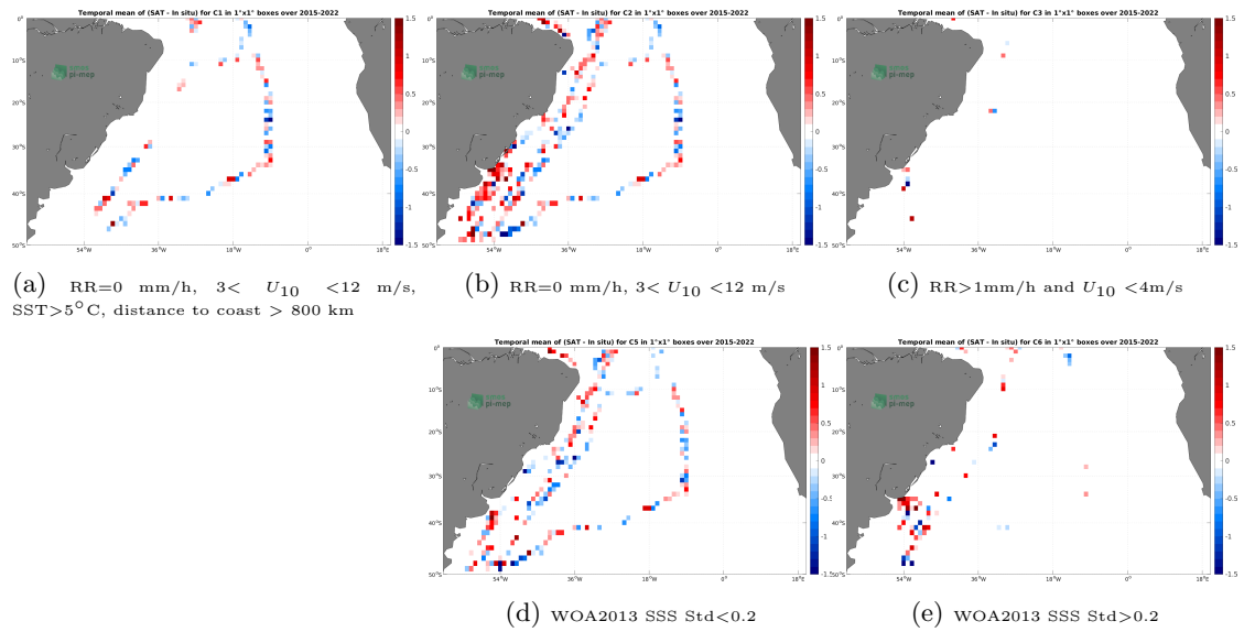
Figure 12: Temporal mean gridded over spatial boxes of size 1^\circ \times 1^\circ of \Delta SSS (SMAP SSS L2 v5 - 40 km (RSS) - TSG (CSIC-UTM)) for 5 different subdatasets corresponding to:RR=0 mm/h, 3 < U_{10} < 12 m/s, SST >5^\circ\text{C} , distance to coast > 800 km (a), RR=0 mm/h, 3 < U_{10} < 12 m/s (b), RR >1 mm/h and U_{10} < 4 m/s (c), WOA2013 SSS Std <0.2 (d), WOA2013 SSS Std >0.2 (e).
