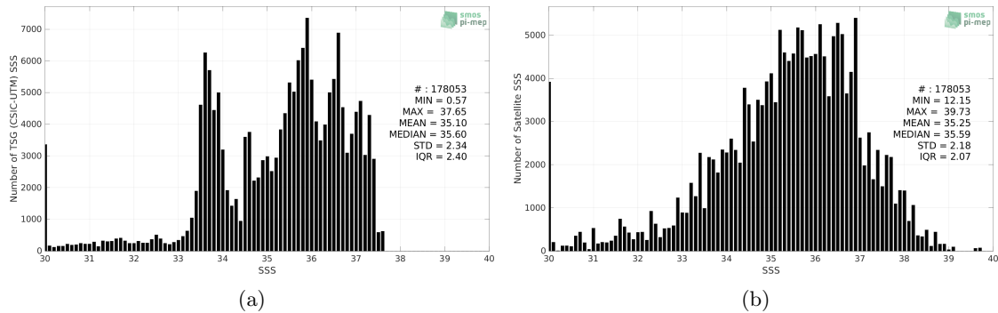
Figure 2: Histograms of SSS from TSG (CSIC-UTM) (a) and SMAP SSS L2 v5 - 40 km (RSS) (b) considering all match-up pairs per bins of 0.1 over the South Atlantic Ocean Pi-MEP region and for the full satellite product period.
