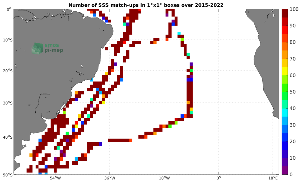
Figure 4: Number of SSS match-ups between TSG (CSIC-UTM) SSS and the SMAP SSS L2 v5 - 40 km (RSS) SSS product for the South Atlantic Ocean Pi-MEP region over 1^\circ \times 1^\circ boxes and for the full satellite product period.
