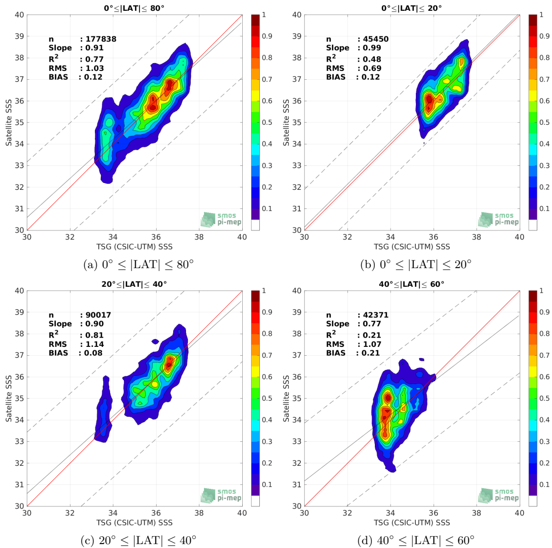
Figure 9: Contour maps of the concentration of SMAP SSS L2 v5 - 40 km (RSS) SSS (y-axis) versus TSG (CSIC-UTM) SSS (x-axis) at match-up pairs for different latitude bands. For each plot, the red line shows x=y . The black thin and dashed lines indicate a linear fit through the data cloud and the \pm 95\% confidence levels, respectively. The number match-up pairs n , the slope and R^2 coefficient of the linear fit, the root mean square (RMS) and the mean bias between satellite and in situ data are indicated for each latitude band in each plots.
