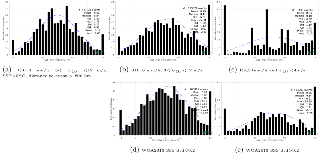
Figure 13: Normalized histogram of \Delta SSS (SMAP SSS L2 v5 - 40 km (RSS) - TSG (CSIC-UTM)) for 5 different subdatasets corresponding to: RR=0 mm/h, 3 < U_{10} < 12 m/s, SST > 5°C, distance to coast > 800 km (a), RR=0 mm/h, 3 < U_{10} < 12 m/s (b), RR > 1mm/h and U_{10} < 4 m/s (c), WOA2013 SSS Std < 0.2 (d), WOA2013 SSS Std > 0.2 (e).
