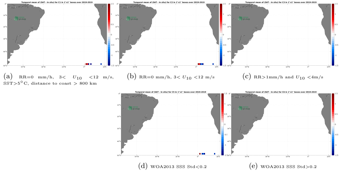
Figure 12: Temporal mean gridded over spatial boxes of size 1^{\circ}\times 1^{\circ} of \Delta\text{SSS} (SMAP SSS L2 v5 - 40 km (RSS) - Sairdron) for 5 different subdatasets corresponding to:RR=0 mm/h, 3 < U_{10} < 12 m/s, SST >5^{\circ}\text{C} , distance to coast > 800 km (a), RR=0 mm/h, 3 < U_{10} < 12 m/s (b), RR >1 mm/h and U_{10} < 4 m/s (c), WOA2013 SSS Std <0.2 (d), WOA2013 SSS Std >0.2 (e).
