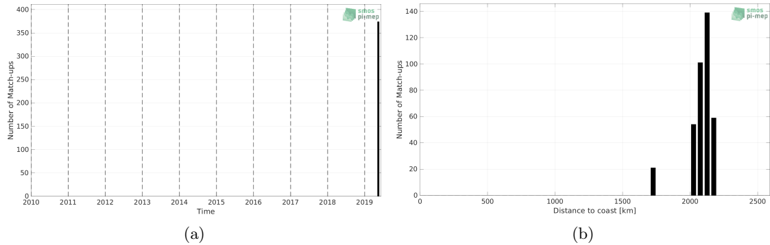
Figure 1: Number of match-ups between Saildrone and SMAP SSS L2 v5 - 40 km (RSS) SSS as a function of time (a) and as function of the distance to coast (b) over the South Atlantic Ocean Pi-MEP region and for the full satellite product period.
