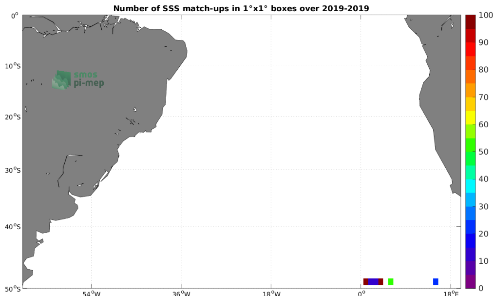
Figure 4: Number of SSS match-ups between Saildrone SSS and the SMAP SSS L2 v5 - 40 km (RSS) SSS product for the South Atlantic Ocean Pi-MEP region over 1^\circ \times 1^\circ boxes and for the full satellite product period.
