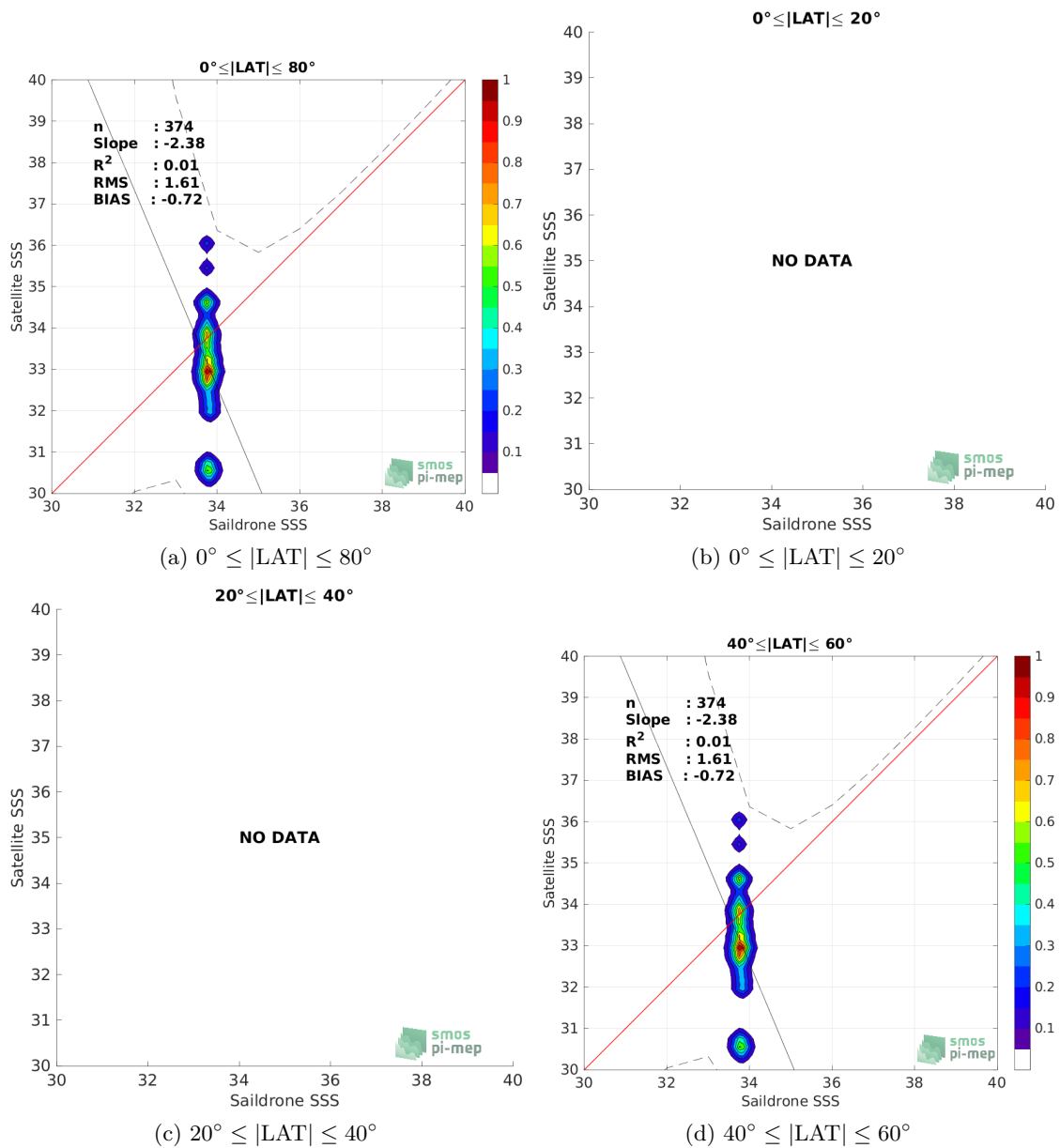
Figure 9: Contour maps of the concentration of SMAP SSS L2 v5 - 40 km (RSS) SSS (y-axis) versus Saildrone SSS (x-axis) at match-up pairs for different latitude bands. For each plot, the red line shows x=y . The black thin and dashed lines indicate a linear fit through the data cloud and the \pm 95\% confidence levels, respectively. The number match-up pairs n , the slope and R^2 coefficient of the linear fit, the root mean square (RMS) and the mean bias between satellite and in situ data are indicated for each latitude band in each plots.
