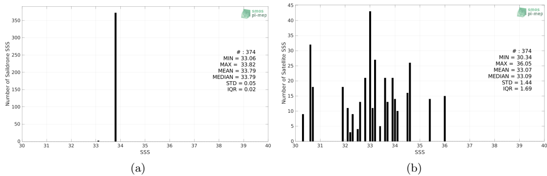
Figure 2: Histograms of SSS from Saildrone (a) and SMAP SSS L2 v5 - 40 km (RSS) (b) considering all match-up pairs per bins of 0.1 over the South Atlantic Ocean Pi-MEP region and for the full satellite product period.
