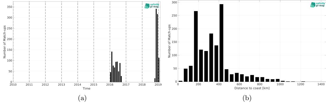
Figure 1: Number of match-ups between Marine mammals and SMAP SSS L2 v5 - 40 km (RSS) SSS as a function of time (a) and as function of the distance to coast (b) over the South Atlantic Ocean Pi-MEP region and for the full satellite product period.
