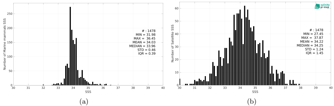
Figure 2: Histograms of SSS from Marine mammals (a) and SMAP SSS L2 v5 - 40 km (RSS) (b) considering all match-up pairs per bins of 0.1 over the South Atlantic Ocean Pi-MEP region and for the full satellite product period.
