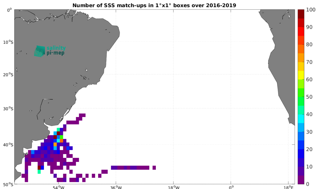
Figure 4: Number of SSS match-ups between Marine mammals SSS and the SMAP SSS L2 v5 - 40 km (RSS) SSS product for the South Atlantic Ocean Pi-MEP region over 1^\circ \times 1^\circ boxes and for the full satellite product period.
