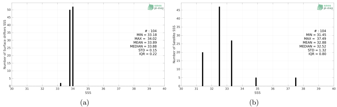
Figure 2: Histograms of SSS from Surface drifters (a) and SMAP SSS L2 v5 - 40 km (RSS) (b) considering all match-up pairs per bins of 0.1 over the South Atlantic Ocean Pi-MEP region and for the full satellite product period.
