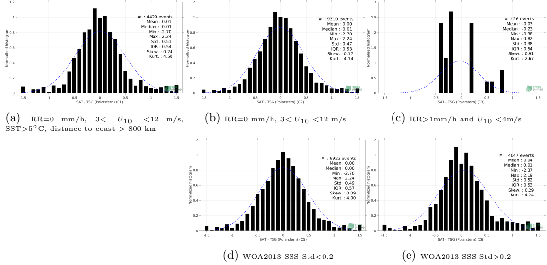
Figure 13: Normalized histogram of \Delta\text{SSS} (SMAP SSS L2 v4 (RSS) - TSG (Polarstern)) for 5 different subdatasets corresponding to: RR=0 mm/h, 3 < U_{10} < 12 m/s, SST>5°C, distance to coast > 800 km (a), RR=0 mm/h, 3 < U_{10} < 12 m/s (b), RR>1mm/h and U_{10} < 4 m/s (c), WOA2013 SSS Std<0.2 (d), WOA2013 SSS Std>0.2 (e).
