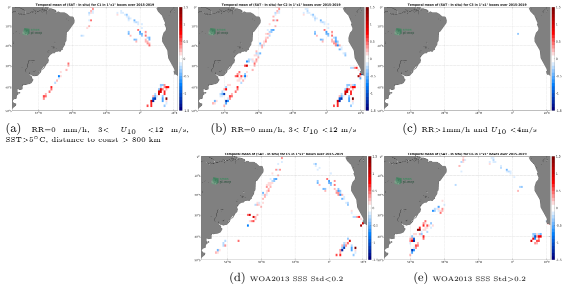
Figure 12: Temporal mean gridded over spatial boxes of size 1^\circ \times 1^\circ of \Delta SSS (SMAP SSS L2 v4 (RSS) - TSG (Polarstern)) for 5 different subdatasets corresponding to: RR=0 mm/h, 3 < U_{10} < 12 m/s, SST > 5^\circ C , distance to coast > 800 km (a), RR=0 mm/h, 3 < U_{10} < 12 m/s (b), RR > 1 mm/h and U_{10} < 4 m/s (c), WOA2013 SSS Std < 0.2 (d), WOA2013 SSS Std > 0.2 (e).
