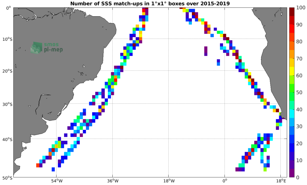
Figure 4: Number of SSS match-ups between TSG (Polarstern) SSS and the SMAP SSS L2 v4 (RSS) SSS product for the South Atlantic Ocean Pi-MEP region over 1^\circ \times 1^\circ boxes and for the full satellite product period.
