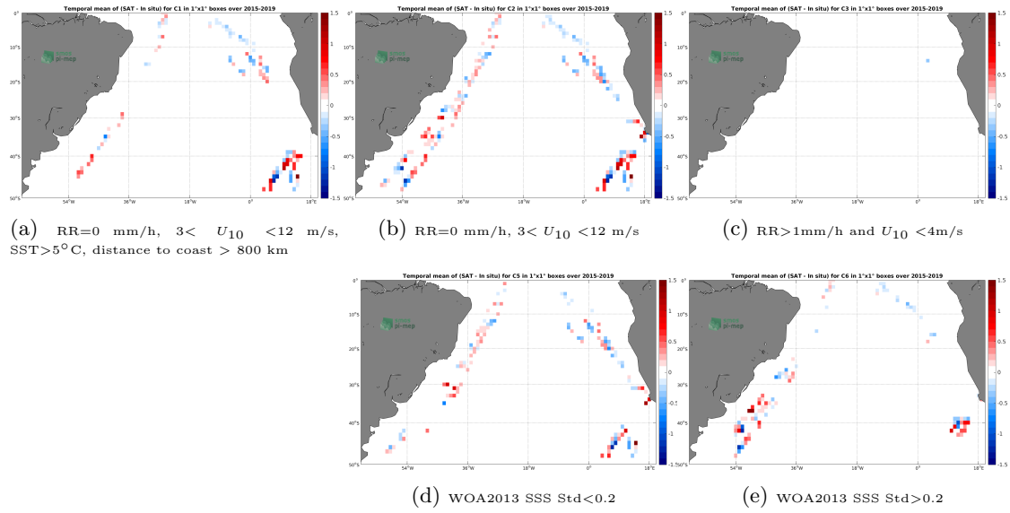
Figure 12: Temporal mean gridded over spatial boxes of size 1^\circ \times 1^\circ of \Delta SSS (SMAP SSS L2 v4 (RSS) - TSG (Polarstern)) for 5 different subdatasets corresponding to: RR=0 mm/h, 3 < U_{10} < 12 m/s, SST > 5^\circ C , distance to coast > 800 km (a), RR=0 mm/h, 3 < U_{10} < 12 m/s (b), RR > 1 mm/h and U_{10} < 4 m/s (c), WOA2013 SSS Std < 0.2 (d), WOA2013 SSS Std > 0.2 (e).
