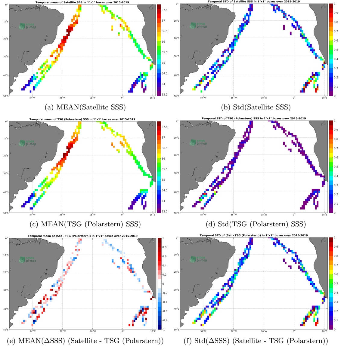
Figure 6: Temporal mean (left) and Std (right) of SSS from SMAP SSS L2 v4 (RSS) (top), TSG (Polarstern) (middle), and of \Delta SSS (Satellite - TSG (Polarstern)). Only match-up pairs are used to generate these maps.
