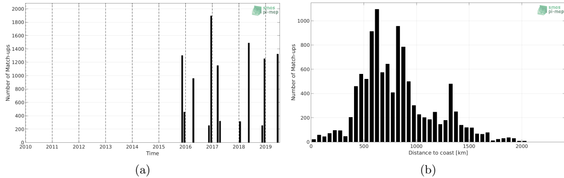
Figure 1: Number of match-ups between TSG (Polarstern) and SMAP SSS L2 v4 (RSS) SSS as a function of time (a) and as function of the distance to coast (b) over the South Atlantic Ocean Pi-MEP region and for the full satellite product period.
