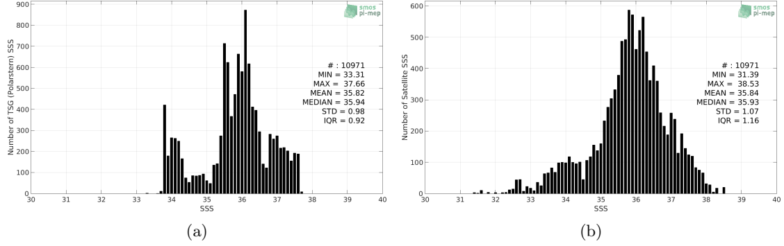
Figure 2: Histograms of SSS from TSG (Polarstern) (a) and SMAP SSS L2 v4 (RSS) (b) considering all match-up pairs per bins of 0.1 over the South Atlantic Ocean Pi-MEP region and for the full satellite product period.
