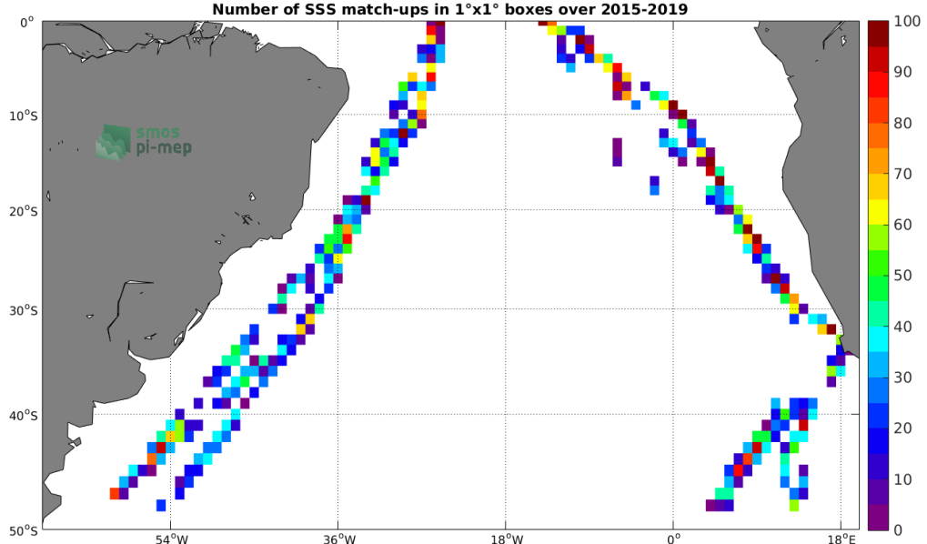
Figure 4: Number of SSS match-ups between TSG (Polarstern) SSS and the SMAP SSS L2 v4 (RSS) SSS product for the South Atlantic Ocean Pi-MEP region over 1^\circ \times 1^\circ boxes and for the full satellite product period.
