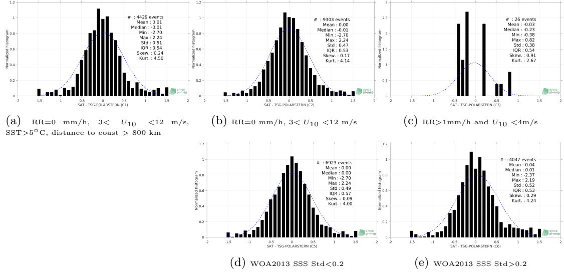
Figure 13: Normalized histogram of \Delta\text{SSS} (SMAP-L2-RSS-V4 - TSG-POLARSTERN) for 5 different subdatasets corresponding to: RR=0 mm/h, 3 < U_{10} < 12 m/s, SST > 5^{\circ}\text{C} , distance to coast > 800 km (a), RR=0 mm/h, 3 < U_{10} < 12 m/s (b), RR > 1 mm/h and U_{10} < 4 m/s (c), WOA2013 SSS Std < 0.2 (d), WOA2013 SSS Std > 0.2 (e).
