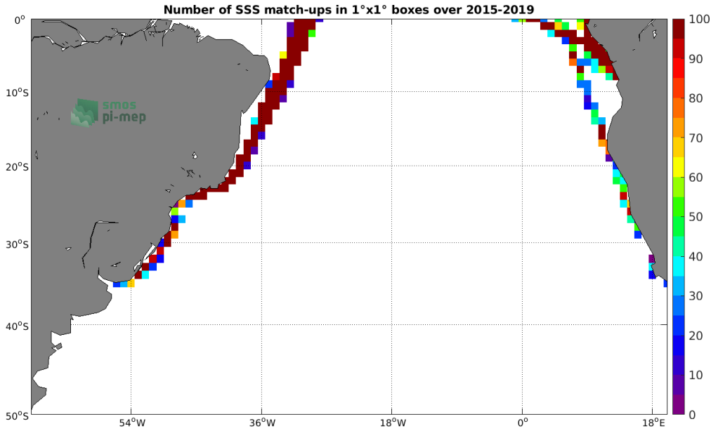
Figure 4: Number of SSS match-ups between TSG (LEGOS-DM) SSS and the SMAP SSS L2 v4 (RSS) SSS product for the South Atlantic Ocean Pi-MEP region over 1^\circ \times 1^\circ boxes and for the full satellite product period.
