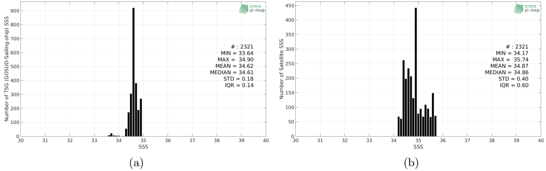
Figure 2: Histograms of SSS from TSG (GOSUD-Sailing-ship) (a) and SMAP SSS L2 v4 (RSS) (b) considering all match-up pairs per bins of 0.1 over the South Atlantic Ocean Pi-MEP region and for the full satellite product period.
