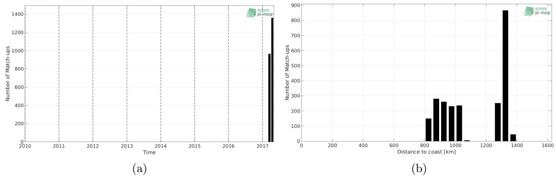
Figure 1: Number of match-ups between TSG (GOSUD-Sailing-ship) and SMAP SSS L2 v4 (RSS) SSS as a function of time (a) and as function of the distance to coast (b) over the South Atlantic Ocean Pi-MEP region and for the full satellite product period.
