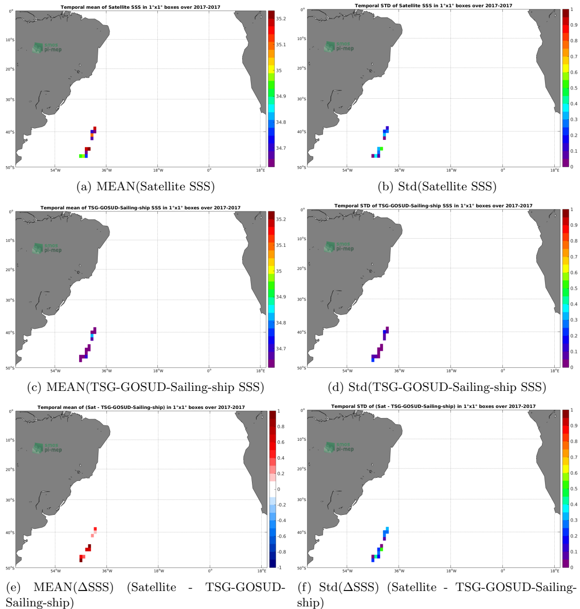
Figure 6: Temporal mean (left) and Std (right) of SSS from SMAP-L2-RSS-V4 (top), TSG-GOSUD-Sailing-ship (middle), and of \Delta SSS (Satellite - TSG-GOSUD-Sailing-ship). Only match-up pairs are used to generate these maps.
