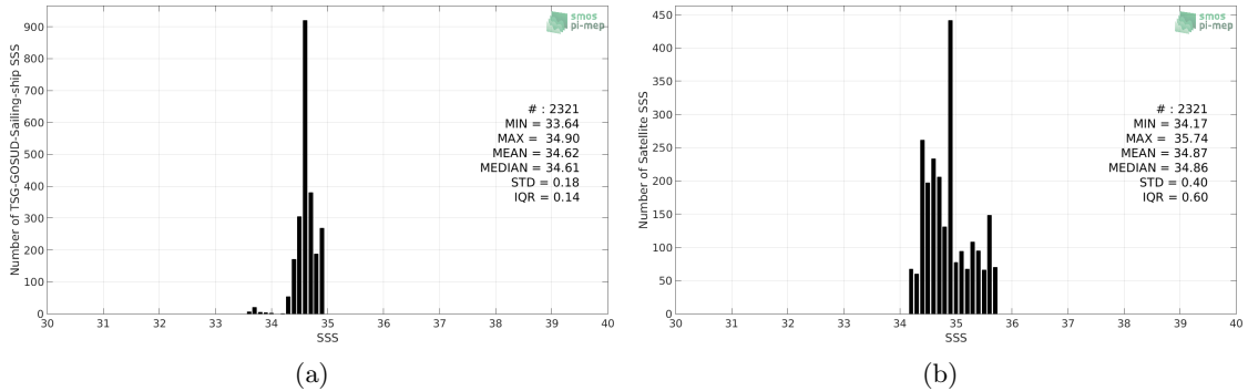
Figure 2: Histograms of SSS from TSG-GOSUD-Sailing-ship (a) and SMAP-L2-RSS-V4 (b) considering all match-up pairs per bins of 0.1 over the South Atlantic Ocean Pi-MEP region and for the full satellite product period.
