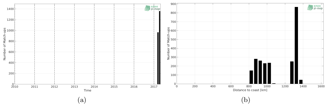
Figure 1: Number of match-ups between TSG-GOSUD-Sailing-ship and SMAP-L2-RSS-V4 SSS as a function of time (a) and as function of the distance to coast (b) over the South Atlantic Ocean Pi-MEP region and for the full satellite product period.
