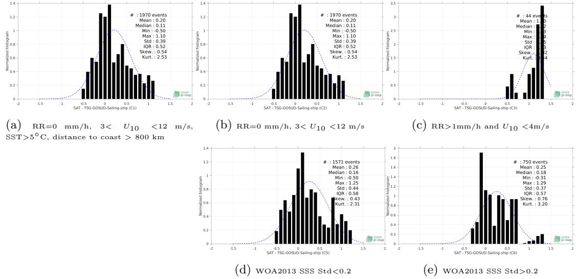
Figure 13: Normalized histogram of \Delta SSS (SMAP-L2-RSS-V4 - TSG-GOSUD-Sailing-ship) for 5 different subdatasets corresponding to: RR=0 mm/h, 3 < U_{10} < 12 m/s, SST > 5^\circ\text{C} , distance to coast > 800 km (a), RR=0 mm/h, 3 < U_{10} < 12 m/s (b), RR > 1\text{mm/h} and U_{10} < 4\text{m/s} (c), WOA2013 SSS Std < 0.2 (d), WOA2013 SSS Std > 0.2 (e).
