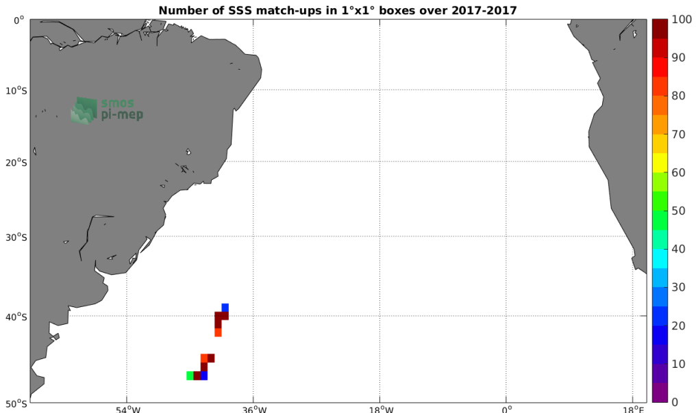
Figure 4: Number of SSS match-ups between TSG-GOSUD-Sailing-ship SSS and the SMAP-L2-RSS-V4 SSS product for the South Atlantic Ocean Pi-MEP region over 1°x1° boxes and for the full satellite product period.
