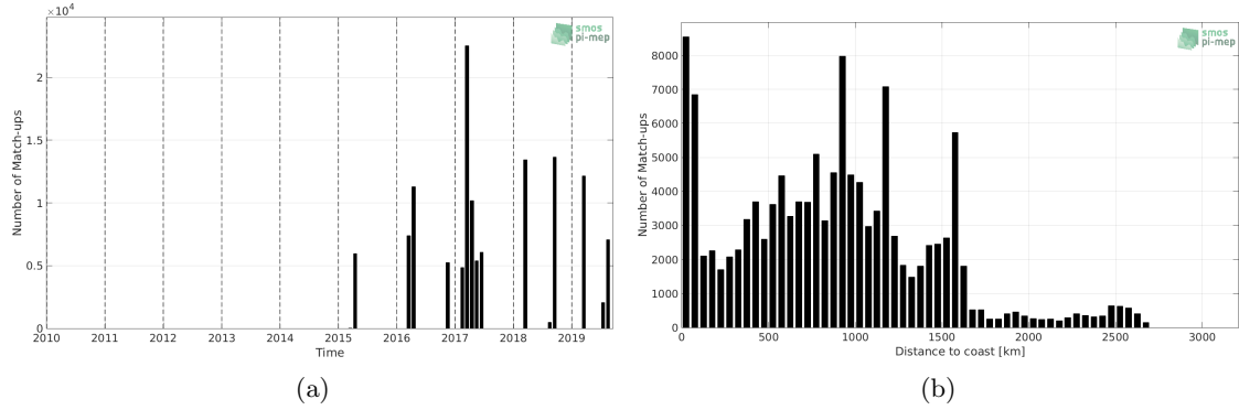
Figure 1: Number of match-ups between TSG (GOSUD-Research-vessel) and SMAP SSS L2 v4 (RSS) SSS as a function of time (a) and as function of the distance to coast (b) over the South Atlantic Ocean Pi-MEP region and for the full satellite product period.
