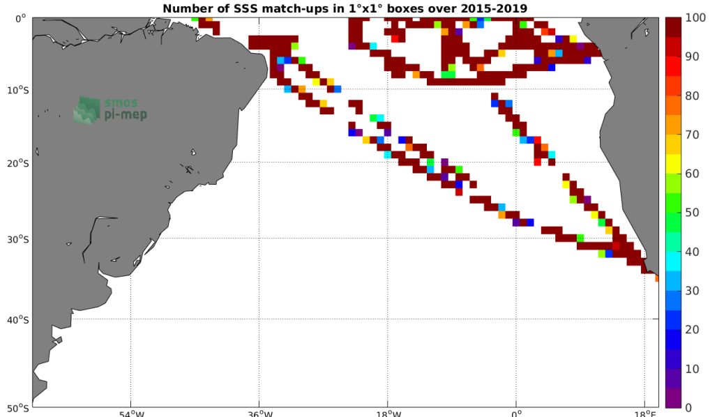
Figure 4: Number of SSS match-ups between TSG (GOSUD-Research-vessel) SSS and the SMAP SSS L2 v4 (RSS) SSS product for the South Atlantic Ocean Pi-MEP region over 1^\circ \times 1^\circ boxes and for the full satellite product period.
