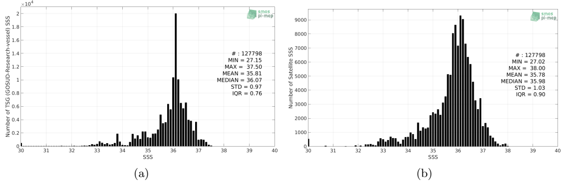
Figure 2: Histograms of SSS from TSG (GOSUD-Research-vessel) (a) and SMAP SSS L2 v4 (RSS) (b) considering all match-up pairs per bins of 0.1 over the South Atlantic Ocean Pi-MEP region and for the full satellite product period.
