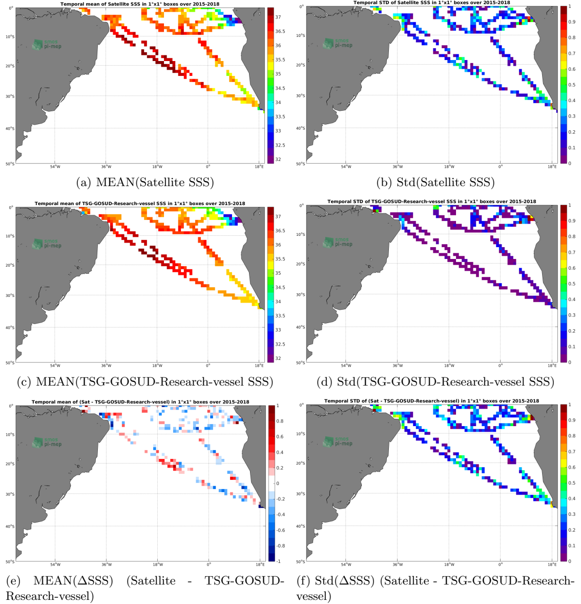
Figure 6: Temporal mean (left) and Std (right) of SSS from SMAP-L2-RSS-V4 (top), TSG-GOSUD-Research-vessel (middle), and of \Delta SSS (Satellite - TSG-GOSUD-Research-vessel). Only match-up pairs are used to generate these maps.
