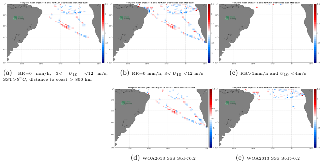
Figure 12: Temporal mean gridded over spatial boxes of size 1^\circ \times 1^\circ of \Delta SSS (SMAP-L2-RSS-V4 - TSG-GOSUD-Research-vessel) for 5 different subdatasets corresponding to: RR=0 mm/h, 3 < U_{10} < 12 m/s, SST > 5^\circ C , distance to coast > 800 km (a), RR=0 mm/h, 3 < U_{10} < 12 m/s (b), RR > 1 mm/h and U_{10} < 4 m/s (c), WOA2013 SSS Std < 0.2 (d), WOA2013 SSS Std > 0.2 (e).
