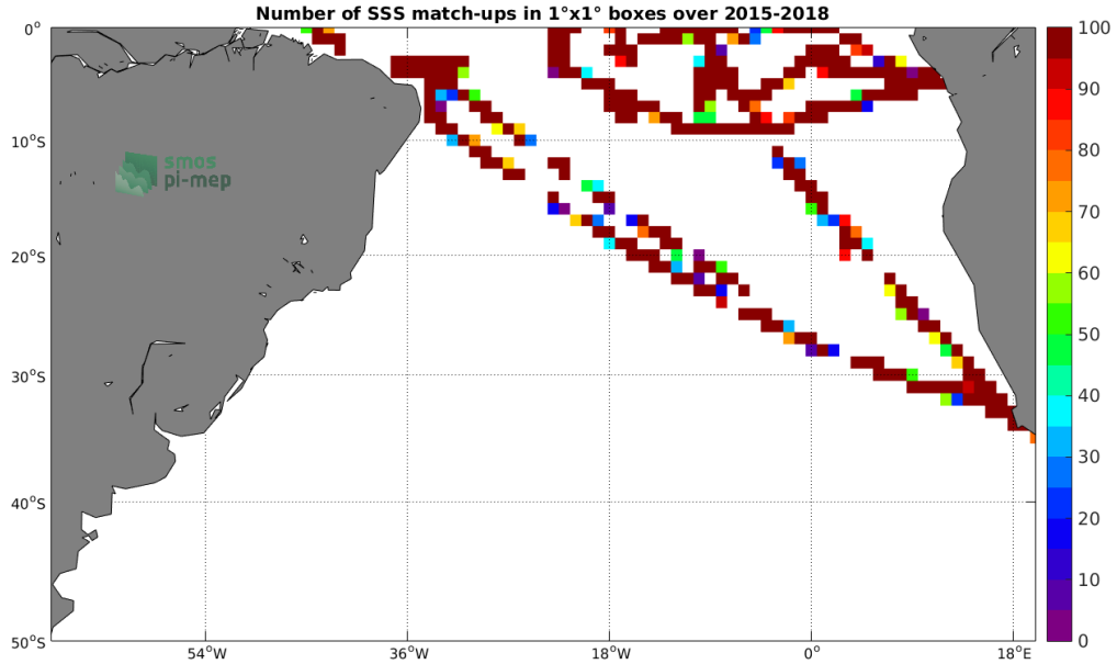
Figure 4: Number of SSS match-ups between TSG-GOSUD-Research-vessel SSS and the SMAP-L2-RSS-V4 SSS product for the South Atlantic Ocean Pi-MEP region over 1^\circ \times 1^\circ boxes and for the full satellite product period.
