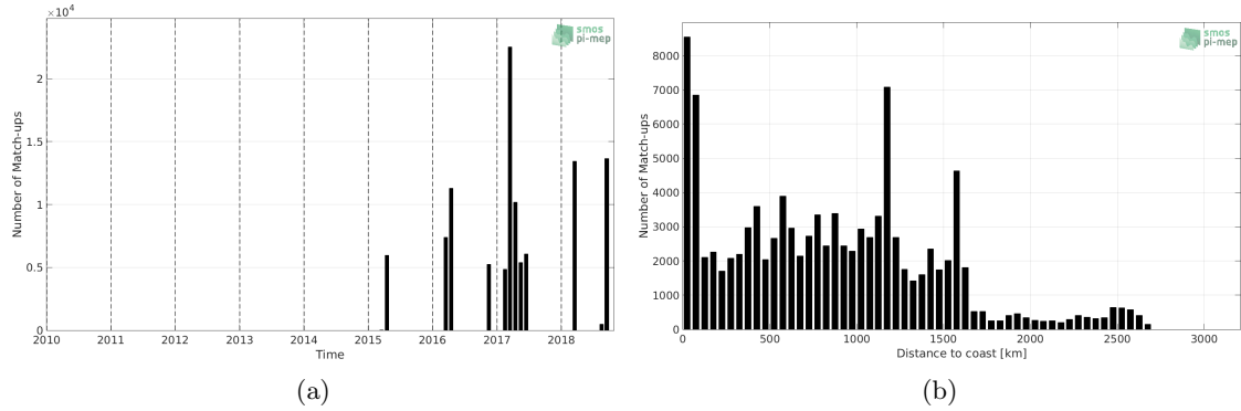
Figure 1: Number of match-ups between TSG-GOSUD-Research-vessel and SMAP-L2-RSS-V4 SSS as a function of time (a) and as function of the distance to coast (b) over the South Atlantic Ocean Pi-MEP region and for the full satellite product period.
