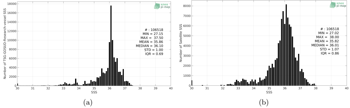
Figure 2: Histograms of SSS from TSG-GOSUD-Research-vessel (a) and SMAP-L2-RSS-V4 (b) considering all match-up pairs per bins of 0.1 over the South Atlantic Ocean Pi-MEP region and for the full satellite product period.
