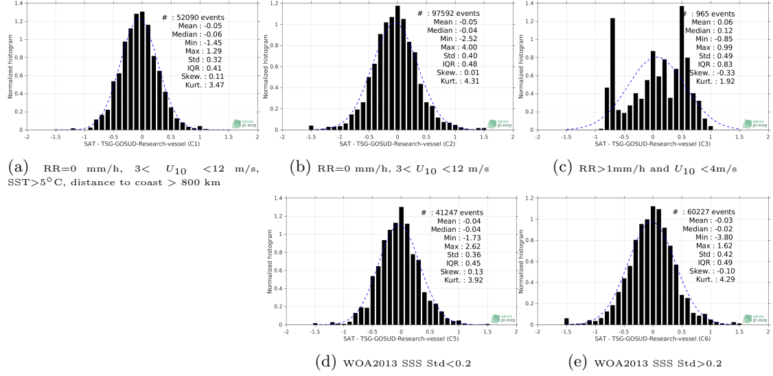
Figure 13: Normalized histogram of \Delta SSS (SMAP-L2-RSS-V4 - TSG-GOSUD-Research-vessel) for 5 different subdatasets corresponding to: RR=0 mm/h, 3 < U_{10} < 12 m/s, SST>5°C, distance to coast > 800 km (a), RR=0 mm/h, 3 < U_{10} < 12 m/s (b), RR>1mm/h and U_{10} < 4 m/s (c), WOA2013 SSS Std<0.2 (d), WOA2013 SSS Std>0.2 (e).
