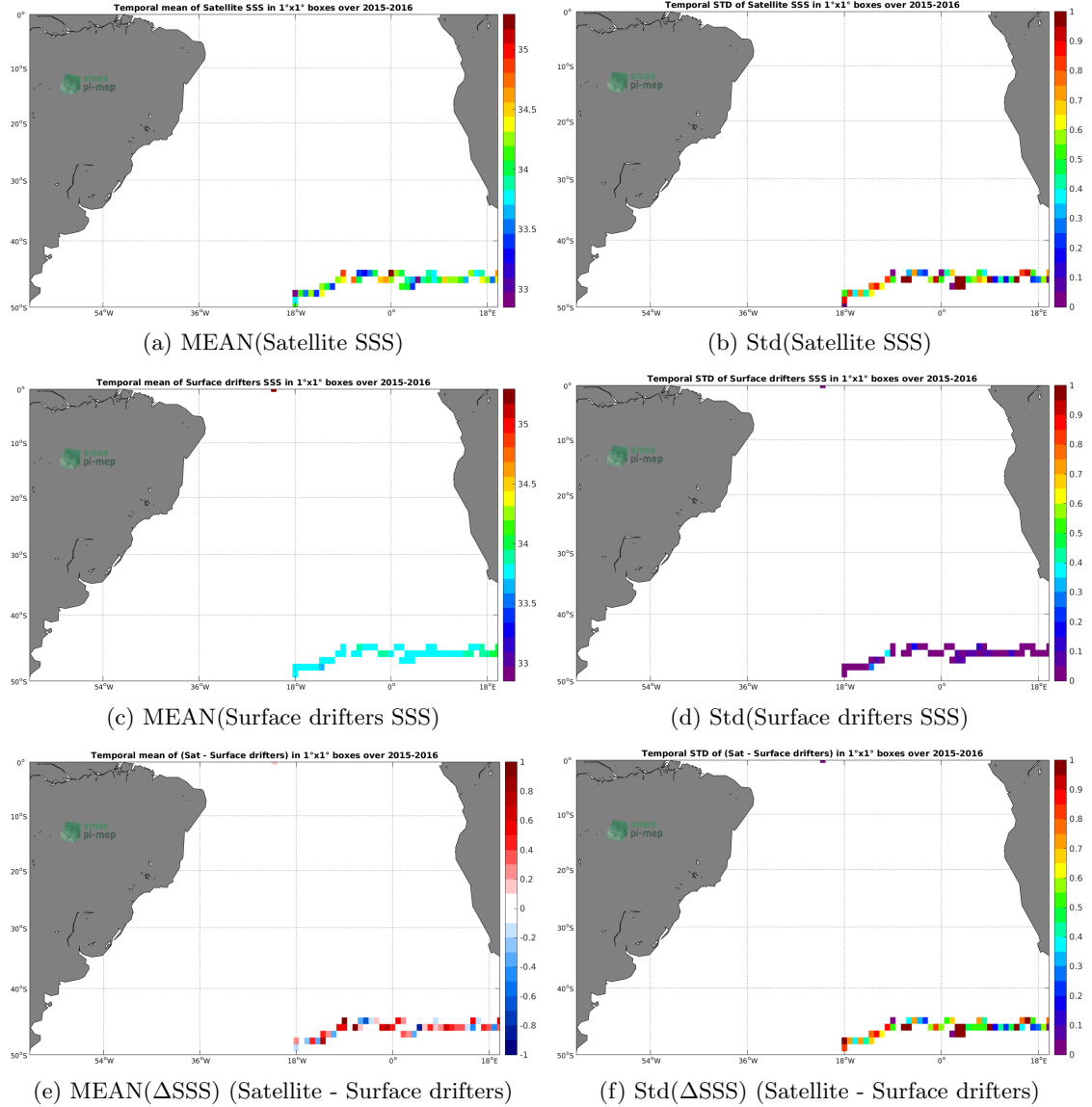
Figure 5: Temporal mean (left) and Std (right) of SSS from SMAP-L2-RSS-V4 (top), Surface drifters (middle), and of \Delta SSS (Satellite - Surface drifters). Only match-up pairs are used to generate these maps.
