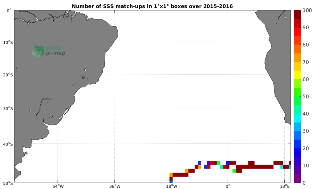
Figure 3: Number of SSS match-ups between Surface drifters SSS and the SMAP-L2-RSS-V4 SSS product for the South Atlantic Ocean Pi-MEP region over 1^\circ \times 1^\circ boxes and for the full satellite product period.
