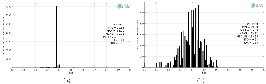
Figure 2: Histograms of SSS from Surface drifters (a) and SMAP-L2-RSS-V4 (b) considering all match-up pairs per bins of 0.1 over the South Atlantic Ocean Pi-MEP region and for the full satellite product period.
