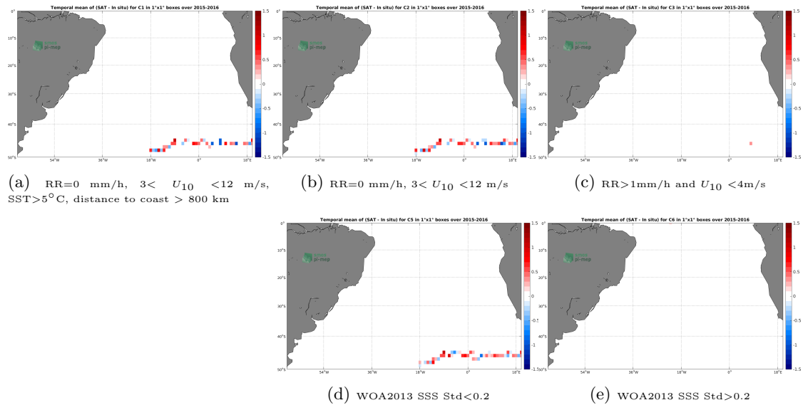
Figure 11: Temporal mean gridded over spatial boxes of size 1^{\circ}\times 1^{\circ} of \Delta\text{SSS} (SMAP-L2-RSS-V4 - Surface drifters) for 5 different subdatasets corresponding to:RR=0 mm/h, 3 < U_{10} < 12 m/s, SST >5^{\circ}\text{C} , distance to coast > 800 km (a), RR=0 mm/h, 3 < U_{10} < 12 m/s (b), RR >1 mm/h and U_{10} < 4 m/s (c), WOA2013 SSS Std <0.2 (d), WOA2013 SSS Std >0.2 (e).
