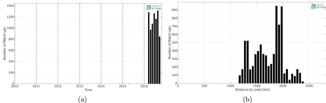
Figure 1: Number of match-ups between Surface drifters and SMAP-L2-RSS-V4 SSS as a function of time (a) and as function of the distance to coast (b) over the South Atlantic Ocean Pi-MEP region and for the full satellite product period.
